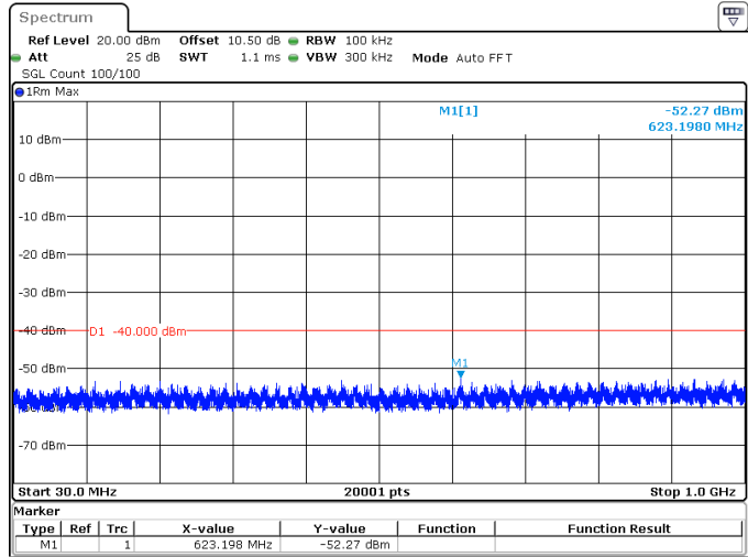
50MHz_30kHz_3625MHz_DFT-s-OFDM QPSK_RB1@132 -52.27 dBm
