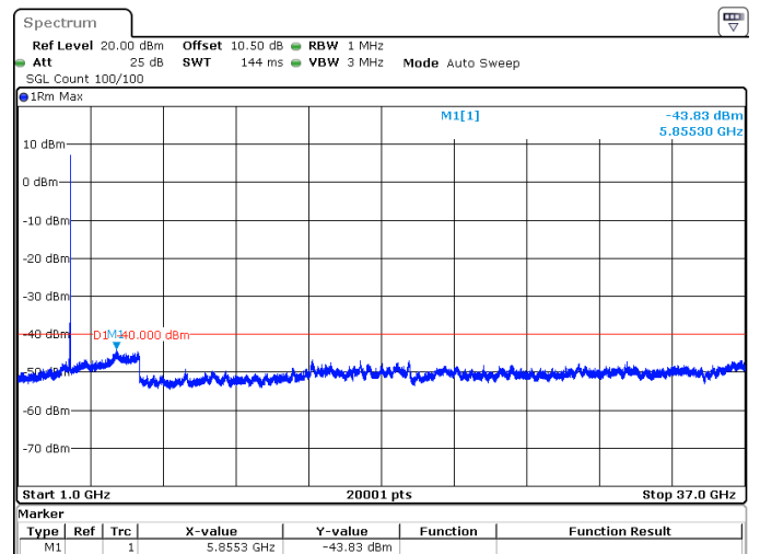
40MHz_30kHz_3570MHz_DFT-s-OFDM QPSK_RB1@105 -43.83 dBm
