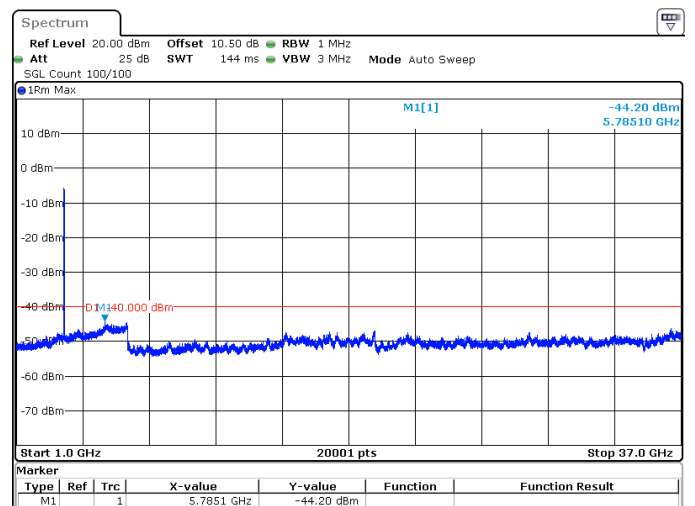
60MHz_30kHz_3580MHz_DFT-s-OFDM QPSK_RB162@0 -44.20 dBm
