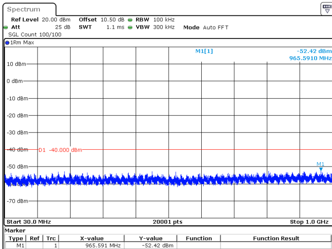
30MHz_15kHz_3685MHz_DFT-s-OFDM QPSK_RB1@159 -52.42 dBm
