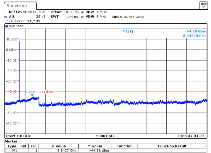
50MHz_15kHz_3625MHz_DFT-s-OFDM QPSK_RB1@0 -44.38 dBm
