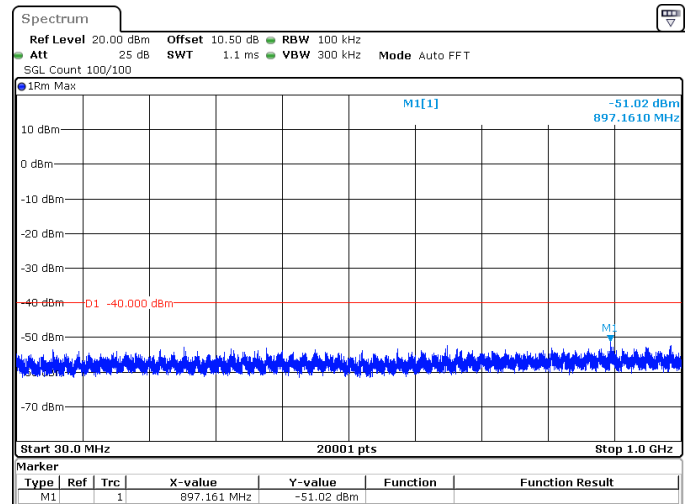
40MHz_15kHz_3680MHz_DFT-s-OFDM QPSK_RB216@0 -51.02 dBm
