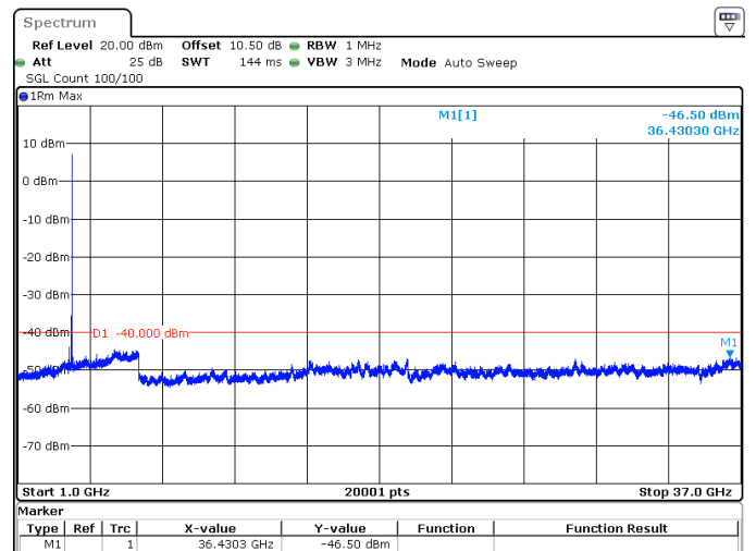
70MHz_30kHz_3665MHz_DFT-s-OFDM QPSK_RB1@188 -46.50 dBm
