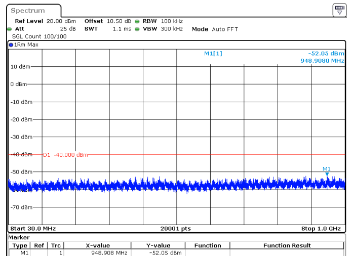
50MHz_30kHz_3675MHz_DFT-s-OFDM QPSK_RB1@132 -52.05 dBm
