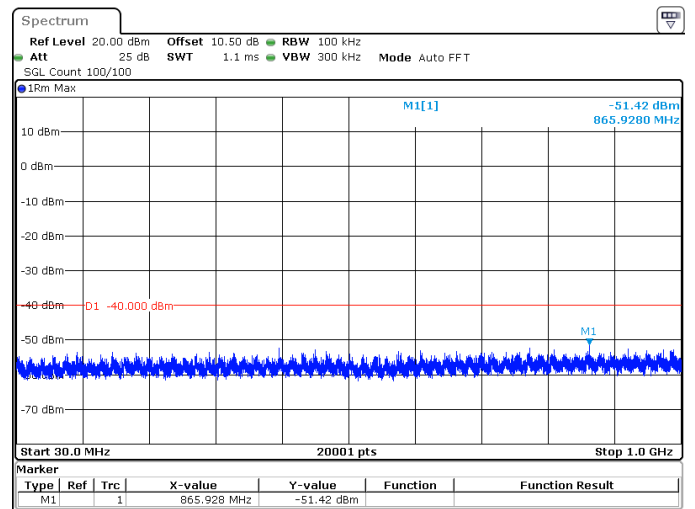
15MHz_30kHz_3625MHz_DFT-s-OFDM QPSK_RB1@37 -51.42 dBm
