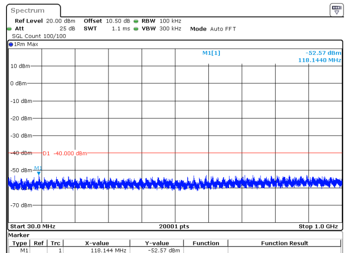
50MHz_30kHz_3575MHz_DFT-s-OFDM QPSK_RB128@0 -52.57 dBm
