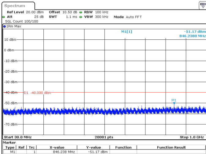
40MHz_15kHz_3680MHz_DFT-s-OFDM QPSK_RB1@215 -51.17 dBm
