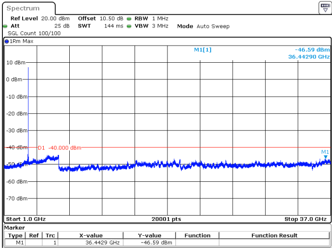
50MHz_30kHz_3625MHz_DFT-s-OFDM QPSK_RB1@132 -46.59 dBm
