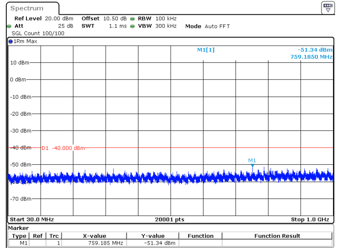
50MHz_30kHz_3575MHz_DFT-s-OFDM QPSK_RB1@0 -51.34 dBm
