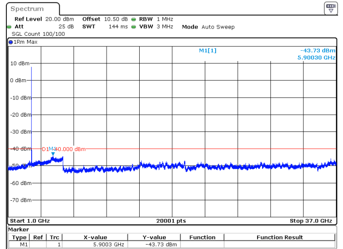
20MHz_15kHz_3560MHz_DFT-s-OFDM QPSK_RB1@105 -43.73 dBm
