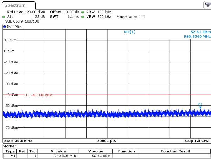
30MHz_15kHz_3625MHz_DFT-s-OFDM QPSK_RB160@0 -52.61 dBm
