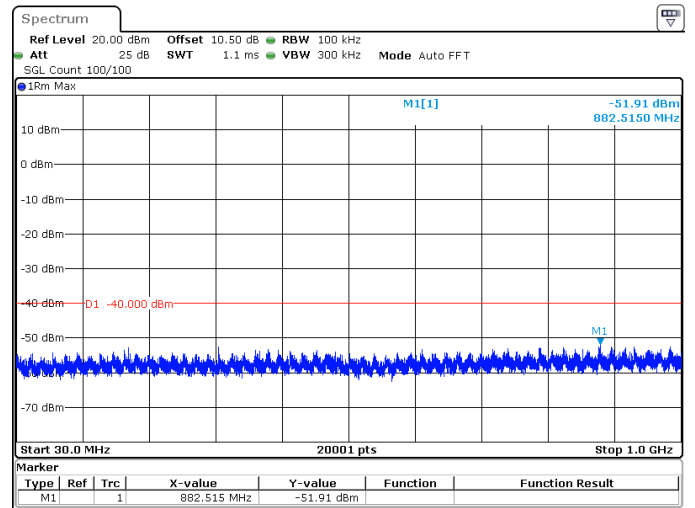
15MHz_30kHz_3625MHz_DFT-s-OFDM QPSK_RB1@0 -51.91 dBm
