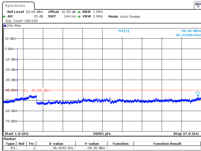
15MHz_30kHz_3557.5MHz_DFT-s-OFDM QPSK_RB36@0 -46.36 dBm
