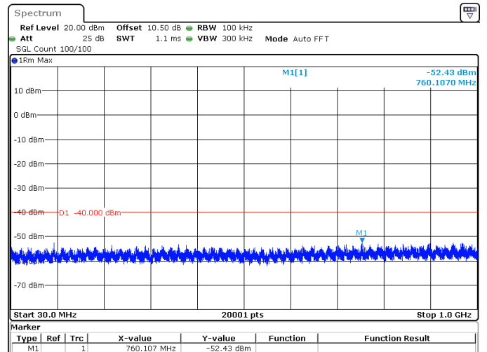
30MHz_15kHz_3565MHz_DFT-s-OFDM QPSK_RB160@0 -52.43 dBm
