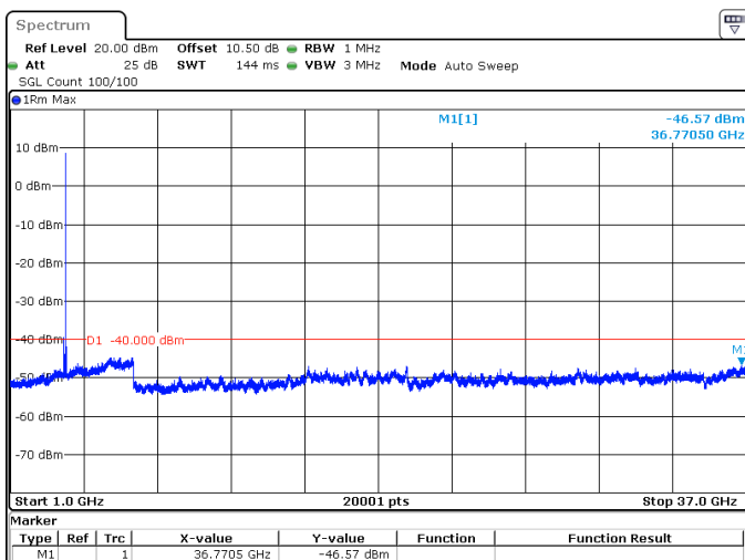
50MHz_15kHz_3675MHz_DFT-s-OFDM QPSK_RB1@269 -46.57 dBm
