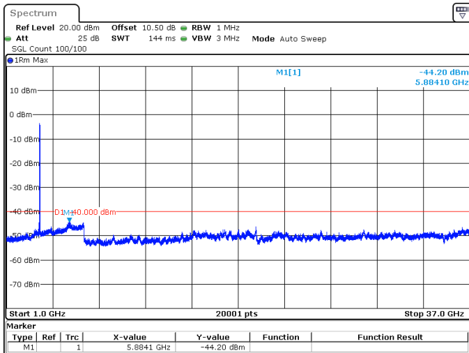
30MHz_15kHz_3565MHz_DFT-s-OFDM QPSK_RB160@0 -44.20 dBm
