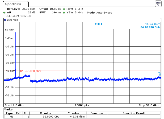
40MHz_15kHz_3680MHz_DFT-s-OFDM QPSK_RB1@0 -46.35 dBm
