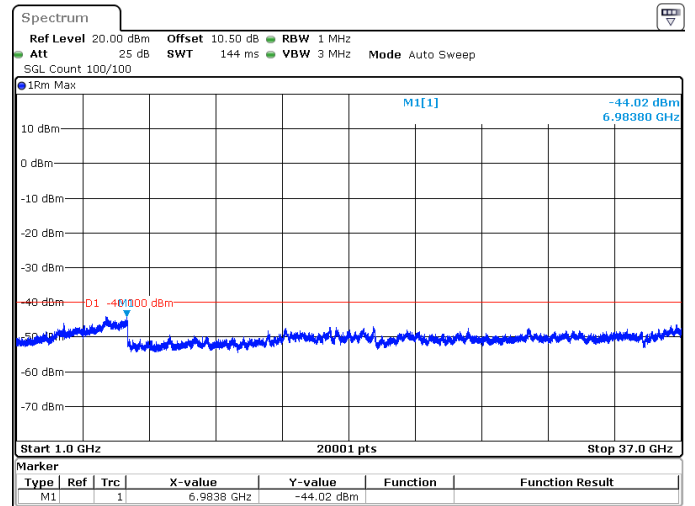
50MHz_30kHz_3575MHz_DFT-s-OFDM QPSK_RB1@132 -44.02 dBm
