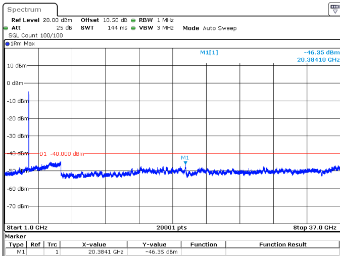
50MHz_15kHz_3575MHz_DFT-s-OFDM QPSK_RB270@0 -46.35 dBm
