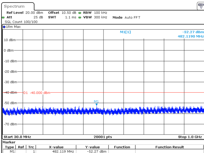
70MHz_30kHz_3585MHz_DFT-s-OFDM QPSK_RB1@188 -52.27 dBm
