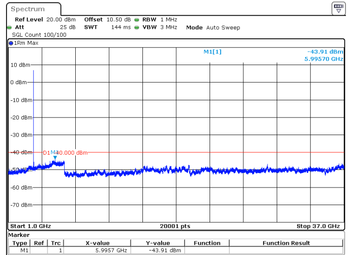
30MHz_15kHz_3685MHz_DFT-s-OFDM QPSK_RB1@159 -43.91 dBm
