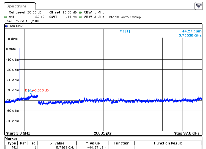
15MHz_30kHz_3692.5MHz_DFT-s-OFDM QPSK_RB36@0 -44.27 dBm
