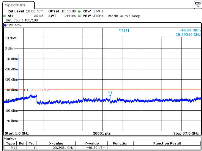
50MHz_30kHz_3625MHz_DFT-s-OFDM QPSK_RB128@0 -46.59 dBm
