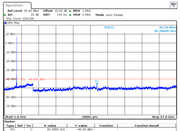
60MHz_30kHz_3580MHz_DFT-s-OFDM QPSK_RB1@161 -46.29 dBm
