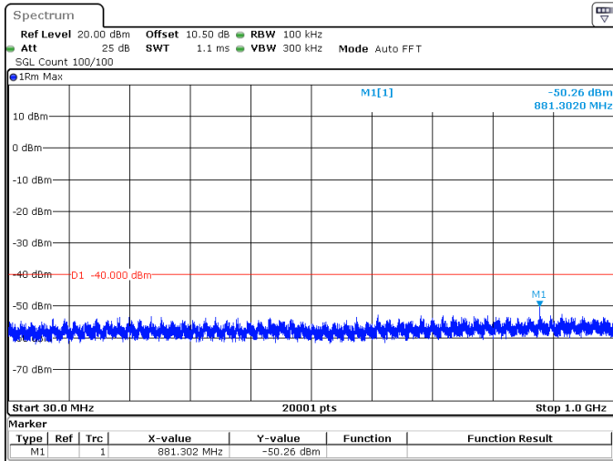
40MHz_15kHz_3570MHz_DFT-s-OFDM QPSK_RB216@0 -50.26 dBm
