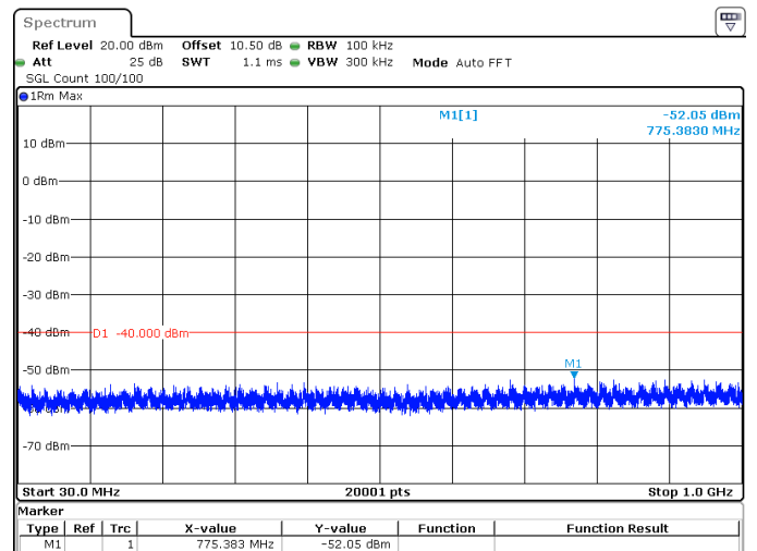
50MHz_15kHz_3675MHz_DFT-s-OFDM QPSK_RB1@269 -52.05 dBm
