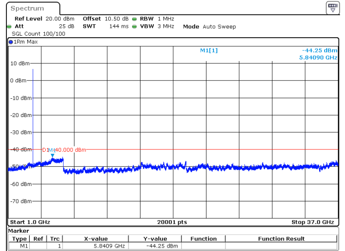
15MHz_30kHz_3692.5MHz_DFT-s-OFDM QPSK_RB1@0 -44.25 dBm
