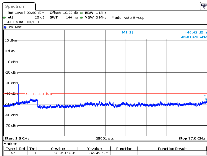
15MHz_30kHz_3625MHz_DFT-s-OFDM QPSK_RB1@0 -46.42 dBm
