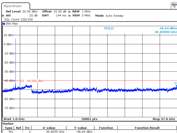
50MHz_30kHz_3675MHz_DFT-s-OFDM QPSK_RB1@132 -46.64 dBm
