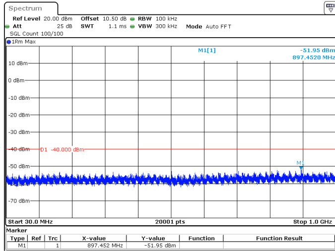
40MHz_30kHz_3680MHz_DFT-s-OFDM QPSK_RB100@0 -51.95 dBm
