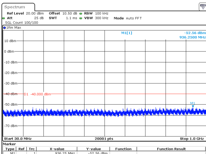
40MHz_30kHz_3570MHz_DFT-s-OFDM QPSK_RB1@105 -52.56 dBm
