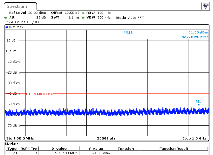
50MHz_15kHz_3625MHz_DFT-s-OFDM QPSK_RB1@269 -51.38 dBm
