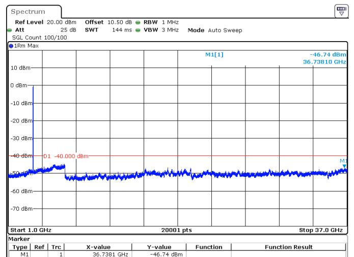
15MHz_30kHz_3625MHz_DFT-s-OFDM QPSK_RB36@0 -46.74 dBm
