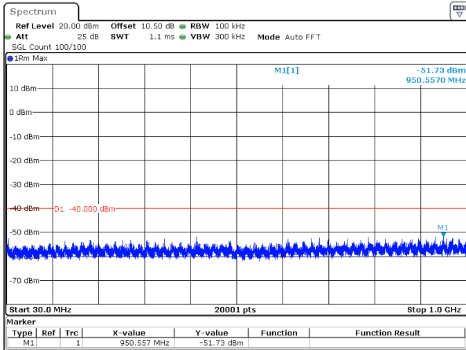
15MHz_30kHz_3625MHz_DFT-s-OFDM QPSK_RB36@0 -51.73 dBm
