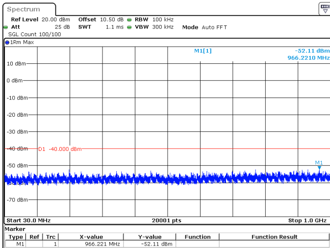
40MHz_30kHz_3570MHz_DFT-s-OFDM QPSK_RB100@0 -52.11 dBm
