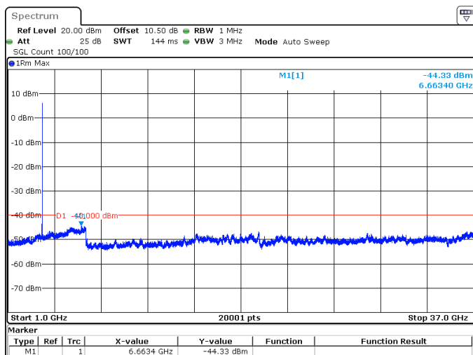
15MHz_30kHz_3625MHz_DFT-s-OFDM QPSK_RB1@37 -44.33 dBm
