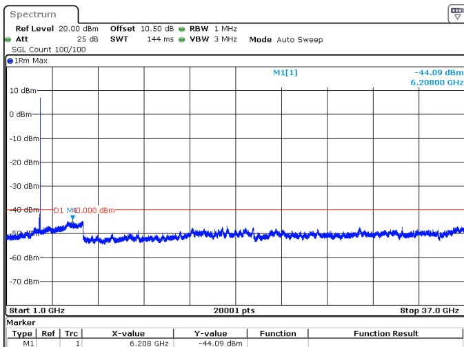
60MHz_30kHz_3625MHz_DFT-s-OFDM QPSK_RB1@161 -44.09 dBm
