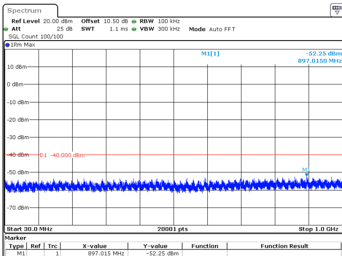
15MHz_30kHz_3692.5MHz_DFT-s-OFDM QPSK_RB1@37 -52.25 dBm
