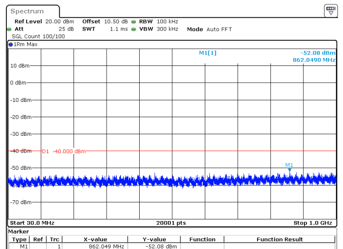
50MHz_30kHz_3675MHz_DFT-s-OFDM QPSK_RB128@0 -52.08 dBm
