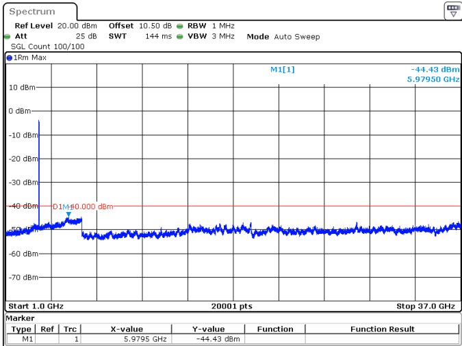
40MHz_30kHz_3625MHz_DFT-s-OFDM QPSK_RB100@0 -44.43 dBm
