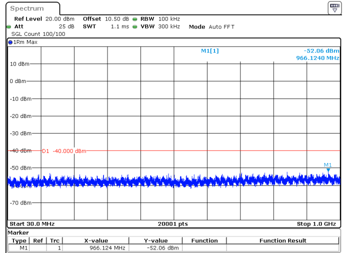
30MHz_15kHz_3565MHz_DFT-s-OFDM QPSK_RB1@0 -52.06 dBm
