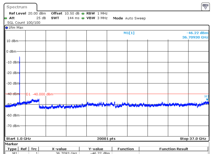
40MHz_30kHz_3570MHz_DFT-s-OFDM QPSK_RB100@0 -46.22 dBm
