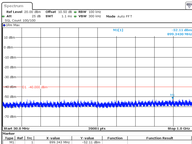
50MHz_15kHz_3625MHz_DFT-s-OFDM QPSK_RB1@0 -52.11 dBm
