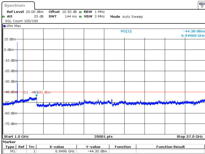
50MHz_30kHz_3575MHz_DFT-s-OFDM QPSK_RB1@0 -44.30 dBm
