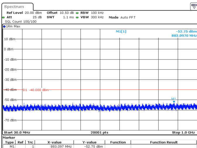
30MHz_15kHz_3625MHz_DFT-s-OFDM QPSK_RB1@159 -52.75 dBm
