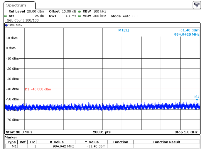
40MHz_15kHz_3625MHz_DFT-s-OFDM QPSK_RB1@215 -51.40 dBm
