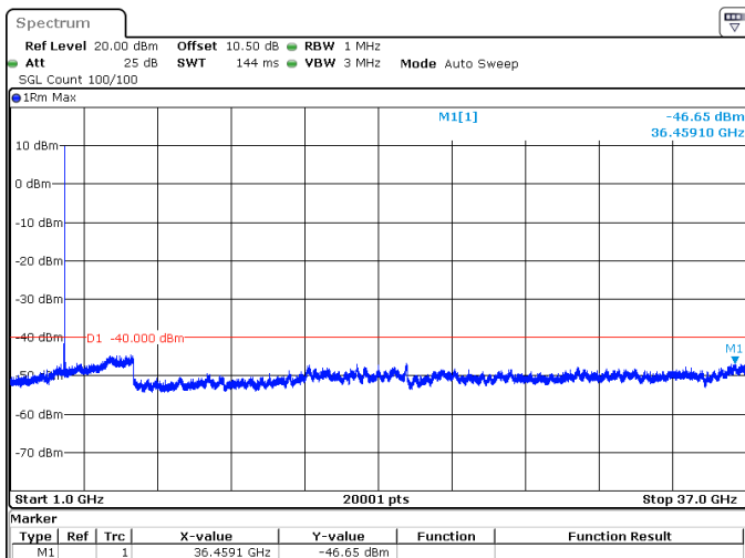
40MHz_15kHz_3625MHz_DFT-s-OFDM QPSK_RB1@215 -46.65 dBm
