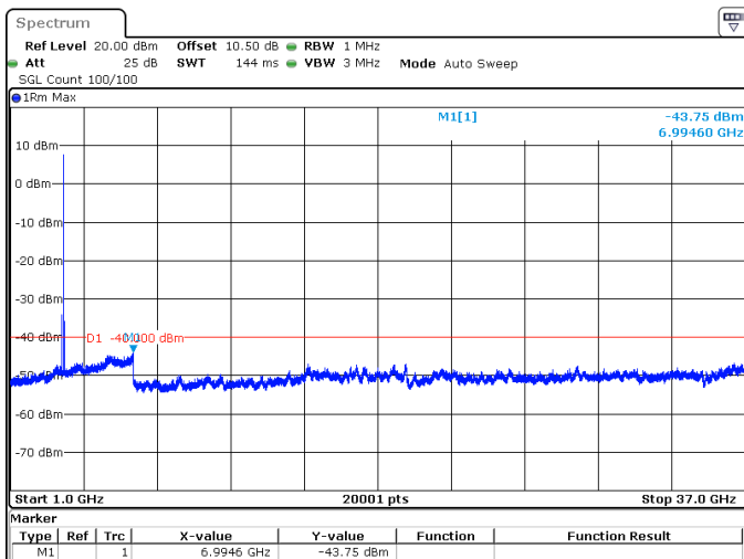
30MHz_15kHz_3625MHz_DFT-s-OFDM QPSK_RB1@0 -43.75 dBm
