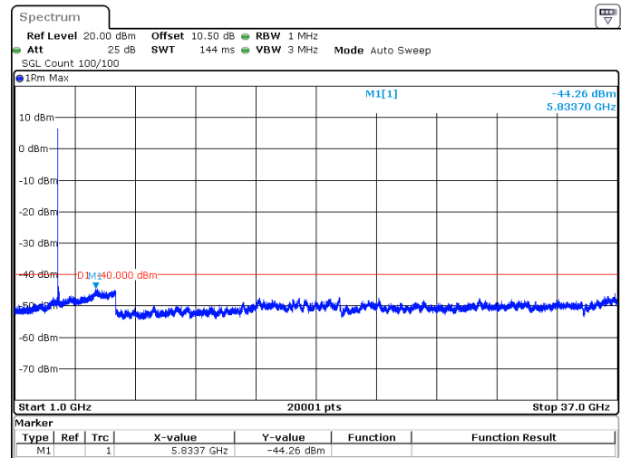
40MHz_30kHz_3570MHz_DFT-s-OFDM QPSK_RB1@0 -44.26 dBm
