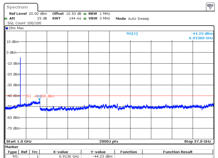
50MHz_15kHz_3625MHz_DFT-s-OFDM QPSK_RB270@0 -44.23 dBm
