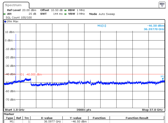
30MHz_15kHz_3625MHz_DFT-s-OFDM QPSK_RB1@159 -46.50 dBm
