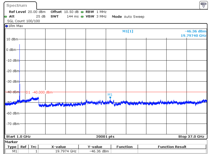
70MHz_30kHz_3585MHz_DFT-s-OFDM QPSK_RB1@188 -46.36 dBm
