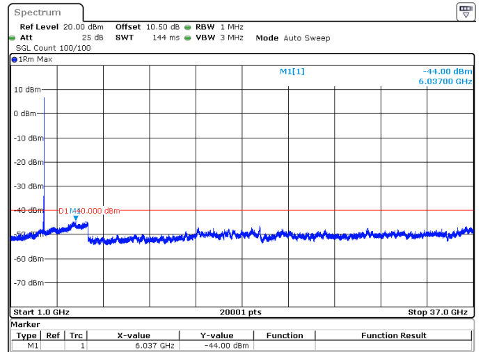
30MHz_15kHz_3565MHz_DFT-s-OFDM QPSK_RB1@159 -44.00 dBm
