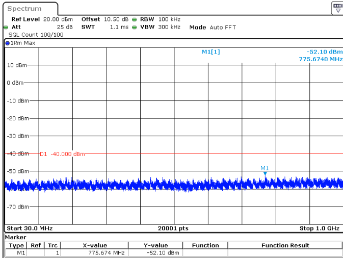
40MHz_15kHz_3625MHz_DFT-s-OFDM QPSK_RB216@0 -52.10 dBm
