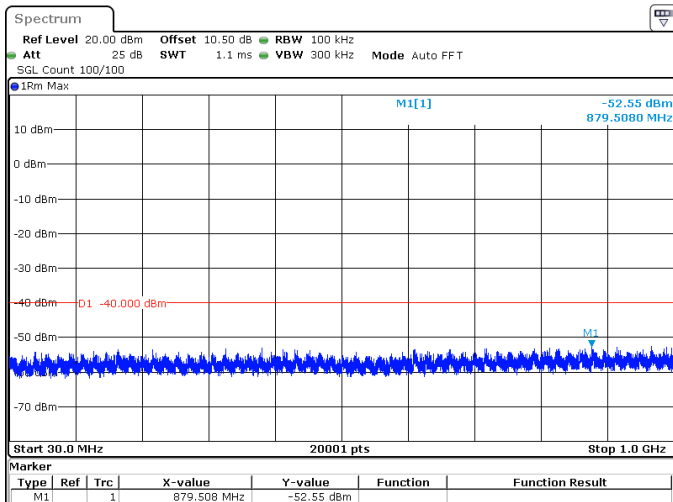
30MHz_15kHz_3565MHz_DFT-s-OFDM QPSK_RB1@159 -52.55 dBm
