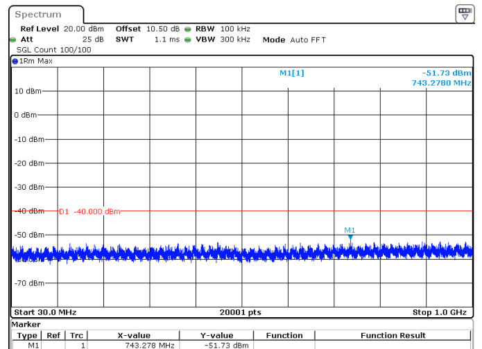
20MHz_15kHz_3560MHz_DFT-s-OFDM QPSK_RB100@0 -51.73 dBm
