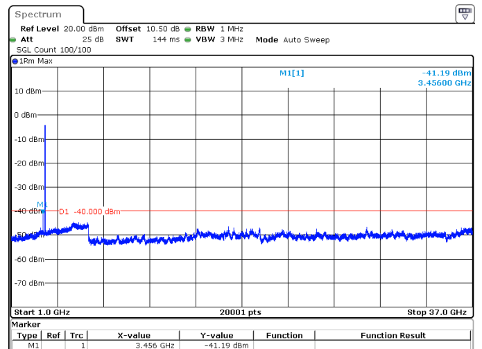
40MHz_15kHz_3625MHz_DFT-s-OFDM QPSK_RB216@0 -41.19 dBm
