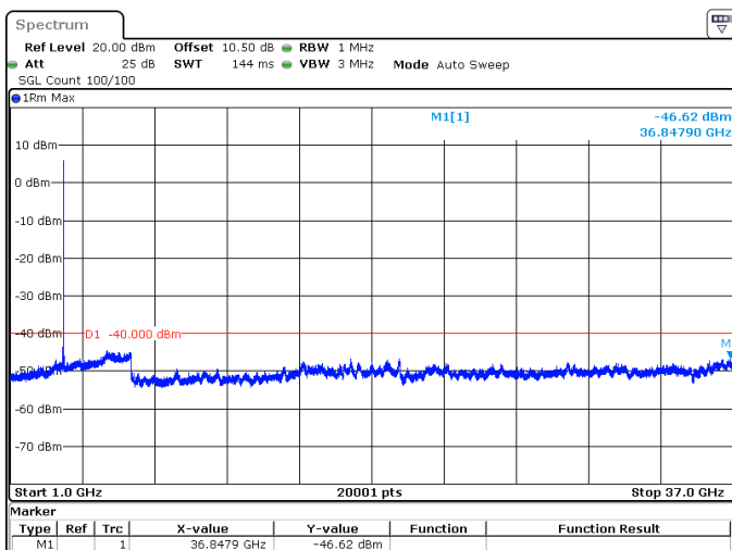
70MHz_30kHz_3625MHz_DFT-s-OFDM QPSK_RB1@188 -46.62 dBm
