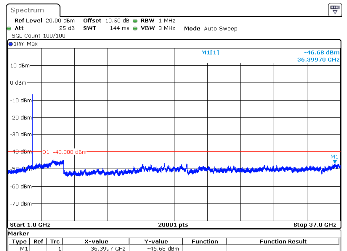
60MHz_30kHz_3625MHz_DFT-s-OFDM QPSK_RB162@0 -46.68 dBm
