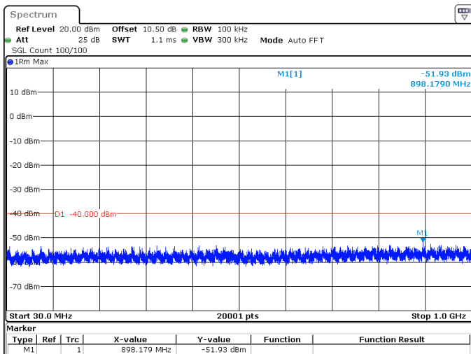
40MHz_30kHz_3570MHz_DFT-s-OFDM QPSK_RB1@0 -51.93 dBm
