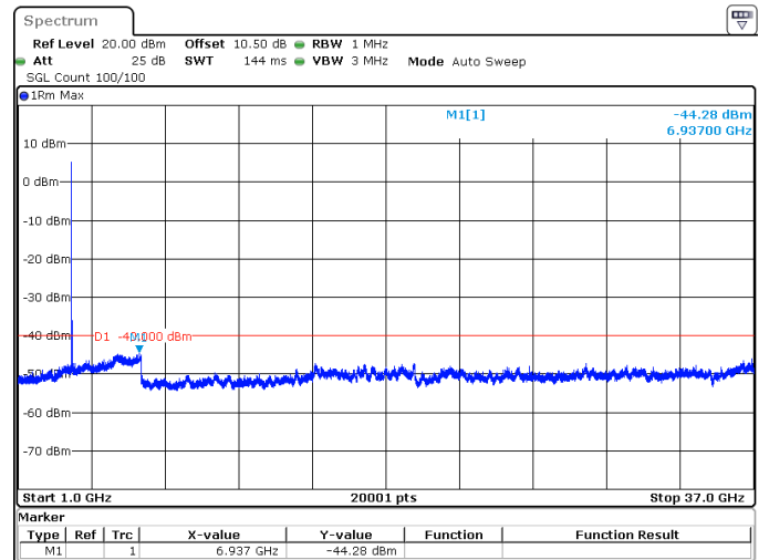
40MHz_30kHz_3625MHz_DFT-s-OFDM QPSK_RB1@0 -44.28 dBm
