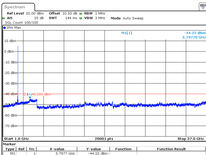
50MHz_15kHz_3625MHz_DFT-s-OFDM QPSK_RB1@269 -44.22 dBm
