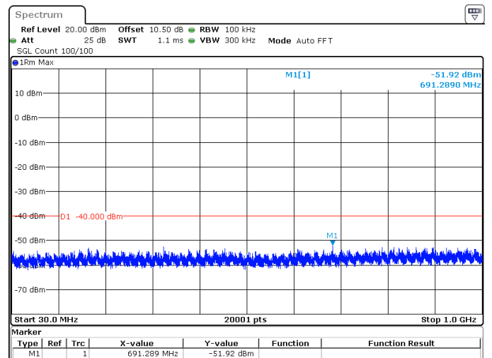
70MHz_30kHz_3625MHz_DFT-s-OFDM QPSK_RB1@188 -51.92 dBm
