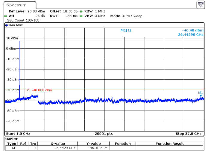
40MHz_15kHz_3625MHz_DFT-s-OFDM QPSK_RB1@0 -46.40 dBm
