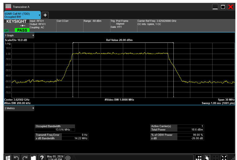
15MHz_30kHz_3625MHz_DFT-s-OFDM \pi/2 BPSK_RB36@0 13.516 MHz
