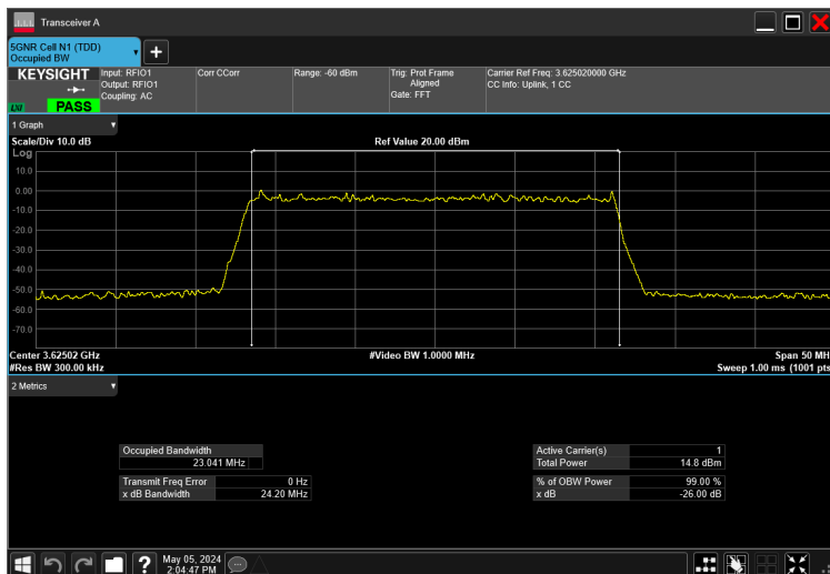
25MHz_30kHz_3625MHz_DFT-s-OFDM 256 QAM_RB64@0 23.041 MHz
