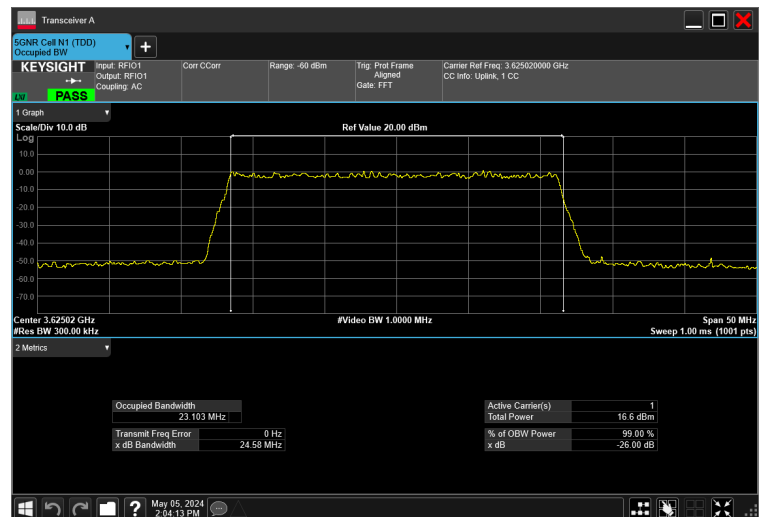
25MHz_30kHz_3625MHz_DFT-s-OFDM 64 QAM_RB64@0 23.103 MHz
