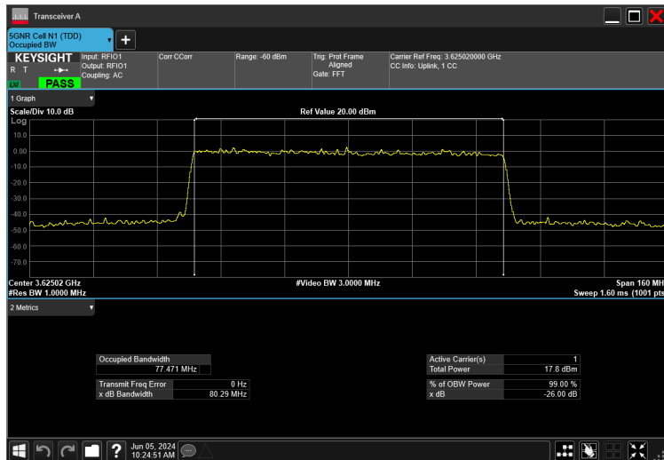
80MHz_30kHz_3625MHz_CP-OFDM QPSK_RB217@0 77.471 MHz
