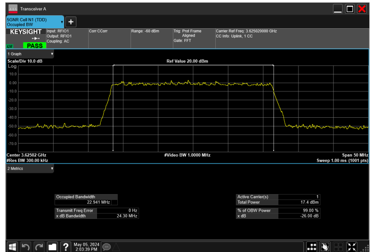
25MHz_30kHz_3625MHz_DFT-s-OFDM 16 QAM_RB64@0 22.941 MHz
