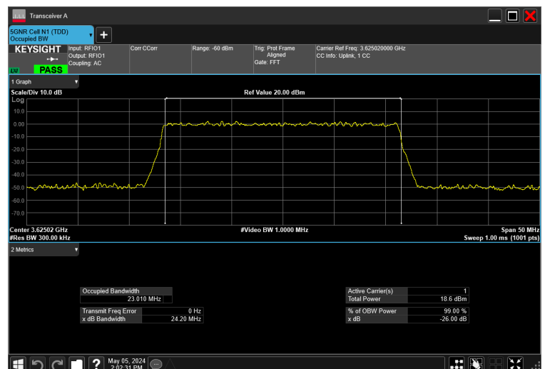
25MHz_30kHz_3625MHz_DFT-s-OFDM \pi/2 BPSK_RB64@0 23.010 MHz
