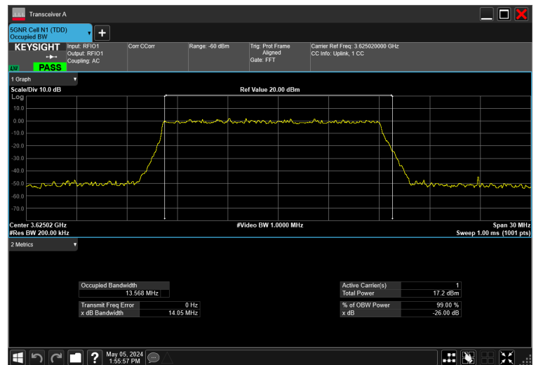
15MHz_30kHz_3625MHz_DFT-s-OFDM 16 QAM_RB36@0 13.568 MHz
