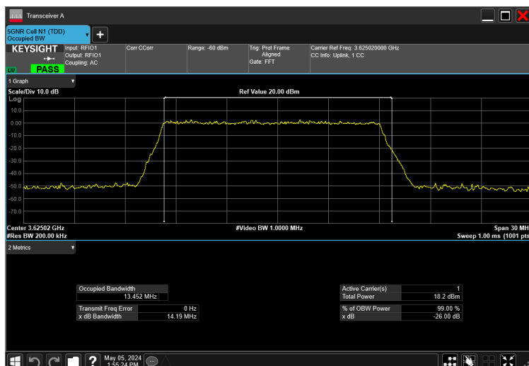
15MHz_30kHz_3625MHz_DFT-s-OFDM QPSK_RB36@0 13.452 MHz
