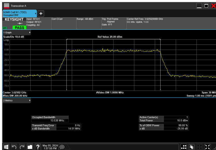
15MHz_30kHz_3625MHz_CP-OFDM QPSK_RB36@0 13.530 MHz
