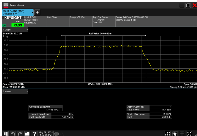
15MHz_30kHz_3625MHz_DFT-s-OFDM 256 QAM_RB36@0 13.455 MHz
