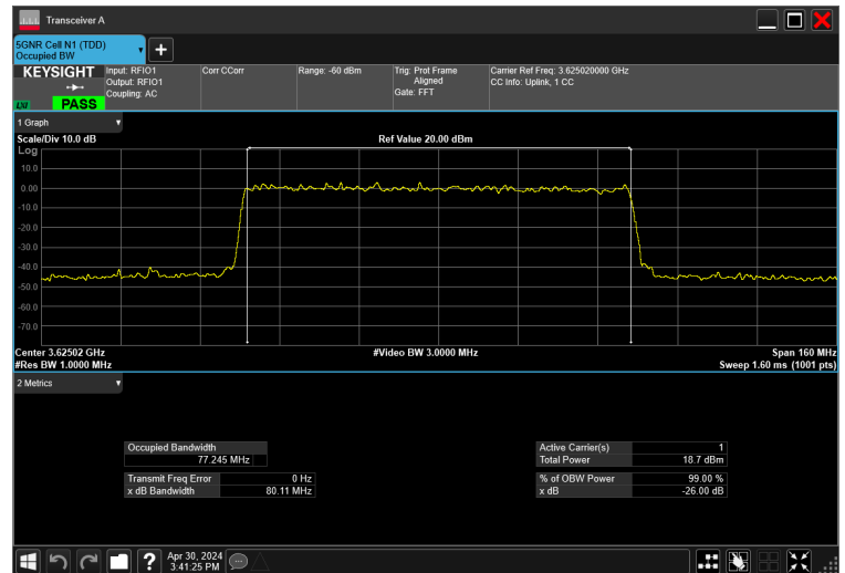
80MHz_30kHz_3625MHz_DFT-s-OFDM 16 QAM_RB216@0 77.245 MHz
