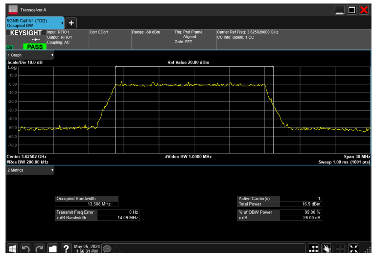
15MHz_30kHz_3625MHz_DFT-s-OFDM 64 QAM_RB36@0 13.508 MHz
