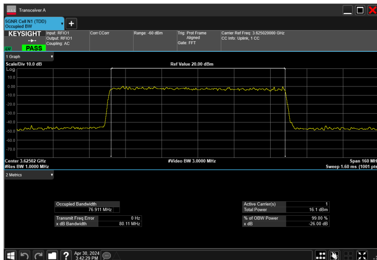
80MHz_30kHz_3625MHz_DFT-s-OFDM 256 QAM_RB216@0 76.911 MHz
