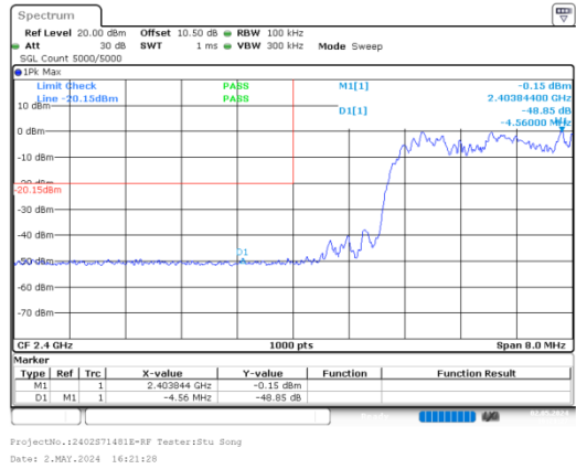
8DPSK_Hopping_Lower
