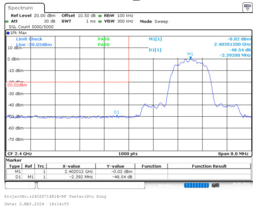
8DPSK_Low
