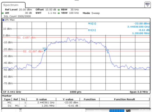
8DPSK_Middle
