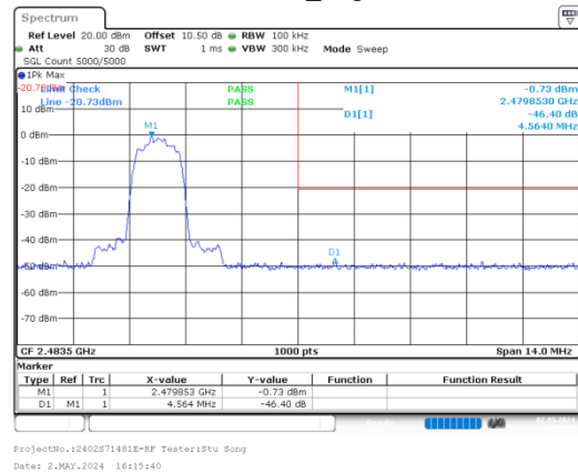
8DPSK_High
