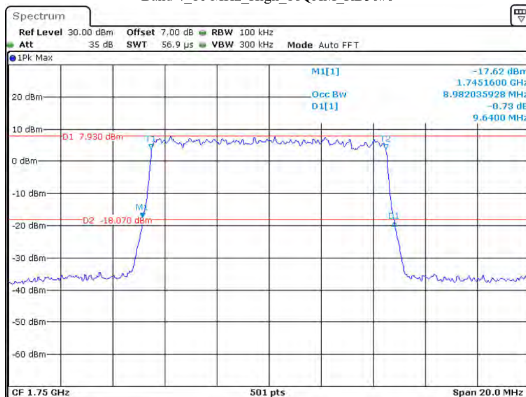
Band 4 10 MHz High 16QAM RB50#0
