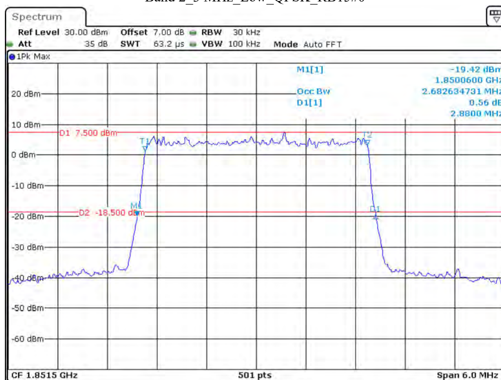
Band 2 3 MHz Low QPSK RB15#0
