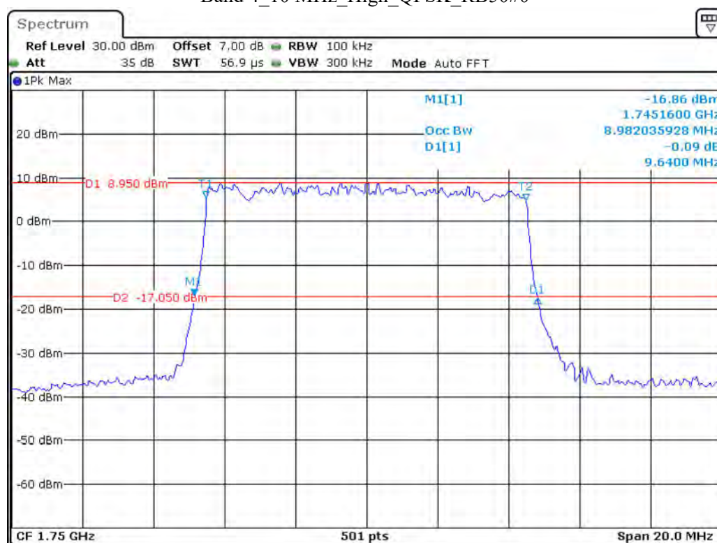
Band 4 10 MHz High QPSK RB50#0
