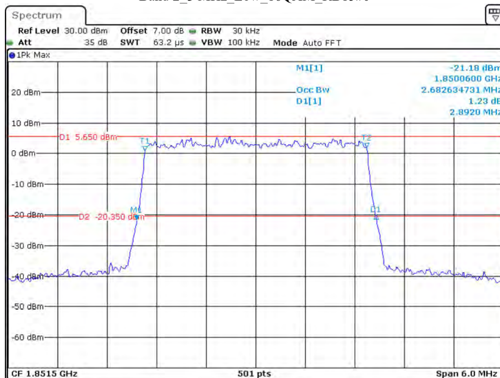
Band 2 3 MHz Low 16QAM RB15#0
