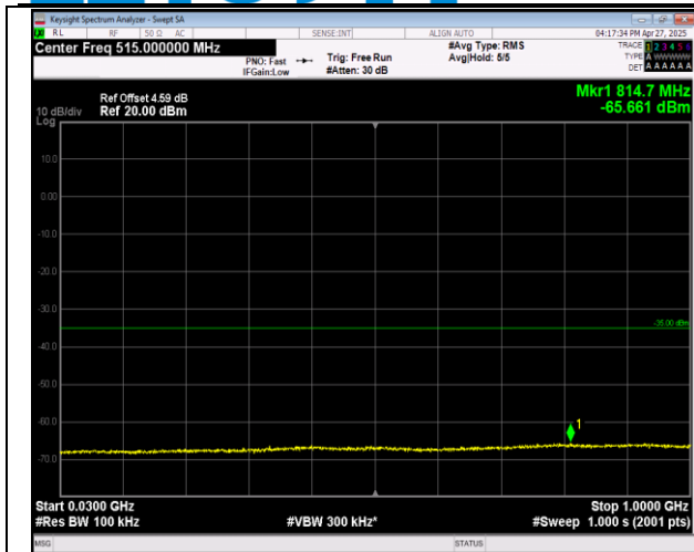
7-7-20MHz-20MHz-QPSK-QPSK-21152-21350-1RB#99-0 RB#0-30~1000MHz-PASS
