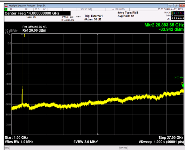
38-38-15MHz-15MHz-QPSK-QPSK-38025-38175-1RB#0-1 RB#74-1000~27000MHz-PASS
