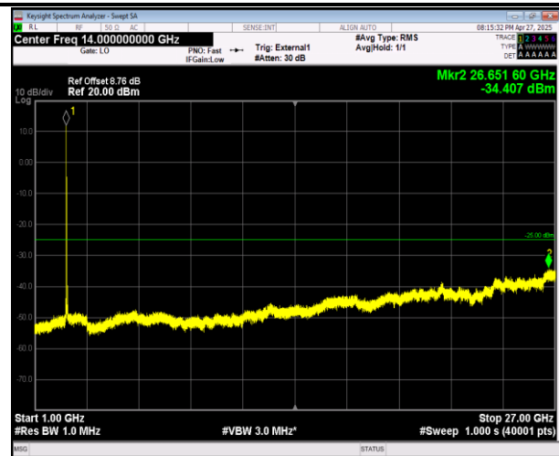
38-38-20MHz-20MHz-16QAM-16QAM-37850-38048-1RB# 99-ORB#0-1000~27000MHz-PASS
