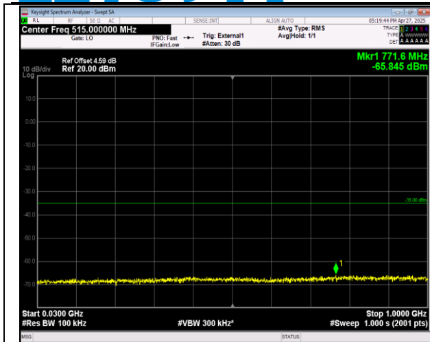
38-38-15MHz-15MHz-QPSK-QPSK-37825-37975-75RB# 0-75RB#0-30~1000MHz-PASS
