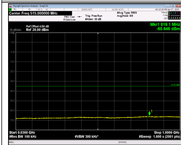
7-7-20MHz-20MHz-16QAM-16QAM-21001-21199-1RB#0 -1RB#99-30~1000MHz-PASS
