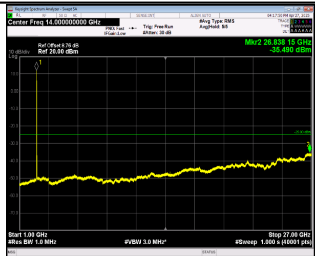
7-7-20MHz-20MHz-QPSK-QPSK-21152-21350-1RB#99-0R B#0-1000~27000MHz-PASS
