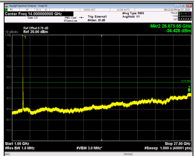
38-38-20MHz-20MHz-16QAM-16QAM-37850-38048-1RB# 0-1RB#99-1000~27000MHz-PASS
