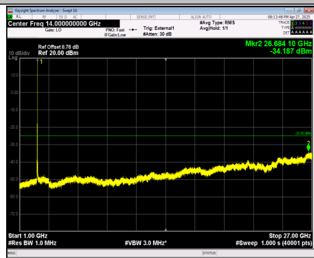
38-38-20MHz-20MHz-16QAM-16QAM-37850-38048-100R B#0-100RB#0-1000~27000MHz-PASS
