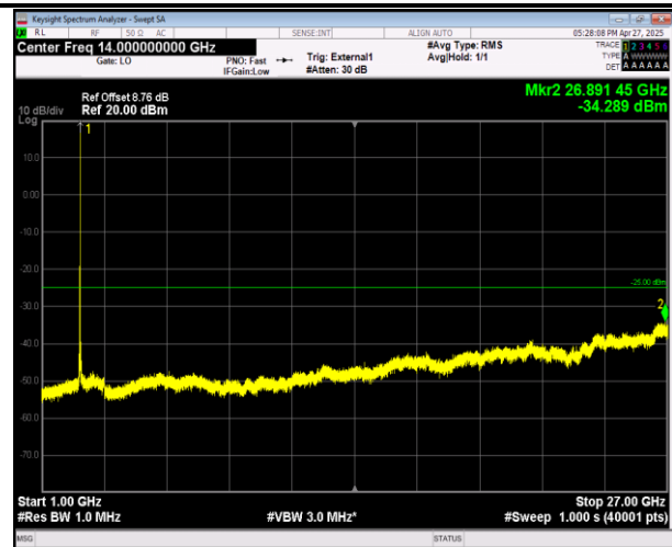
38-38-15MHz-15MHz-16QAM-16QAM-37925-38075-75RB #0-75RB#0-1000~27000MHz-PASS
