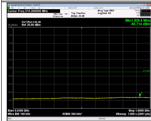
7-7-20MHz-20MHz-QPSK-QPSK-21152-21350-100RB#0- 100RB#0-30~1000MHz-PASS
