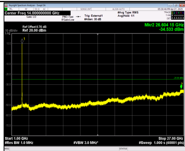
38-38-15MHz-15MHz-16QAM-16QAM-37925-38075-1RB# 0-ORB#0-1000~27000MHz-PASS
