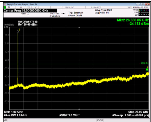
38-38-15MHz-15MHz-16QAM-16QAM-37825-37975-1RB# 74-ORB#0-1000~27000MHz-PASS
