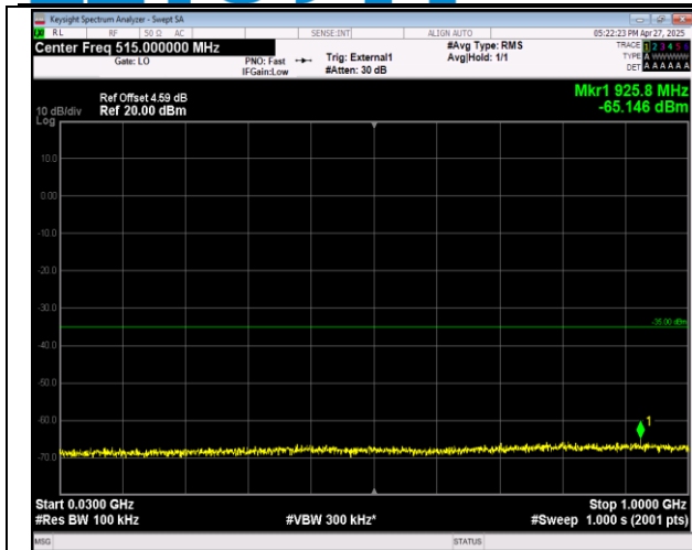
38-38-15MHz-15MHz-16QAM-16QAM-37825-37975-1RB #74-ORB#0-30~1000MHz-PASS
