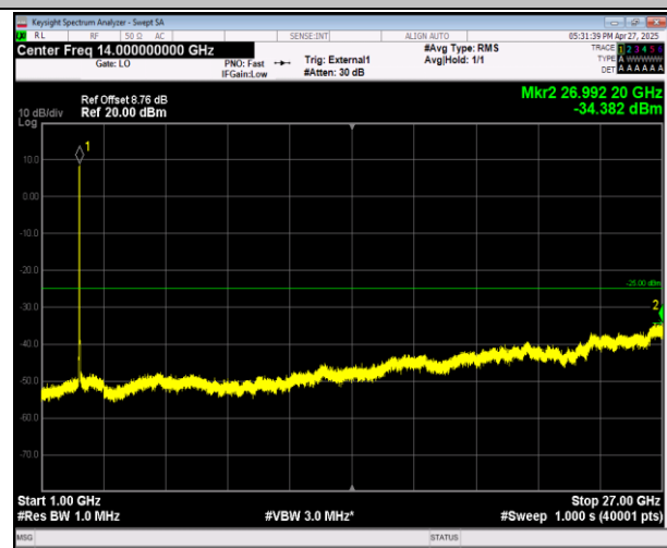
38-38-15MHz-15MHz-QPSK-QPSK-38025-38175-1RB#0-0 RB#0-1000~27000MHz-PASS
