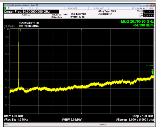
38-38-15MHz-15MHz-16QAM-16QAM-37825-37975-75RB #0-75RB#0-1000~27000MHz-PASS
