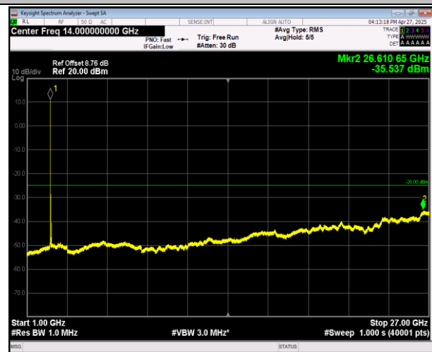
7-7-20MHz-20MHz-16QAM-16QAM-21001-21199-1RB#99- 0RB#0-1000~27000MHz-PASS
