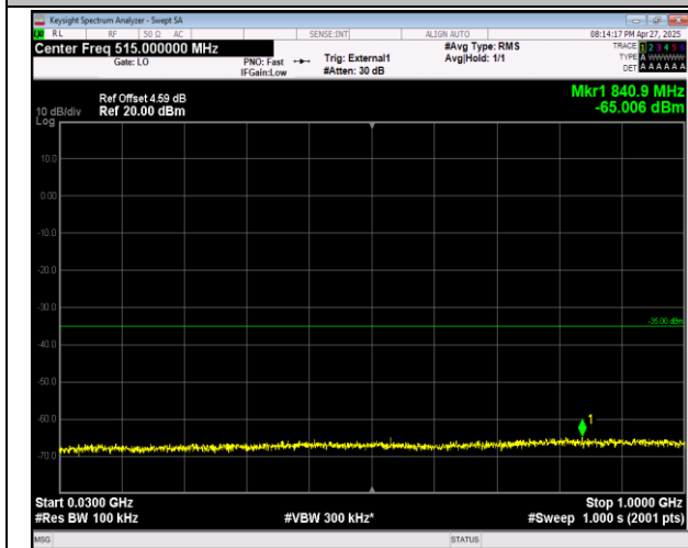
38-38-20MHz-20MHz-QPSK-QPSK-37850-38048-1RB#99-9-ORB#0-30~1000MHz-PASS
