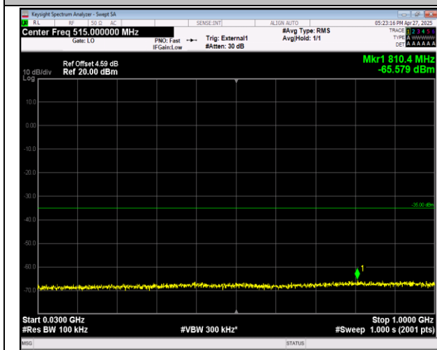
38-38-15MHz-15MHz-16QAM-16QAM-37825-37975-1RB #0-0RB#0-30~1000MHz-PASS
