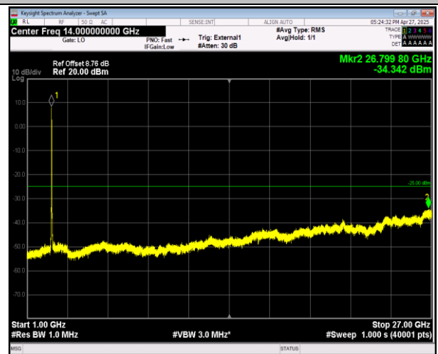
38-38-15MHz-15MHz-QPSK-QPSK-37925-38075-1RB#0-0 RB#0-1000~27000MHz-PASS
