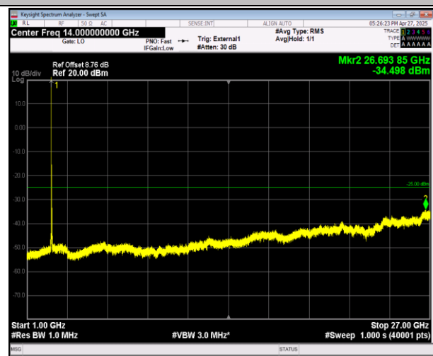
38-38-15MHz-15MHz-16QAM-16QAM-37925-38075-1RB# 0-1RB#74-1000~27000MHz-PASS
