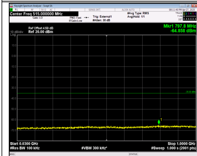
38-38-20MHz-20MHz-16QAM-16QAM-37850-38048-1RB #0-1RB#99-30~1000MHz-PASS
