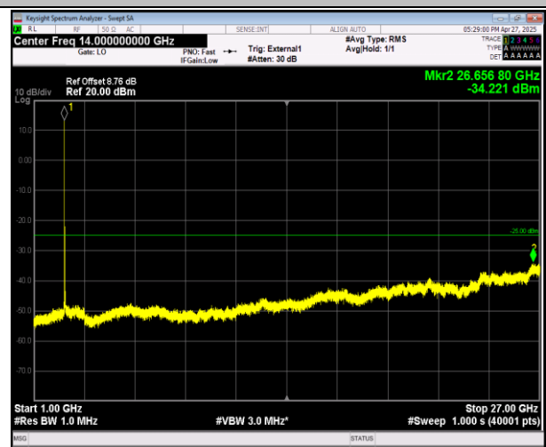
38-38-15MHz-15MHz-QPSK-QPSK-37925-38075-1RB#74-0RB#0-1000~27000MHz-PASS
