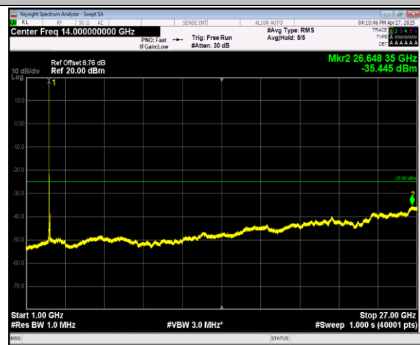
7-7-20MHz-20MHz-16QAM-16QAM-21001-21199-1RB#0-1 RB#99-1000~27000MHz-PASS
