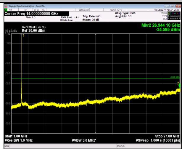
38-38-15MHz-15MHz-QPSK-QPSK-37825-37975-1RB#0-1 RB#74-1000~27000MHz-PASS
