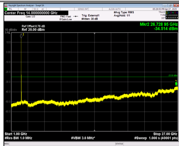
38-38-15MHz-15MHz-16QAM-16QAM-37925-38075-1RB# 74-ORB#0-1000~27000MHz-PASS
