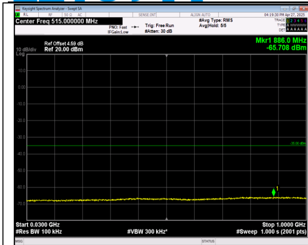
38-38-15MHz-15MHz-QPSK-QPSK-37825-37975-1RB#0- ORB#0-30~1000MHz-PASS
