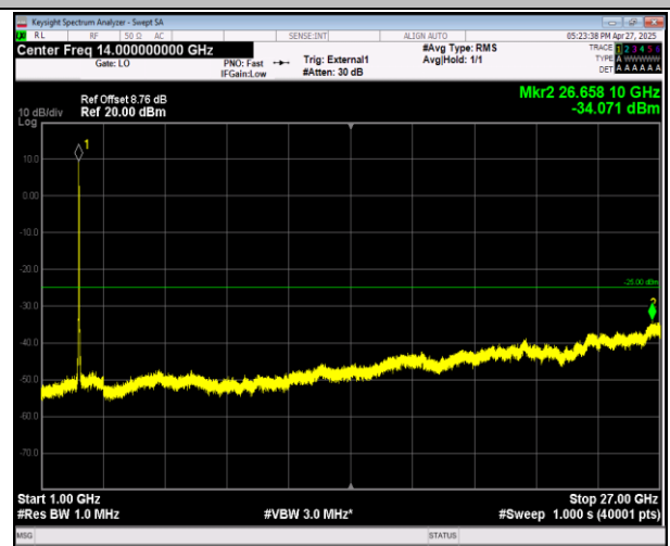
38-38-15MHz-15MHz-16QAM-16QAM-37825-37975-1RB# 0-0RB#0-1000~27000MHz-PASS
