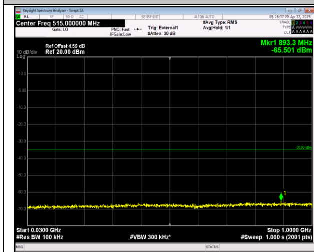
38-38-15MHz-15MHz-QPSK-QPSK-37925-38075-1RB#7-4-0RB#0-30~1000MHz-PASS
