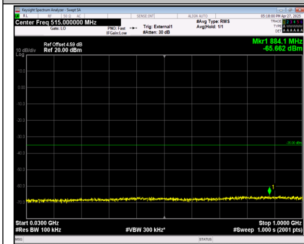
38-38-15MHz-15MHz-QPSK-QPSK-37825-37975-1RB#0- 1RB#74-30~1000MHz-PASS
