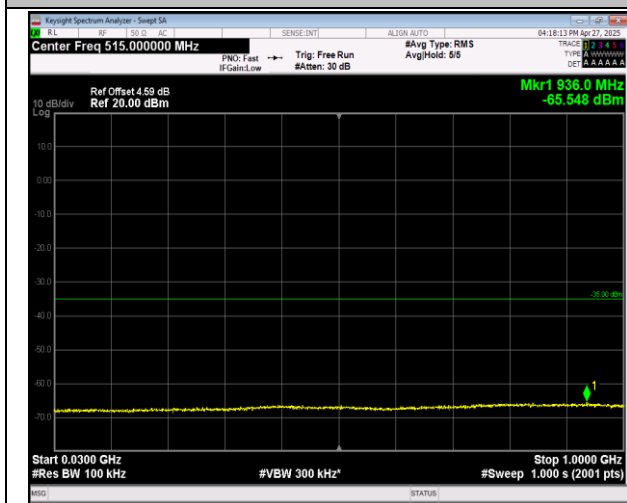
7-7-20MHz-20MHz-16QAM-16QAM-21152-21350-1RB#9 9-0RB#0-30~1000MHz-PASS
