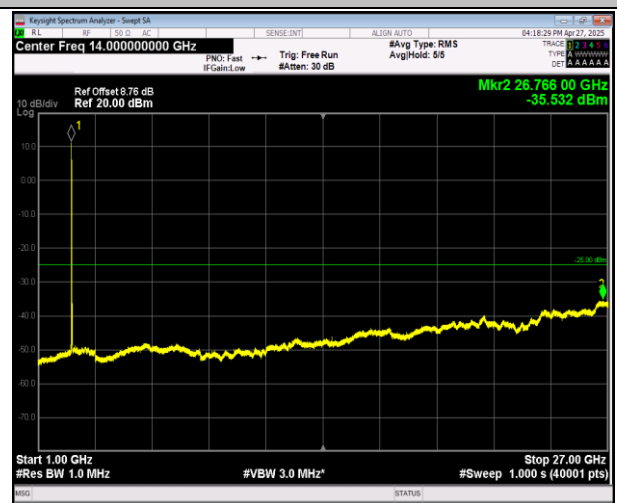
7-7-20MHz-20MHz-16QAM-16QAM-21152-21350-1RB#99- 0RB#0-1000~27000MHz-PASS
