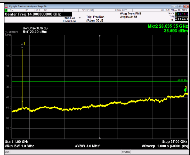
7-7-20MHz-20MHz-QPSK-QPSK-21152-21350-1RB#0-0RB #0-1000~27000MHz-PASS
