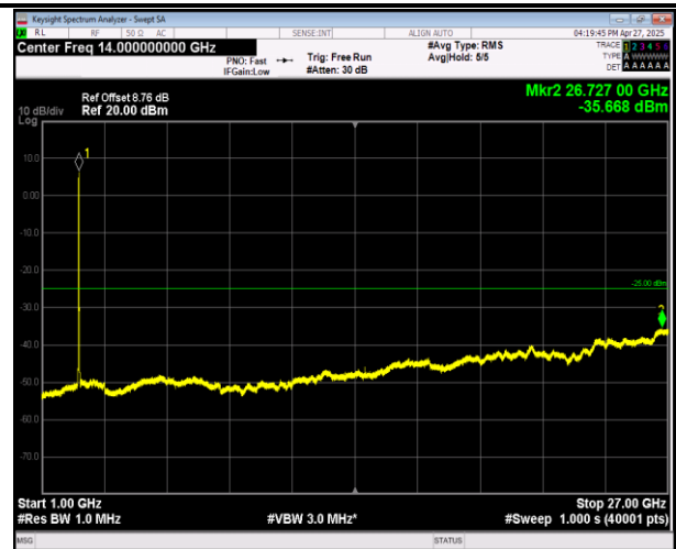
38-38-15MHz-15MHz-QPSK-QPSK-37825-37975-1RB#0-0 RB#0-1000~27000MHz-PASS
