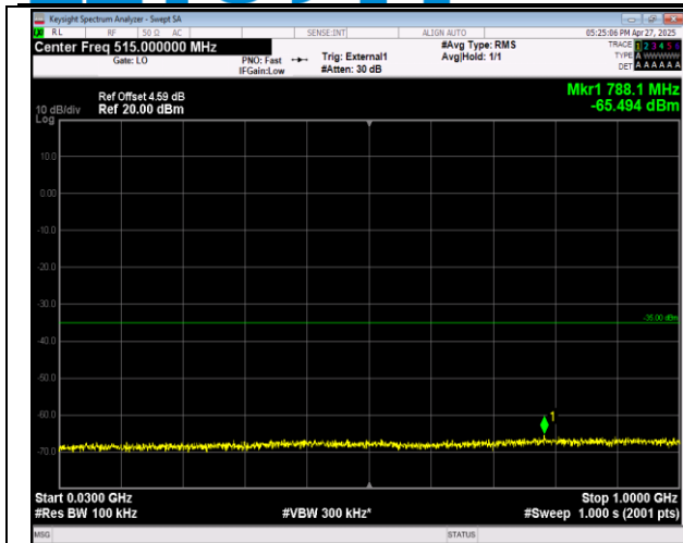
38-38-15MHz-15MHz-QPSK-QPSK-37925-38075-1RB#0-1RB#74-30~1000MHz-PASS
