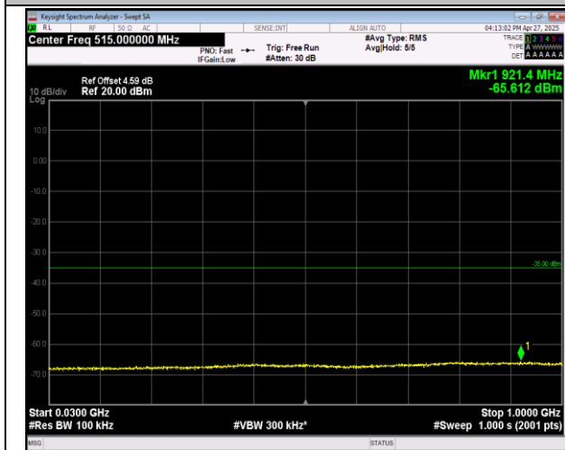
7-7-20MHz-20MHz-16QAM-16QAM-21001-21199-1RB#9 9-0RB#0-30~1000MHz-PASS
