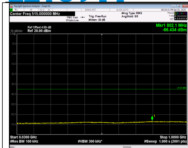
7-7-20MHz-10MHz-QPSK-QPSK-20850-20994-1RB#0-0 RB#0-30~1000MHz-PASS
