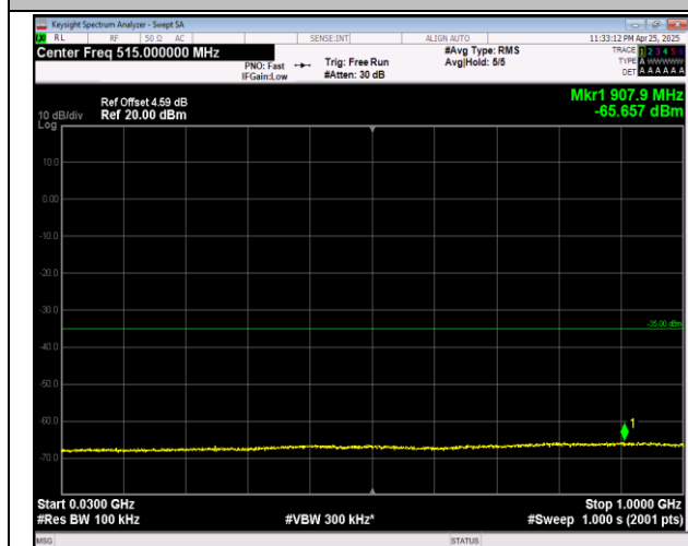
7-7-20MHz-10MHz-QPSK-QPSK-20850-20994-1RB#0-1 RB#49-30~1000MHz-PASS
