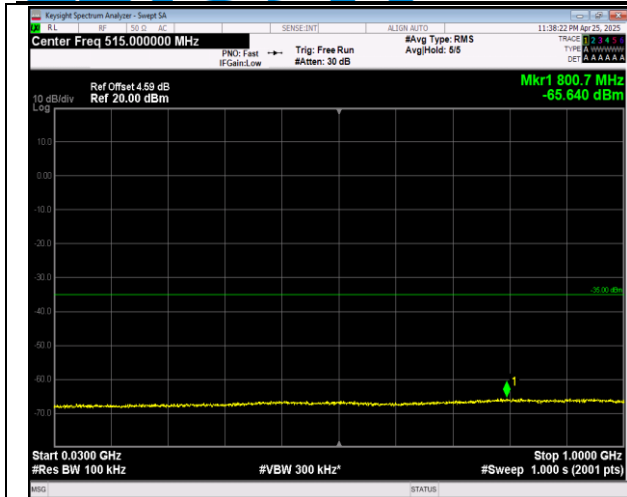
7-7-20MHz-10MHz-QPSK-QPSK-21051-21195-1RB#0-1 RB#49-30~1000MHz-PASS
