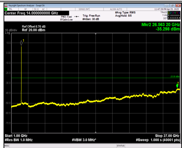
7-7-20MHz-10MHz-16QAM-16QAM-21251-21395-1RB#0-0RB#0-30~1000MHz-PASS RB#0-1000~27000MHz-PASS
