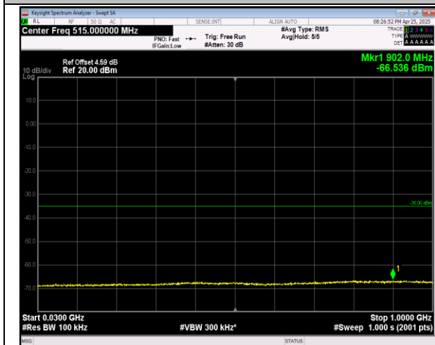
7-7-10MHz-20MHz-16QAM-16QAM-21206-21350-50RB# 0-100RB#0-30~1000MHz-PASS
