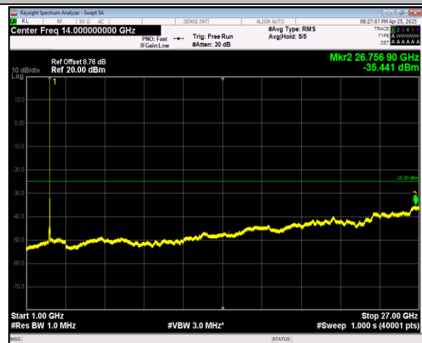
7-7-10MHz-20MHz-16QAM-16QAM-21206-21350-50RB#0- 100RB#0-1000~27000MHz-PASS
