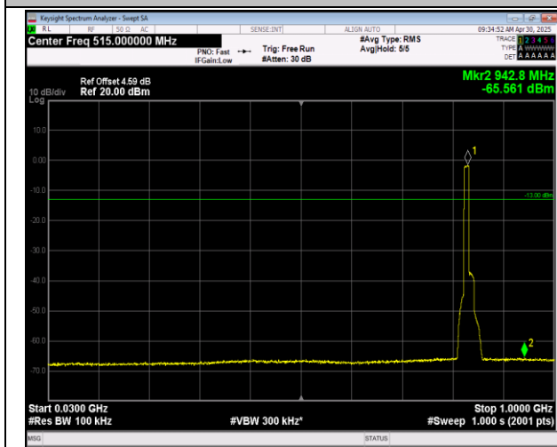
5-5-10MHz-10MHz-QPSK-QPSK-20501-20600-1RB#0-0 RB#0-30~1000MHz-PASS
