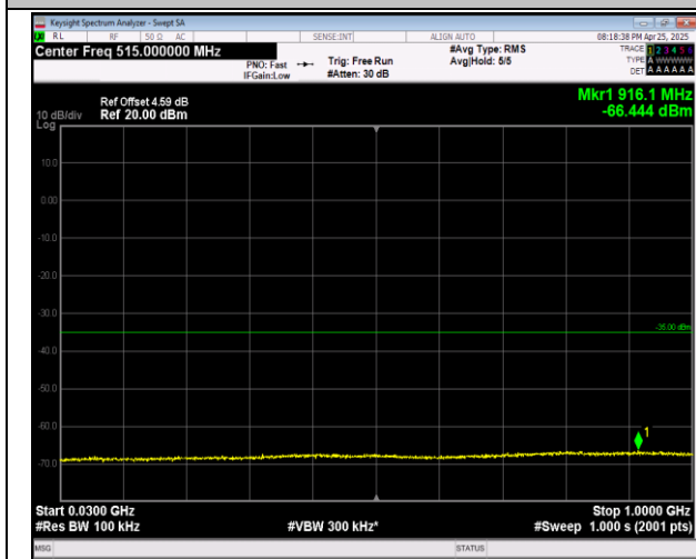
7-7-10MHz-20MHz-16QAM-16QAM-20805-20949-1RB#0 -0RB#0-30~1000MHz-PASS
