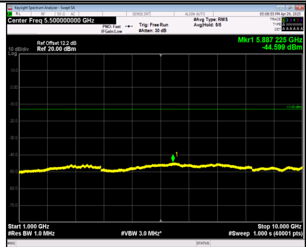
5-5-5MHz-3MHz-QPSK-QPSK-20510-20549-1RB#0-1RB#1 5-1000~10000MHz-PASS
