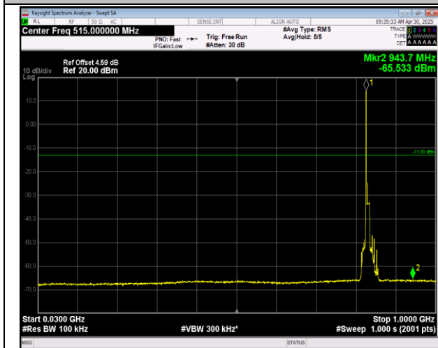
5-5-10MHz-10MHz-QPSK-QPSK-20501-20600-1RB#0-0-1 RB#49-30~1000MHz-PASS
