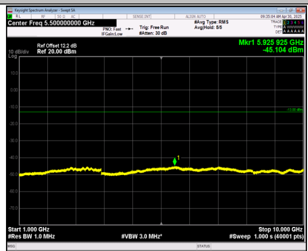
5-5-10MHz-10MHz-QPSK-QPSK-20501-20600-1RB#0-0RB #0-1000~10000MHz-PASS
