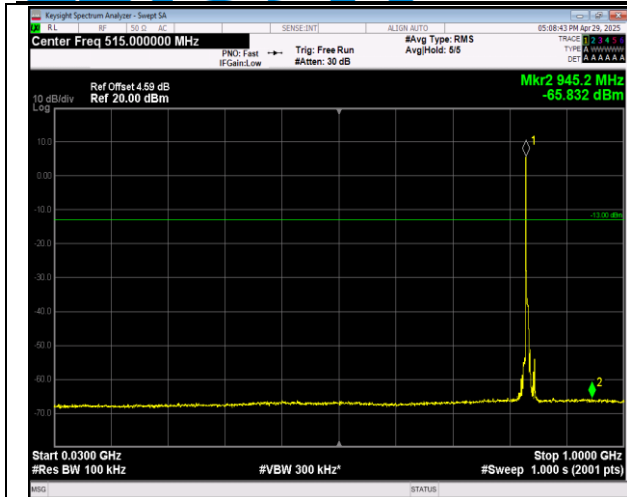
5-5-5MHz-3MHz-QPSK-QPSK-20510-20549-1RB#0-1RB #15-30~1000MHz-PASS
