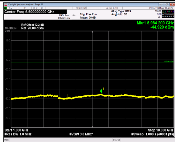
5-5-10MHz-10MHz-16QAM-16QAM-20501-20600-1RB#0-1 RB#49-1000~10000MHz-PASS
