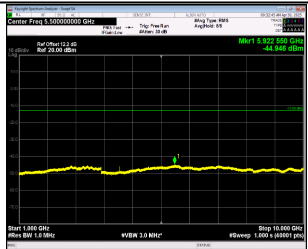
5-5-10MHz-10MHz-16QAM-16QAM-20476-20575-50RB#0- 50RB#0-1000~10000MHz-PASS
