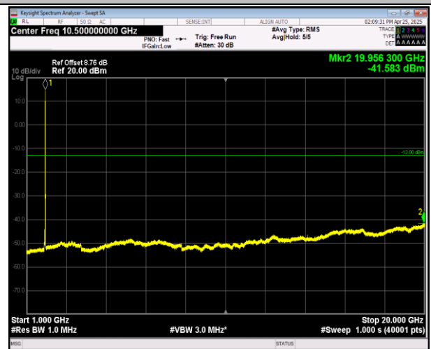
2-2-5MHz-20MHz-16QAM-16QAM-18983-19100-1RB#0-0RB B#0-1000~20000MHz-PASS
