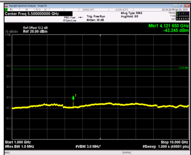
5-5-3MHz-5MHz-16QAM-16QAM-20416-20455-1RB#0-1R B#24-1000~10000MHz-PASS
