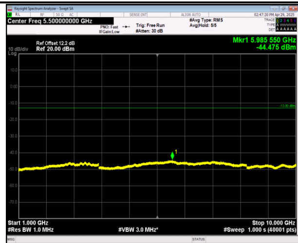
5-5-5MHz-3MHz-QPSK-QPSK-20425-20464-1RB#0-0RB#0 -1000~10000MHz-PASS
