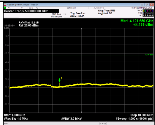
5-5-5MHz-3MHz-16QAM-16QAM-20425-20464-1RB#0-1R B#15-1000~10000MHz-PASS
