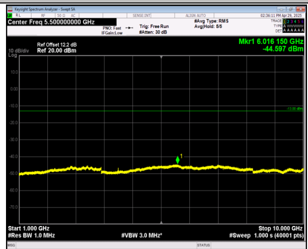
5-5-3MHz-5MHz-QPSK-QPSK-20416-20455-1RB#14-0RB# 0-1000~10000MHz-PASS
