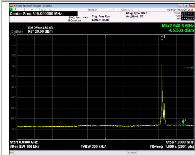
5-5-3MHz-5MHz-16QAM-16QAM-20416-20455-1RB#0-1 RB#24-30~1000MHz-PASS
