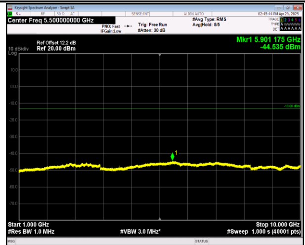
5-5-3MHz-5MHz-QPSK-QPSK-20586-20625-1RB#14-0RB# 0-1000~10000MHz-PASS
