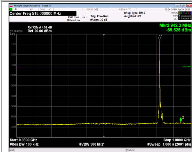
5-5-5MHz-3MHz-16QAM-16QAM-20425-20464-1RB#0-1 RB#15-30~1000MHz-PASS
