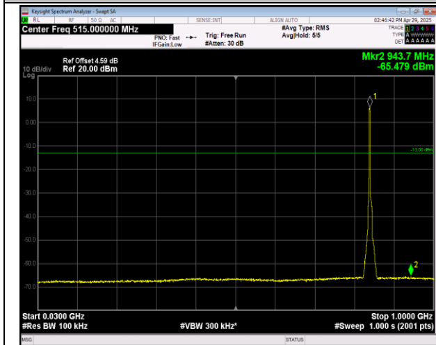
5-5-3MHz-5MHz-16QAM-16QAM-20586-20625-1RB#0-0 RB#0-30~1000MHz-PASS
