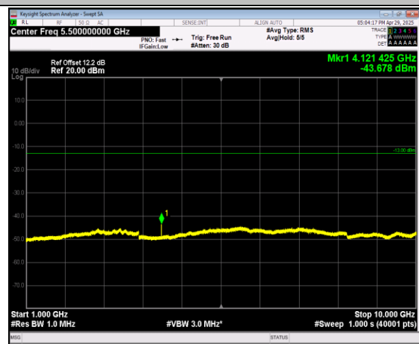
5-5-5MHz-3MHz-QPSK-QPSK-20425-20464-1RB#0-1RB#1 5-1000~10000MHz-PASS
