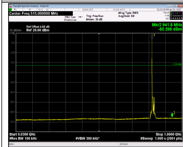
5-5-3MHz-5MHz-QPSK-QPSK-20416-20455-1RB#0-1RB #24-30~1000MHz-PASS
