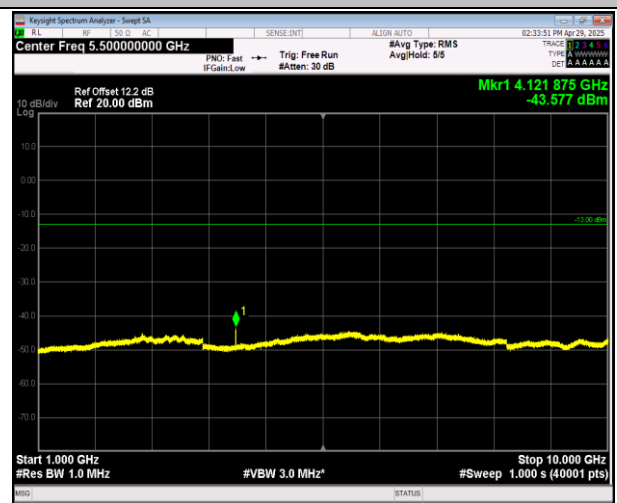
5-5-3MHz-5MHz-QPSK-QPSK-20416-20455-1RB#0-1RB#2 4-1000~10000MHz-PASS
