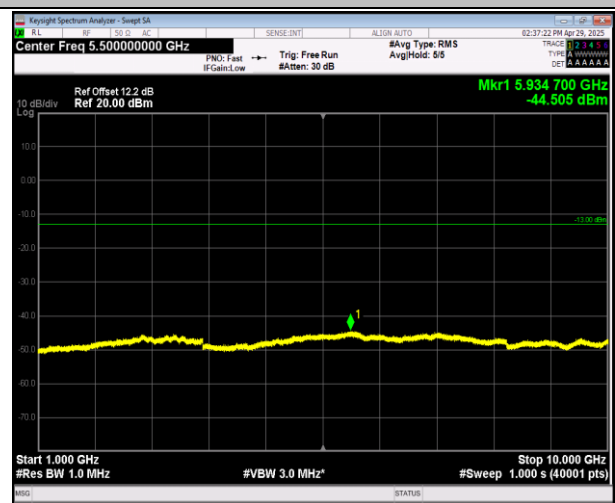
5-5-3MHz-5MHz-16QAM-16QAM-20416-20455-1RB#0-0R B#0-1000~10000MHz-PASS
