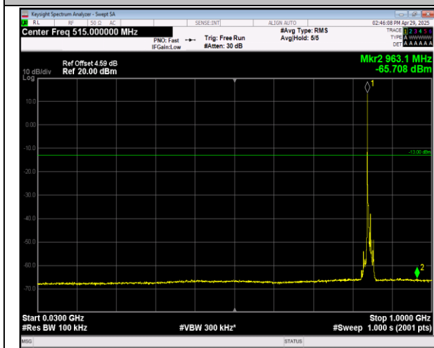
5-5-3MHz-5MHz-16QAM-16QAM-20586-20625-1RB#14- 0RB#0-30~1000MHz-PASS
