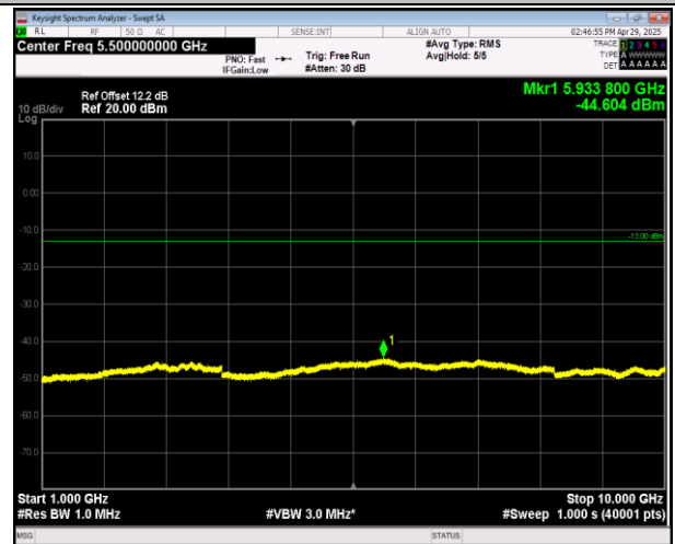
5-5-3MHz-5MHz-16QAM-16QAM-20586-20625-1RB#0-0R B#0-1000~10000MHz-PASS
