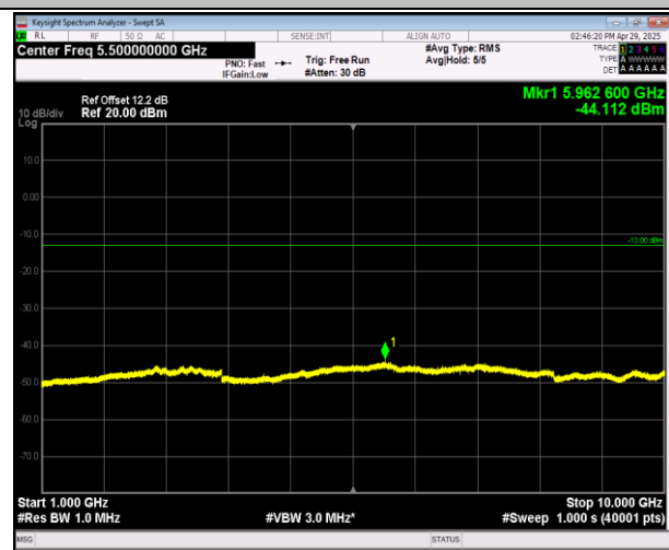
5-5-3MHz-5MHz-16QAM-16QAM-20586-20625-1RB#14-0R B#0-1000~10000MHz-PASS
