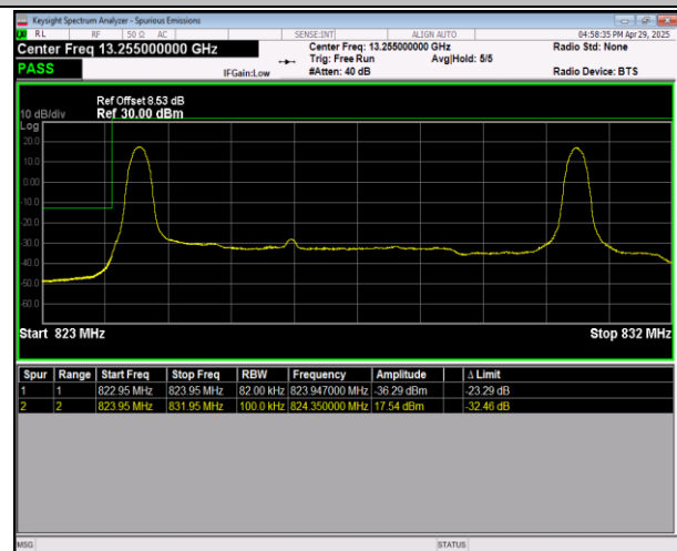
5-5-5MHz-3MHz-16QAM@16QAM-16QAM@16QAM-2042 5-20464-25RB#0@25RB#0-15RB#0@15RB#0-PASS
