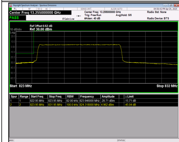
5-5-5MHz-3MHz-16QAM@16QAM-16QAM@16QAM-204 25-20464-1RB#24@25RB#0-0RB#0@15RB#0-PASS
