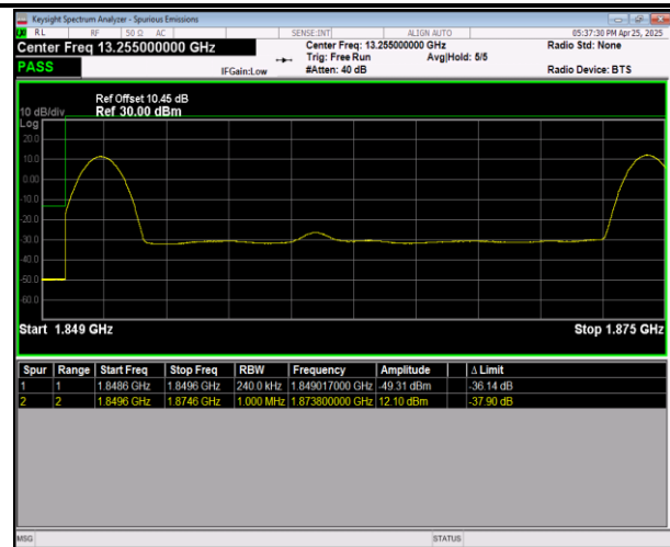
2-2-20MHz-5MHz-QPSK@QPSK-QPSK@QPSK-18700-18817-100RB#0@100RB#0-25RB#0@25RB#0-PASS
