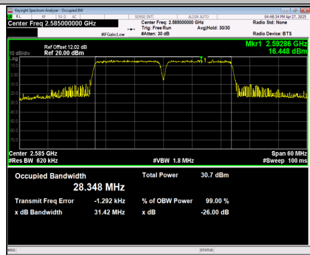
38-38-15MHz-15MHz-16QAM-16QAM-37925-38075-75RB #0-75RB#0-PASS
