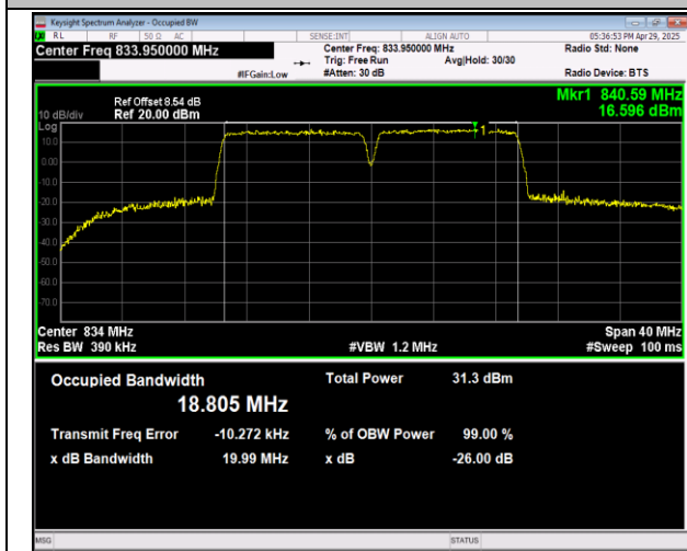
5-5-10MHz-10MHz-QPSK-QPSK-20476-20575-50RB#0-5 ORB#0-PASS
