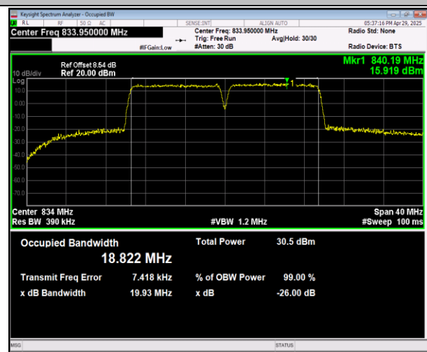
5-5-10MHz-10MHz-16QAM-16QAM-20476-20575-50RB#0-5 50RB#0-PASS
