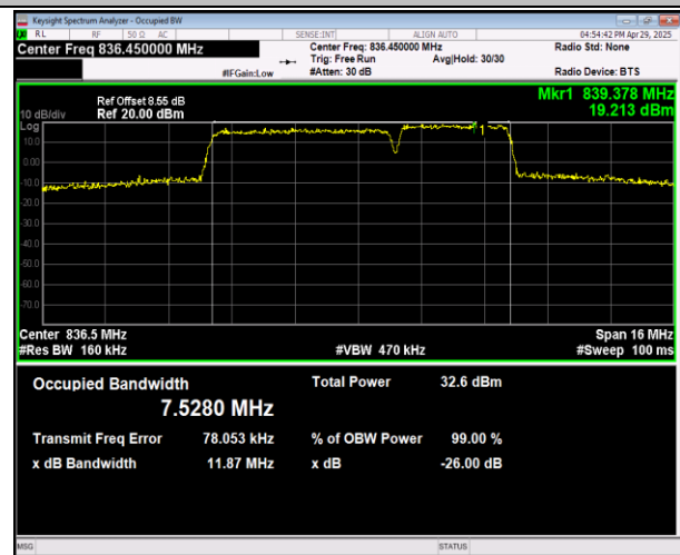
5-5-5MHz-3MHz-16QAM-16QAM-20595-20634-25RB#0-15 RB#0-PASS
