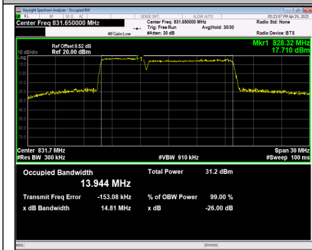
5-5-5MHz-10MHz-QPSK-QPSK-20478-20550-25RB#0-50 RB#0-PASS
