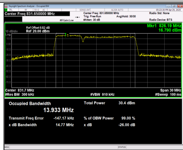
5-5-5MHz-10MHz-16QAM-16QAM-20478-20550-25RB#0-5 ORB#0-PASS
