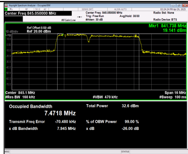
5-5-5MHz-3MHz-16QAM-16QAM-20425-20464-25RB#0-15 RB#0-PASS
