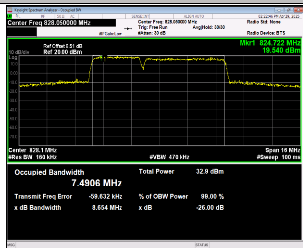
5-5-3MHz-5MHz-16QAM-16QAM-20501-20540-15RB#0-25 RB#0-PASS
