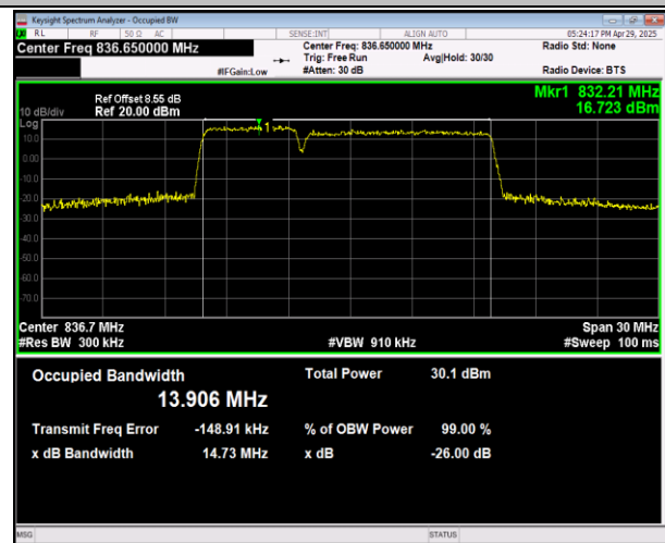
5-5-5MHz-10MHz-16QAM-16QAM-20528-20600-25RB#0-5 ORB#0-PASS
