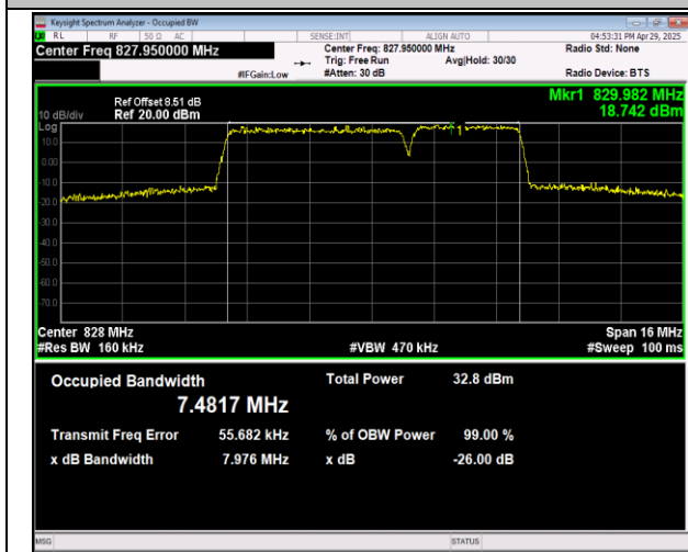
5-5-5MHz-3MHz-QPSK-QPSK-20510-20549-25RB#0-15 RB#0-PASS
