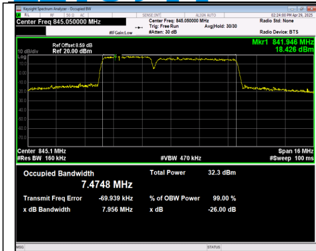
5-5-5MHz-3MHz-QPSK-QPSK-20425-20464-25RB#0-15 RB#0-PASS
