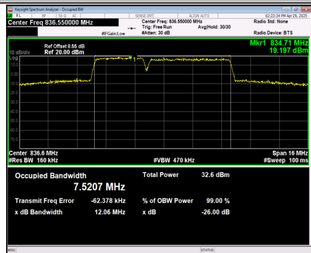
5-5-3MHz-5MHz-16QAM-16QAM-20586-20625-15RB#0-25 RB#0-PASS
