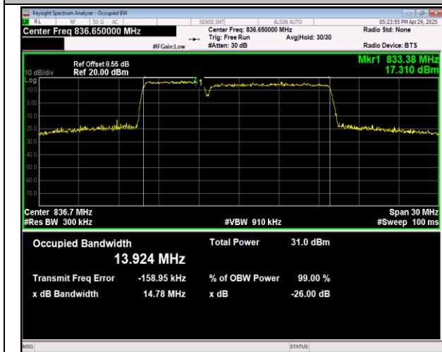
5-5-5MHz-10MHz-QPSK-QPSK-20528-20600-25RB#0-50 RB#0-PASS
