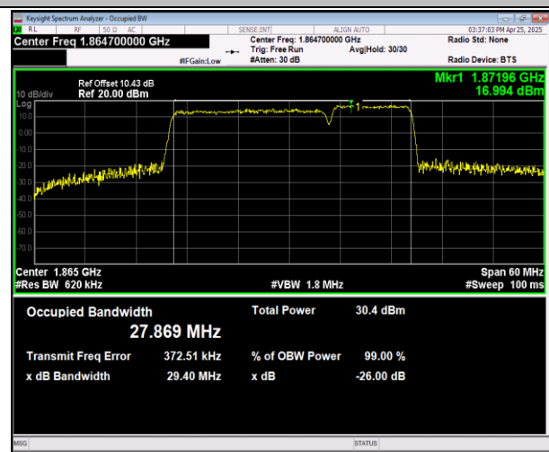
2-2-20MHz-10MHz-16QAM-16QAM-1864-1864-100RB#0-50RB#0-PASS
