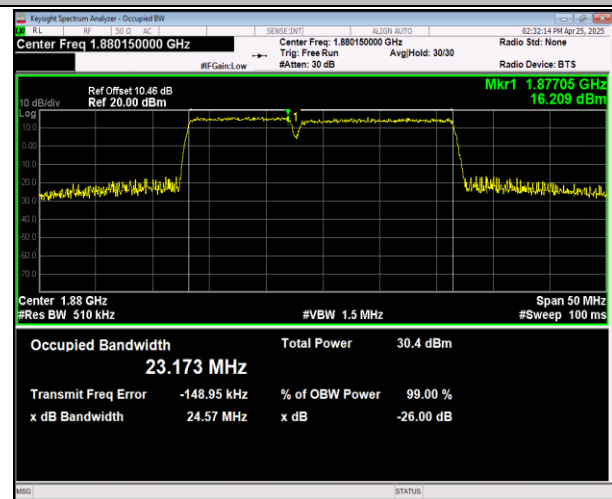
2-2-10MHz-15MHz-16QAM-16QAM-19005-19125-50RB#0- 75RB#0-PASS
