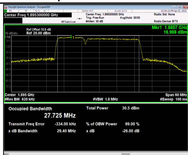
2-2-15MHz-10MHz-16QAM-16QAM-18675-18795-75RB#0-5 50RB#0-PASS
