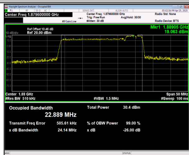
2-2-20MHz-5MHz-16QAM-16QAM-19050-19167-100RB#0- 25RB#0-PASS
