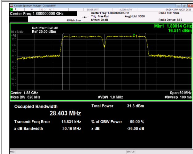
2-2-15MHz-15MHz-QPSK-QPSK-18975-19125-75RB#0-7 5RB#0-PASS
