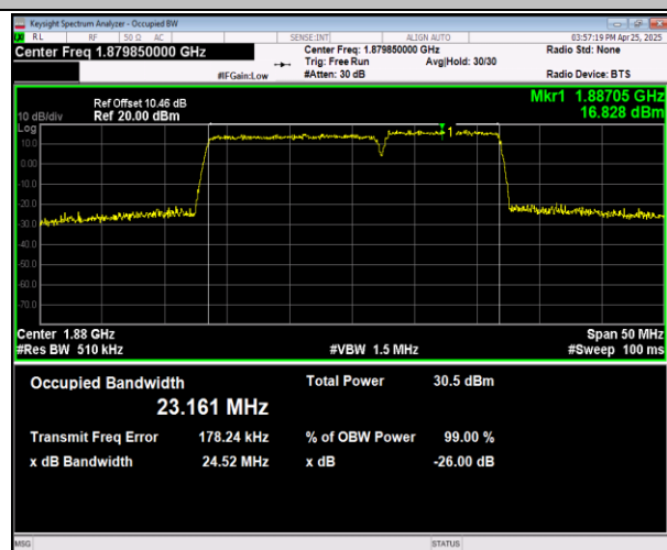
2-2-15MHz-10MHz-16QAM-16QAM-19027-19147-75RB#0-5 50RB#0-PASS
