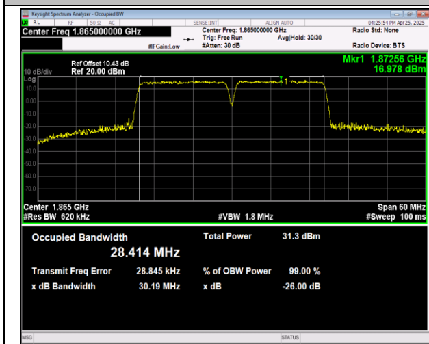
2-2-15MHz-15MHz-QPSK-QPSK-18825-18975-75RB#0-7 5RB#0-PASS
