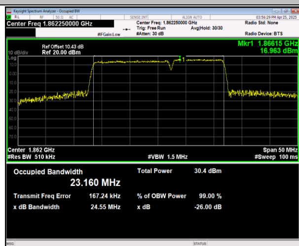
2-2-15MHz-10MHz-16QAM-16QAM-18851-18971-75RB#0-5 50RB#0-PASS
