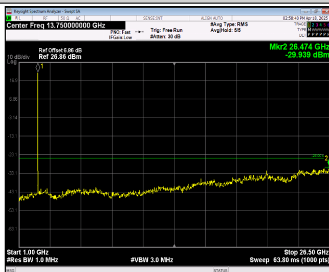
Band38-5MHz-QPSK-37775-1RB#0-Range2:1000~26500MHz
