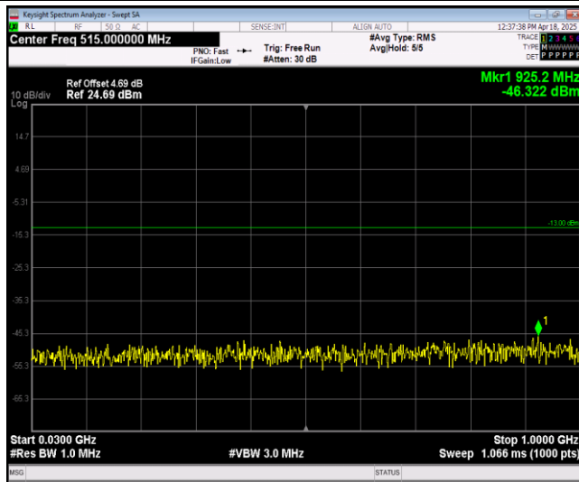
Band2-20MHz-64QAM-18900-1RB#0-Range1:30~1000MHz
