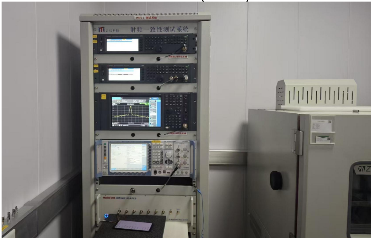
Conducted method(WiFi mode)
