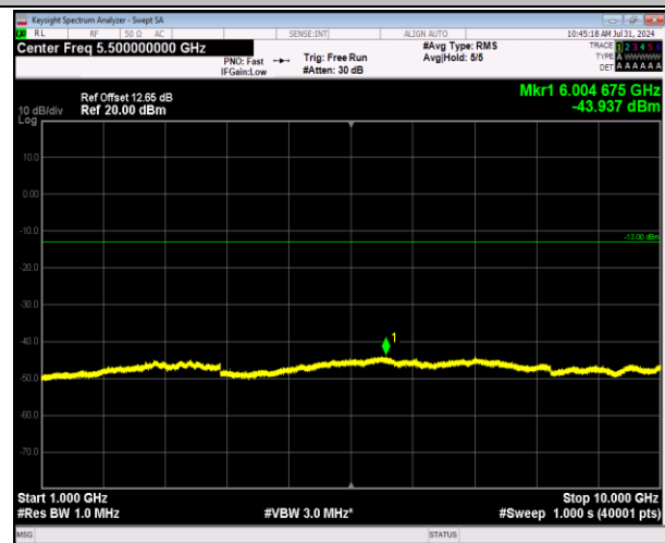
5-5-3MHz-5MHz-64QAM-64QAM-20416-20455-15RB#0- 25RB#0-1000~10000MHz-PASS
