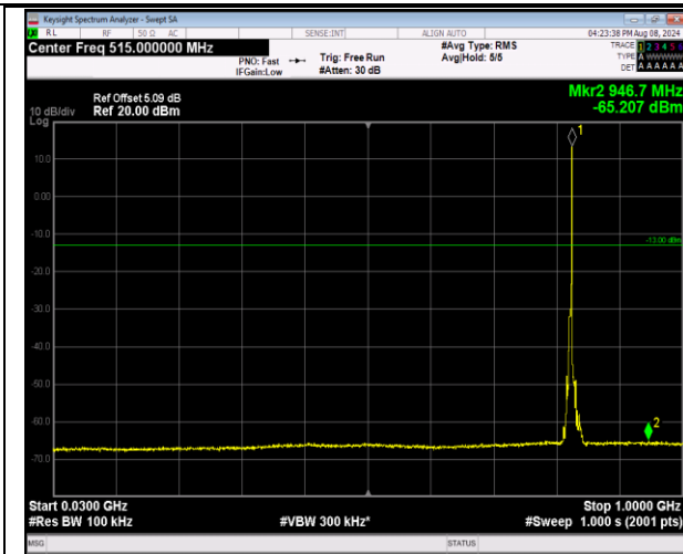
5-5-5MHz-3MHz-16QAM-16QAM-20425-20464-1RB#24- ORB#0-30~1000MHz-PASS
