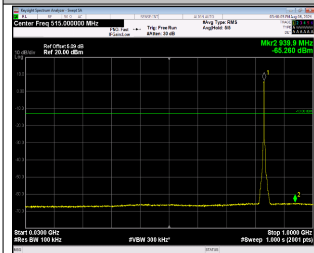
5-5-3MHz-5MHz-16QAM-16QAM-20501-20540-15RB#0-25RB#0-30~1000MHz-PASS
