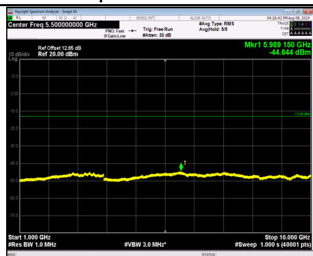
5-5-5MHz-3MHz-QPSK-QPSK-20510-20549-1RB#0-0RB #0-1000~10000MHz-PASS
