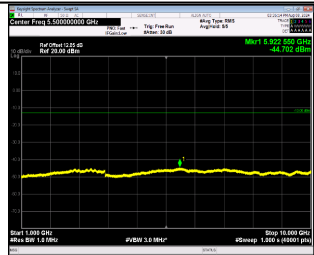
5-5-3MHz-5MHz-QPSK-QPSK-20501-20540-1RB#0-0RB #0-1000~10000MHz-PASS
