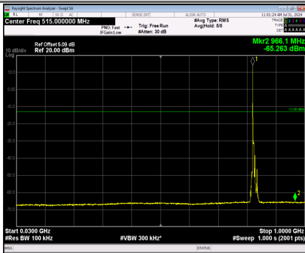
5-5-5MHz-3MHz-64QAM-64QAM-20425-20464-1RB#0-0 RB#0-30~1000MHz-PASS
