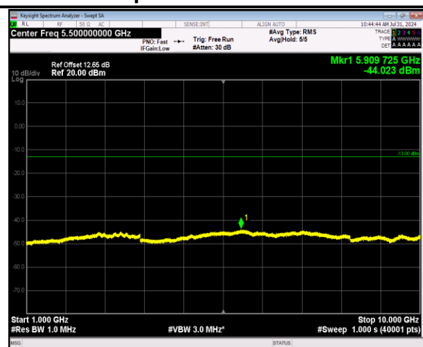
5-5-3MHz-5MHz-64QAM-64QAM-20416-20455-1RB#0-1 RB#24-1000~10000MHz-PASS
