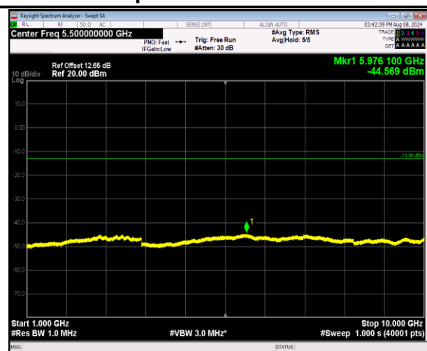
5-5-3MHz-5MHz-16QAM-16QAM-20586-20625-1RB#14-ORB#0-1000~10000MHz-PASS
