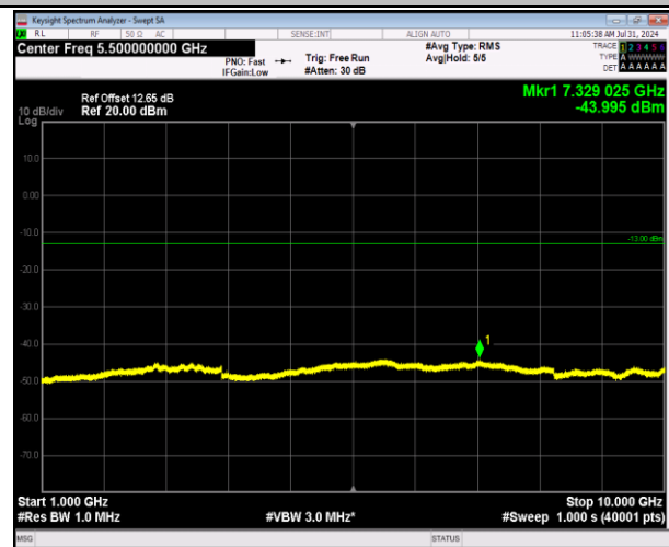
5-5-5MHz-3MHz-64QAM-64QAM-20510-20549-25RB#0- 15RB#0-1000~10000MHz-PASS
