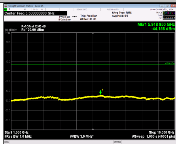
5-5-3MHz-5MHz-64QAM-64QAM-20501-20540-1RB#14- ORB#0-1000~10000MHz-PASS
