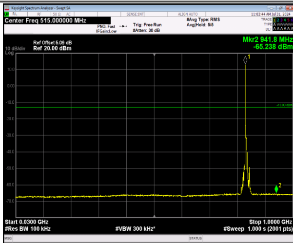
5-5-5MHz-3MHz-64QAM-64QAM-20510-20549-1RB#0-0RB#0-30~1000MHz-PASS
