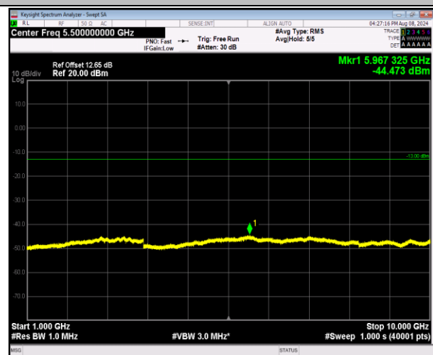
5-5-5MHz-3MHz-16QAM-16QAM-20510-20549-1RB#0-0 RB#0-1000~10000MHz-PASS
