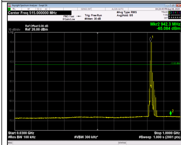
5-5-5MHz-3MHz-16QAM-16QAM-20425-20464-1RB#0-1 RB#15-30~1000MHz-PASS
