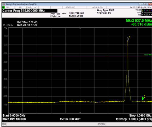
5-5-5MHz-3MHz-16QAM-16QAM-20510-20549-25RB#0-15RB#0-30~1000MHz-PASS
