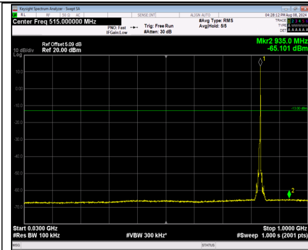
5-5-5MHz-3MHz-16QAM-16QAM-20510-20549-1RB#24-ORB#0-30~1000MHz-PASS
