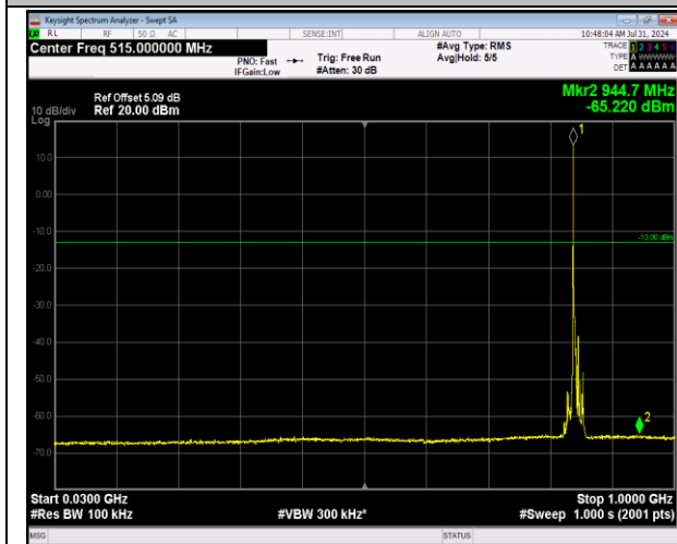
5-5-3MHz-5MHz-64QAM-64QAM-20586-20625-1RB#0-0RB#0-30~1000MHz-PASS
