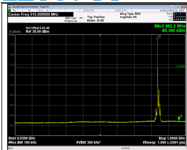
5-5-3MHz-5MHz-64QAM-64QAM-20586-20625-1RB#0-1 RB#24-30~1000MHz-PASS
