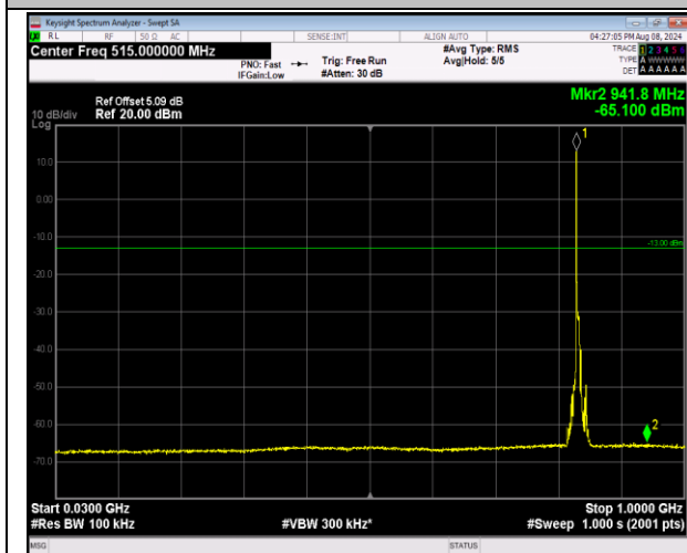
5-5-5MHz-3MHz-16QAM-16QAM-20510-20549-1RB#0-0 RB#0-30~1000MHz-PASS
