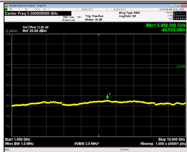
5-5-3MHz-5MHz-64QAM-64QAM-20501-20540-1RB#0-0RB#0-1000~10000MHz-PASS
