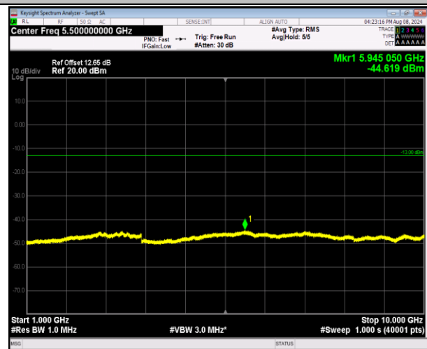
5-5-5MHz-3MHz-QPSK-QPSK-20425-20464-1RB#24-0R B#0-1000~10000MHz-PASS
