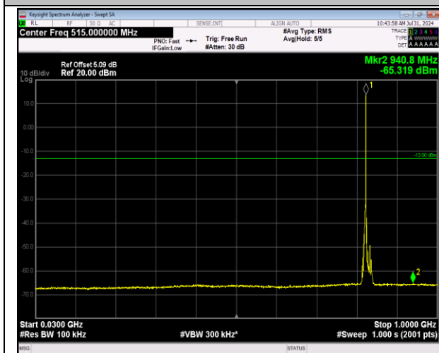
5-5-3MHz-5MHz-64QAM-64QAM-20416-20455-1RB#14- ORB#0-30~1000MHz-PASS
