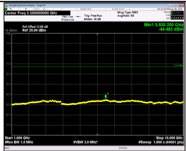
5-5-5MHz-3MHz-16QAM-16QAM-20425-20464-1RB#24- ORB#0-1000~10000MHz-PASS
