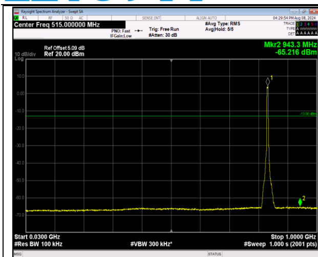
5-5-5MHz-3MHz-QPSK-QPSK-20510-20549-25RB#0-15 RB#0-30~1000MHz-PASS
