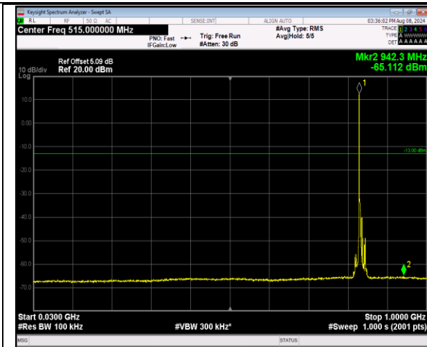
5-5-3MHz-5MHz-QPSK-QPSK-20501-20540-1RB#0-0R B#0-30~1000MHz-PASS
