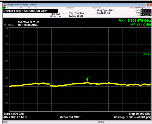
5-5-3MHz-5MHz-16QAM-16QAM-20586-20625-1RB#0-1 RB#24-1000~10000MHz-PASS
