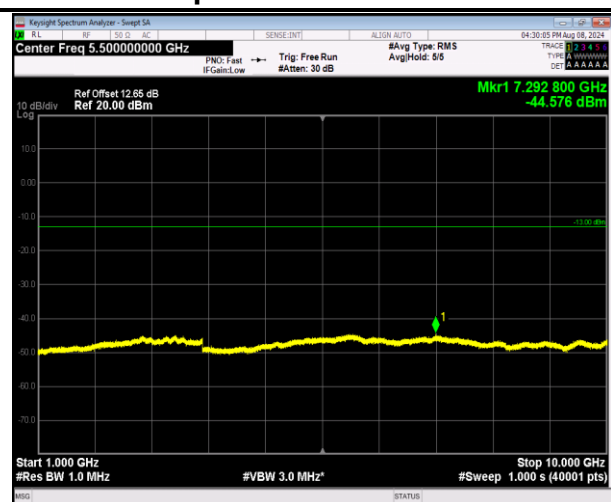
5-5-5MHz-3MHz-QPSK-QPSK-20510-20549-25RB#0-15 RB#0-1000~10000MHz-PASS
