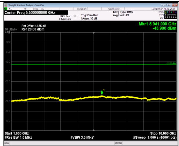
5-5-5MHz-3MHz-64QAM-64QAM-20425-20464-1RB#0-1 RB#15-1000~10000MHz-PASS
