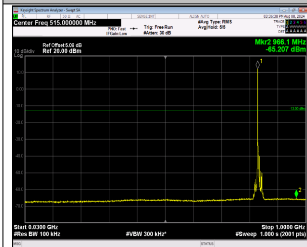
5-5-3MHz-5MHz-16QAM-16QAM-20501-20540-1RB#0-0 RB#0-30~1000MHz-PASS
