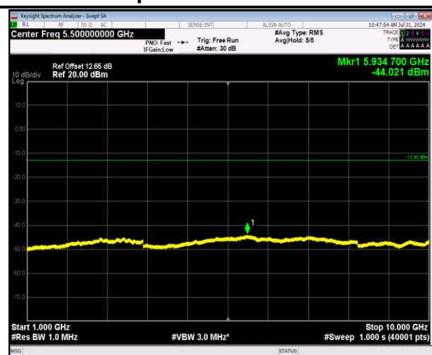
5-5-3MHz-5MHz-64QAM-64QAM-20501-20540-1RB#0-1 RB#24-1000~10000MHz-PASS
