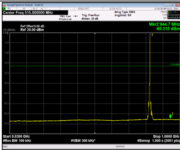
5-5-5MHz-3MHz-64QAM-64QAM-20425-20464-1RB#24- ORB#0-30~1000MHz-PASS
