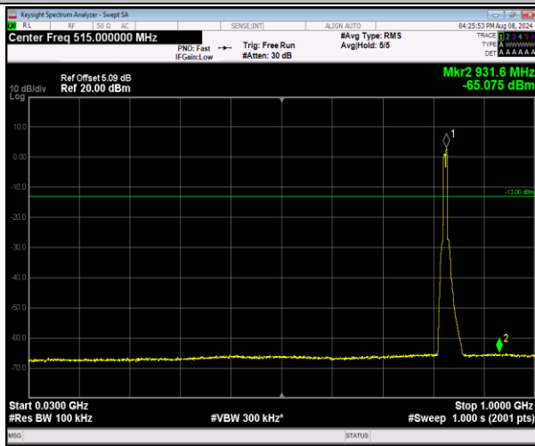
5-5-5MHz-3MHz-16QAM-16QAM-20425-20464-25RB#0- 15RB#0-30~1000MHz-PASS
