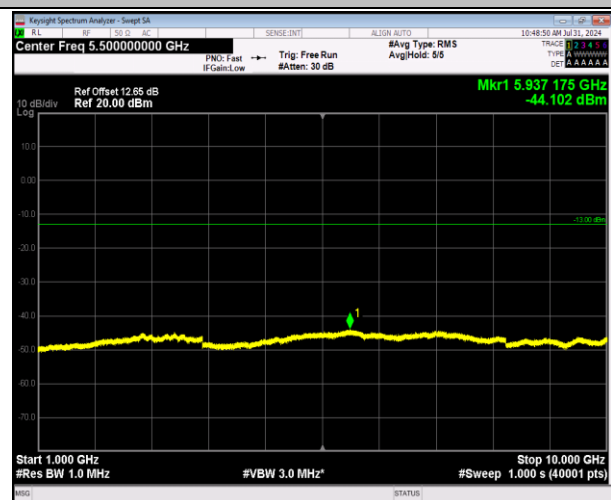
5-5-3MHz-5MHz-64QAM-64QAM-20586-20625-1RB#14- ORB#0-1000~10000MHz-PASS
