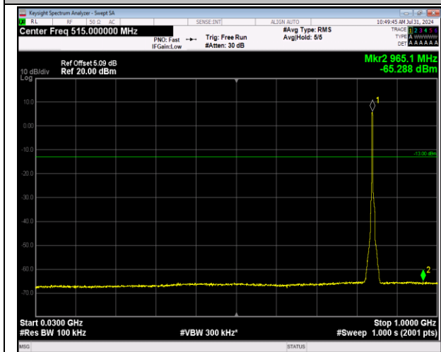
5-5-3MHz-5MHz-64QAM-64QAM-20586-20625-15RB#0- 25RB#0-30~1000MHz-PASS
