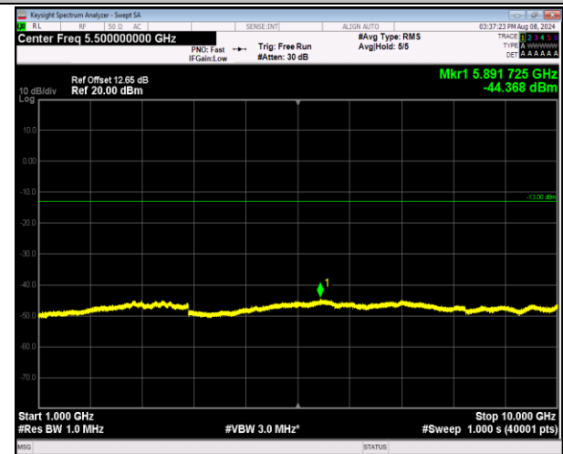
5-5-3MHz-5MHz-QPSK-QPSK-20501-20540-1RB#14-0R B#0-1000~10000MHz-PASS
