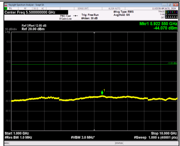
5-5-5MHz-3MHz-64QAM-64QAM-20510-20549-1RB#0-0RB#0-1000~10000MHz-PASS
