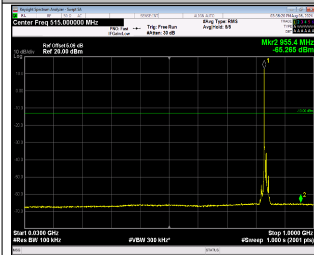
5-5-3MHz-5MHz-QPSK-QPSK-20501-20540-1RB#0-1R B#24-30~1000MHz-PASS
