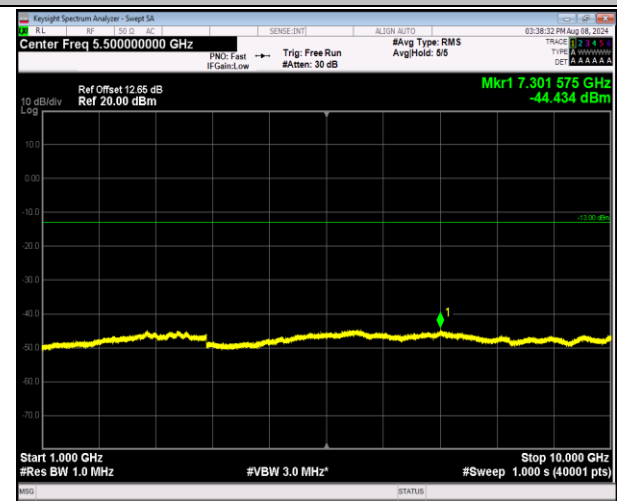
5-5-3MHz-5MHz-QPSK-QPSK-20501-20540-1RB#0-1RB #24-1000~10000MHz-PASS
