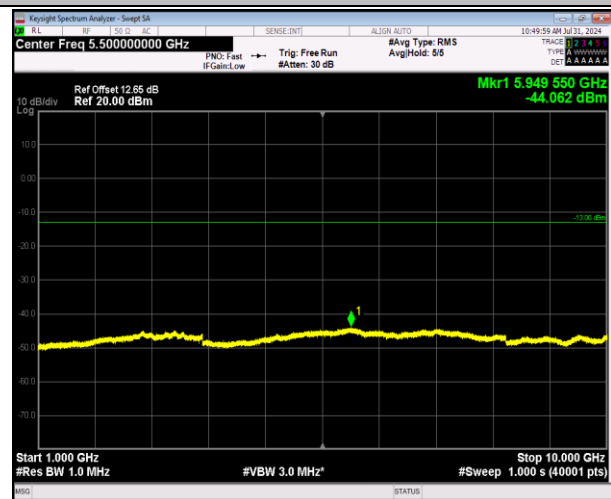
5-5-3MHz-5MHz-64QAM-64QAM-20586-20625-15RB#0- 25RB#0-1000~10000MHz-PASS
