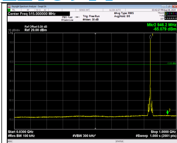
5-5-3MHz-5MHz-16QAM-16QAM-20586-20625-1RB#14-ORB#0-30~1000MHz-PASS
