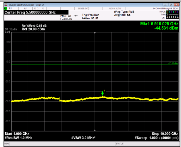
5-5-5MHz-3MHz-16QAM-16QAM-20510-20549-25RB#0-15RB#0-1000~10000MHz-PASS
