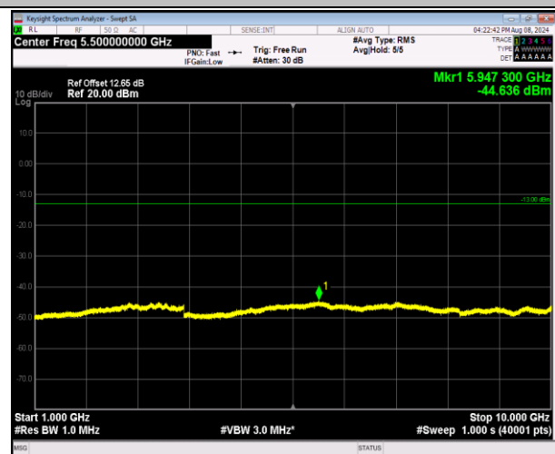
5-5-5MHz-3MHz-16QAM-16QAM-20425-20464-1RB#0-0 RB#0-1000~10000MHz-PASS
