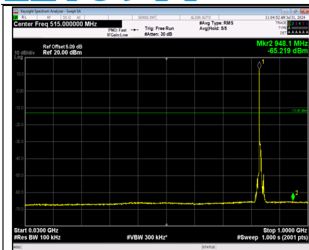
5-5-5MHz-3MHz-64QAM-64QAM-20510-20549-1RB#0-1 RB#15-30~1000MHz-PASS
