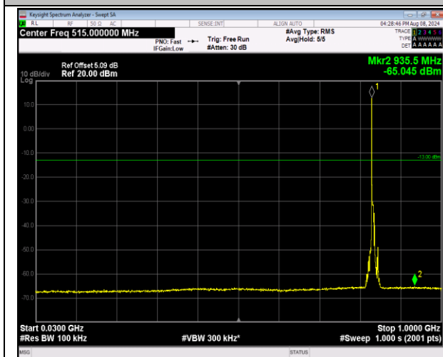
5-5-5MHz-3MHz-QPSK-QPSK-20510-20549-1RB#0-1R B#15-30~1000MHz-PASS
