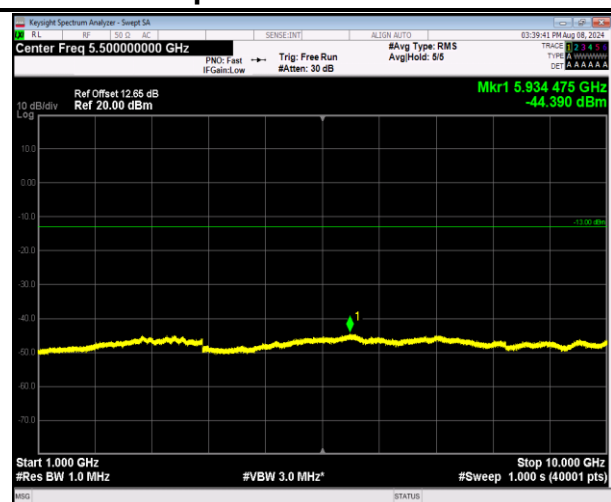
5-5-3MHz-5MHz-QPSK-QPSK-20501-20540-15RB#0-25 RB#0-1000~10000MHz-PASS
