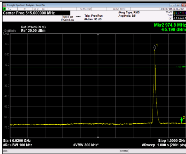
5-5-5MHz-3MHz-64QAM-64QAM-20425-20464-25RB#0- 15RB#0-30~1000MHz-PASS
