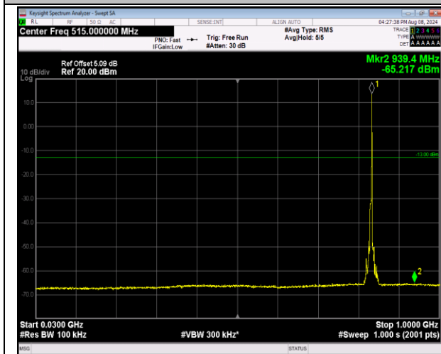
5-5-5MHz-3MHz-QPSK-QPSK-20510-20549-1RB#24-0R B#0-30~1000MHz-PASS
