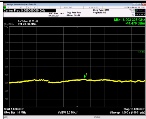
5-5-3MHz-5MHz-16QAM-16QAM-20501-20540-1RB#0-1 RB#24-1000~10000MHz-PASS
