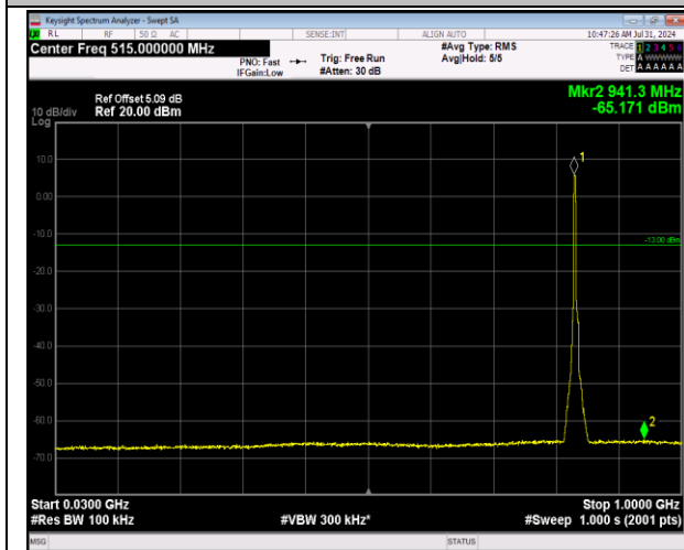
5-5-3MHz-5MHz-64QAM-64QAM-20501-20540-15RB#0- 25RB#0-30~1000MHz-PASS
