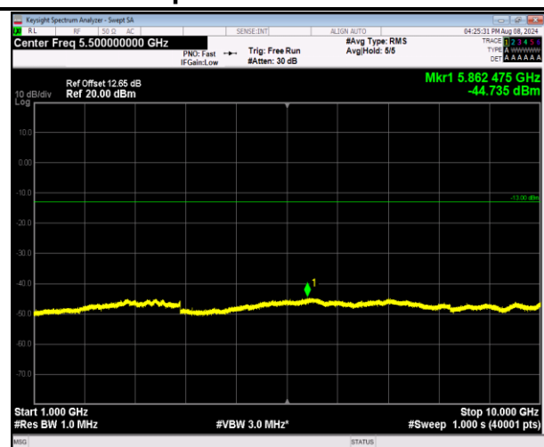
5-5-5MHz-3MHz-QPSK-QPSK-20425-20464-25RB#0-15 RB#0-1000~10000MHz-PASS
