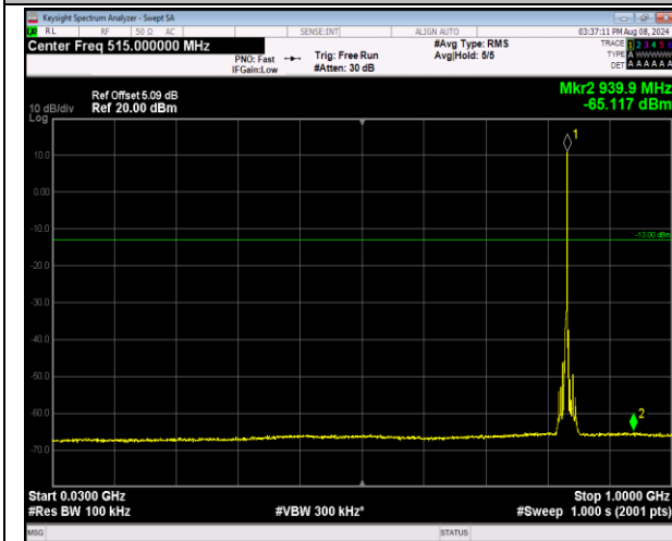
5-5-3MHz-5MHz-QPSK-QPSK-20501-20540-1RB#14-0R B#0-30~1000MHz-PASS
