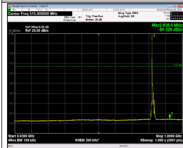
5-5-5MHz-3MHz-16QAM-16QAM-20425-20464-1RB#0-0 RB#0-30~1000MHz-PASS
