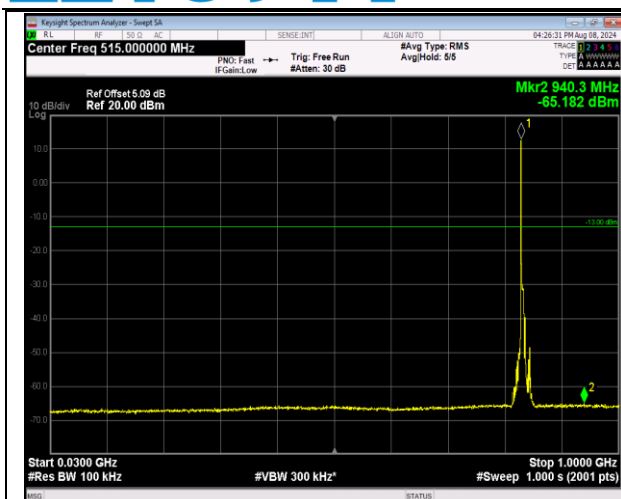
5-5-5MHz-3MHz-QPSK-QPSK-20510-20549-1RB#0-0R B#0-30~1000MHz-PASS
