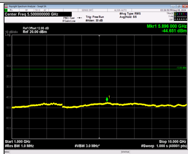
5-5-3MHz-5MHz-16QAM-16QAM-20501-20540-1RB#0-0 RB#0-1000~10000MHz-PASS
