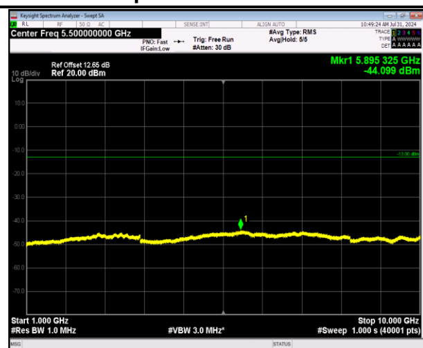
5-5-3MHz-5MHz-64QAM-64QAM-20586-20625-1RB#0-1 RB#24-1000~10000MHz-PASS
