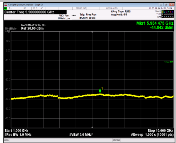
5-5-5MHz-3MHz-64QAM-64QAM-20425-20464-25RB#0- 15RB#0-1000~10000MHz-PASS
