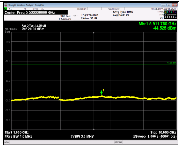
5-5-5MHz-3MHz-16QAM-16QAM-20510-20549-1RB#24-ORB#0-1000~10000MHz-PASS
