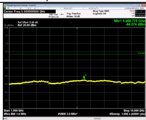
5-5-5MHz-3MHz-64QAM-64QAM-20510-20549-1RB#0-1 RB#15-1000~10000MHz-PASS
