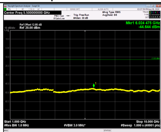
5-5-3MHz-5MHz-16QAM-16QAM-20501-20540-1RB#14-ORB#0-1000~10000MHz-PASS
