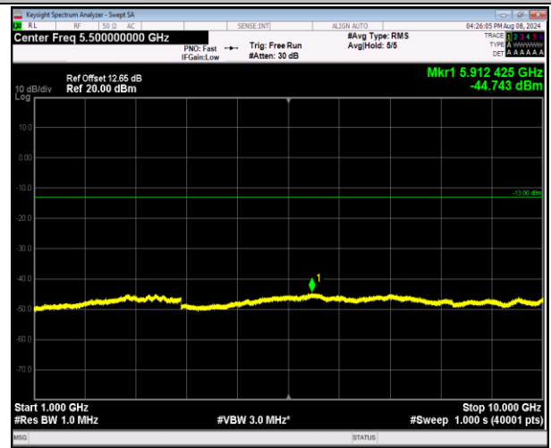
5-5-5MHz-3MHz-16QAM-16QAM-20425-20464-25RB#0- 15RB#0-1000~10000MHz-PASS
