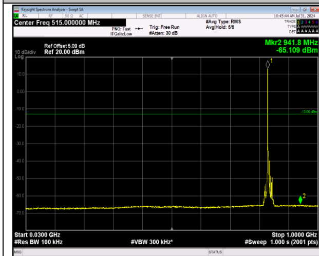
5-5-3MHz-5MHz-64QAM-64QAM-20501-20540-1RB#0-0RB#0-30~1000MHz-PASS
