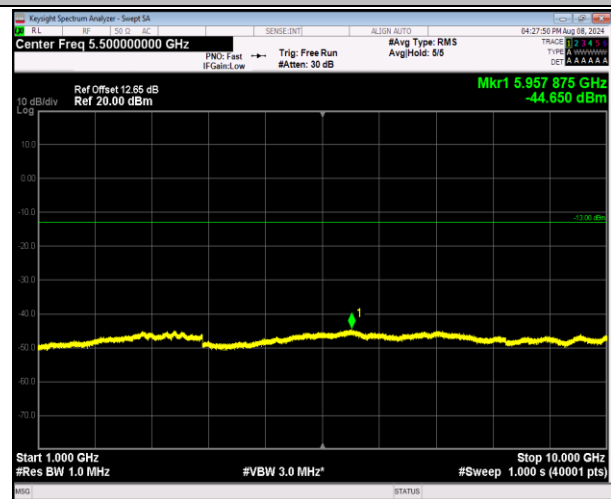
5-5-5MHz-3MHz-QPSK-QPSK-20510-20549-1RB#24-0R B#0-1000~10000MHz-PASS
