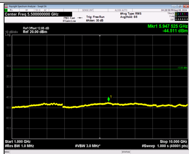
5-5-5MHz-3MHz-QPSK-QPSK-20510-20549-1RB#0-1RB #15-1000~10000MHz-PASS
