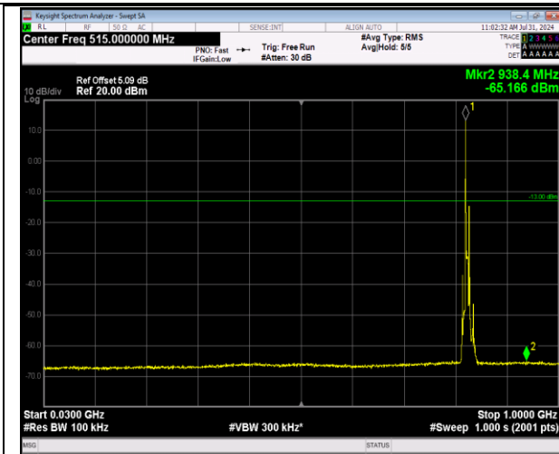
5-5-5MHz-3MHz-64QAM-64QAM-20425-20464-1RB#0-1 RB#15-30~1000MHz-PASS
