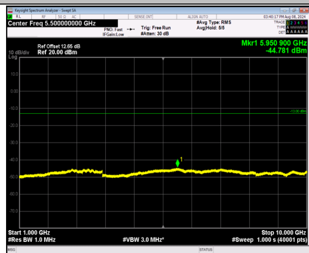
5-5-3MHz-5MHz-16QAM-16QAM-20501-20540-15RB#0-25RB#0-1000~10000MHz-PASS
