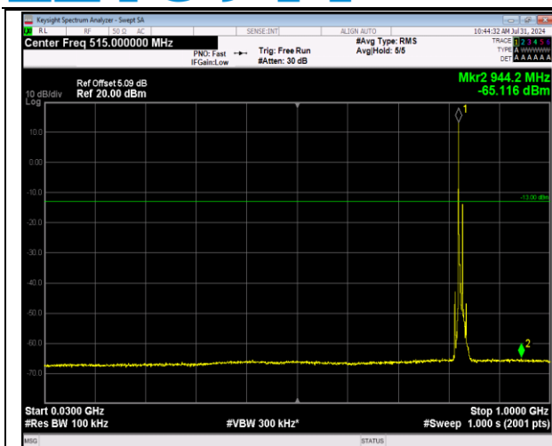
5-5-3MHz-5MHz-64QAM-64QAM-20416-20455-1RB#0-1 RB#24-30~1000MHz-PASS
