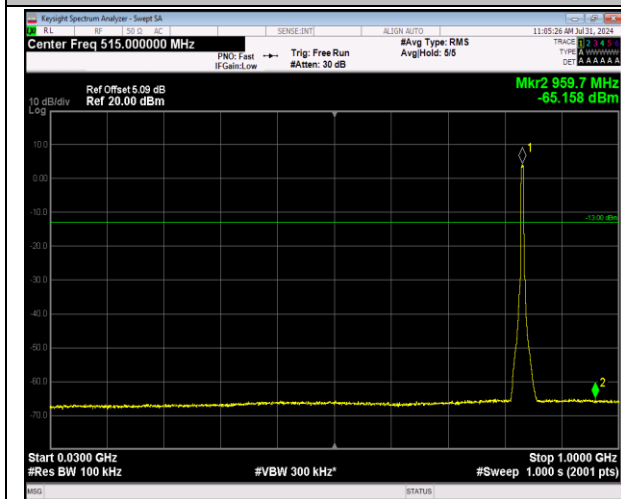
5-5-5MHz-3MHz-64QAM-64QAM-20510-20549-25RB#0- 15RB#0-30~1000MHz-PASS
