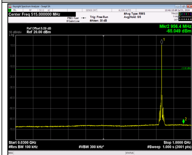
5-5-3MHz-5MHz-64QAM-64QAM-20501-20540-1RB#14- ORB#0-30~1000MHz-PASS
