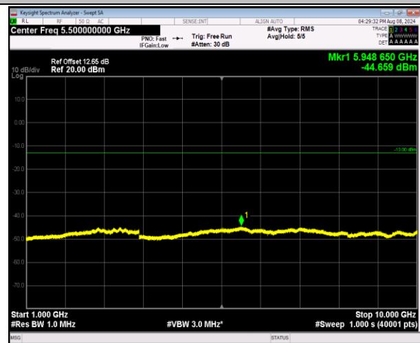
5-5-5MHz-3MHz-16QAM-16QAM-20510-20549-1RB#0-1 RB#15-1000~10000MHz-PASS
