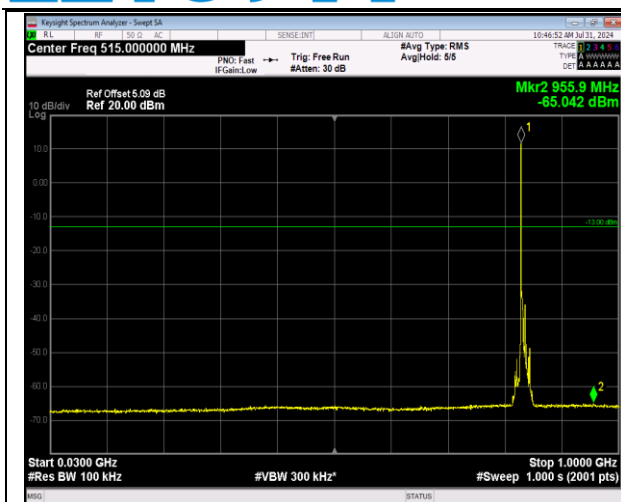
5-5-3MHz-5MHz-64QAM-64QAM-20501-20540-1RB#0-1 RB#24-30~1000MHz-PASS
