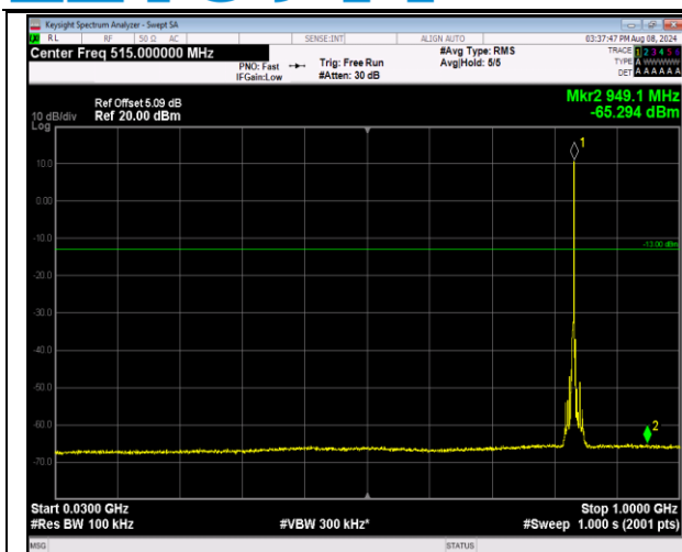
5-5-3MHz-5MHz-16QAM-16QAM-20501-20540-1RB#14-ORB#0-30~1000MHz-PASS
