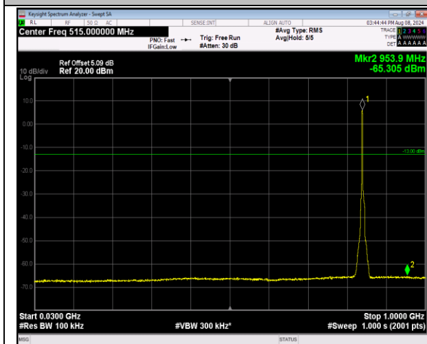
5-5-3MHz-5MHz-16QAM-16QAM-20586-20625-15RB#0-25RB#0-30~1000MHz-PASS
