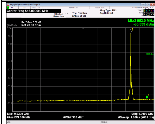
5-5-3MHz-5MHz-16QAM-16QAM-20586-20625-1RB#0-1 RB#24-30~1000MHz-PASS
