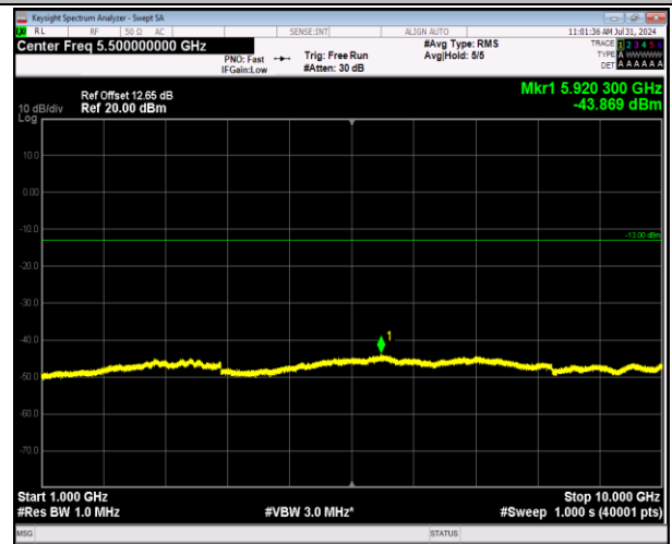
5-5-5MHz-3MHz-64QAM-64QAM-20425-20464-1RB#0-0 RB#0-1000~10000MHz-PASS
