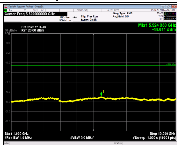
5-5-3MHz-5MHz-QPSK-QPSK-20586-20625-1RB#0-0RB #0-1000~10000MHz-PASS
