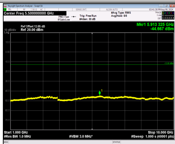
5-5-3MHz-5MHz-16QAM-16QAM-20586-20625-1RB#0-0 RB#0-1000~10000MHz-PASS
