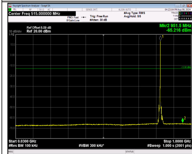
5-5-5MHz-3MHz-QPSK-QPSK-20425-20464-1RB#24-0R B#0-30~1000MHz-PASS
