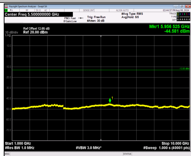
5-5-3MHz-5MHz-16QAM-16QAM-20586-20625-15RB#0-25RB#0-1000~10000MHz-PASS
