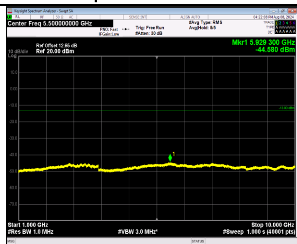
5-5-5MHz-3MHz-QPSK-QPSK-20425-20464-1RB#0-0RB #0-1000~10000MHz-PASS
