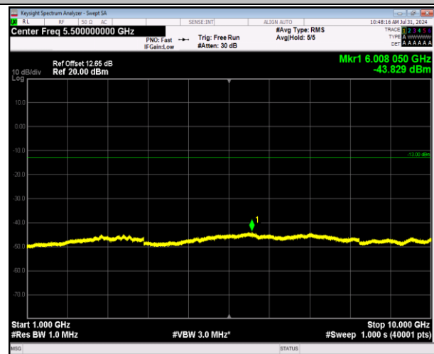
5-5-3MHz-5MHz-64QAM-64QAM-20586-20625-1RB#0-0RB#0-1000~10000MHz-PASS
