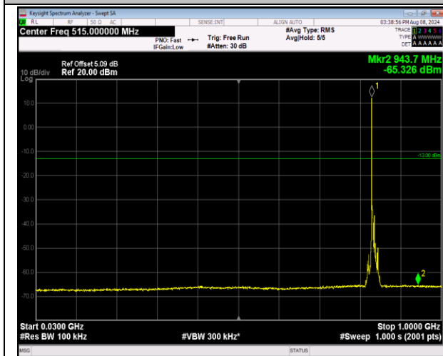
5-5-3MHz-5MHz-16QAM-16QAM-20501-20540-1RB#0-1 RB#24-30~1000MHz-PASS
