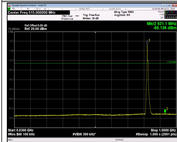
5-5-3MHz-5MHz-64QAM-64QAM-20416-20455-15RB#0- 25RB#0-30~1000MHz-PASS
