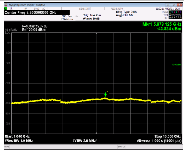
5-5-5MHz-3MHz-64QAM-64QAM-20425-20464-1RB#24- ORB#0-1000~10000MHz-PASS
