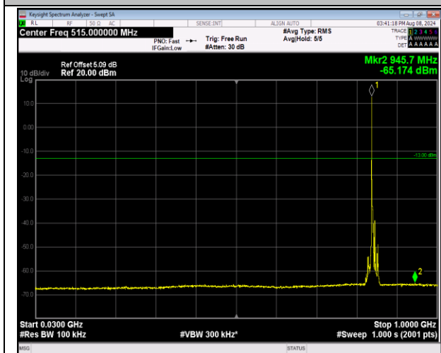
5-5-3MHz-5MHz-16QAM-16QAM-20586-20625-1RB#0-0 RB#0-30~1000MHz-PASS
