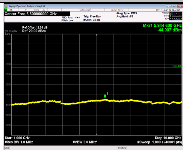
5-5-3MHz-5MHz-64QAM-64QAM-20416-20455-1RB#14- ORB#0-1000~10000MHz-PASS
