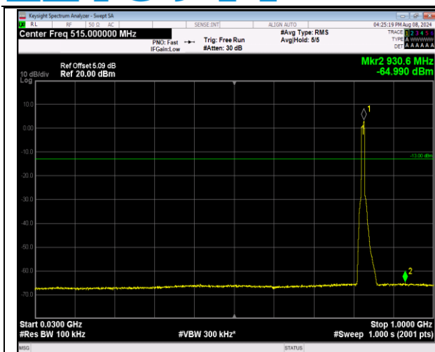
5-5-5MHz-3MHz-QPSK-QPSK-20425-20464-25RB#0-15 RB#0-30~1000MHz-PASS
