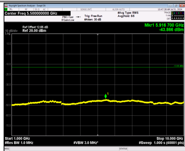
5-5-3MHz-5MHz-64QAM-64QAM-20501-20540-15RB#0- 25RB#0-1000~10000MHz-PASS
