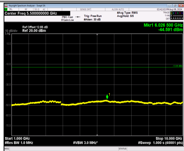
5-5-3MHz-5MHz-QPSK-QPSK-20586-20625-1RB#14-0R B#0-1000~10000MHz-PASS
