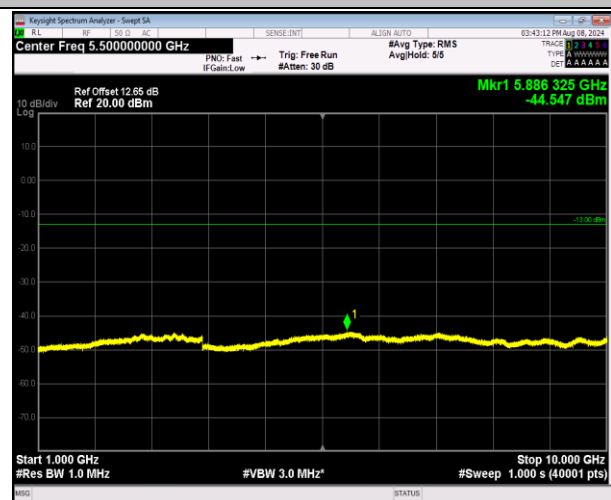
5-5-3MHz-5MHz-QPSK-QPSK-20586-20625-1RB#0-1RB #24-1000~10000MHz-PASS
