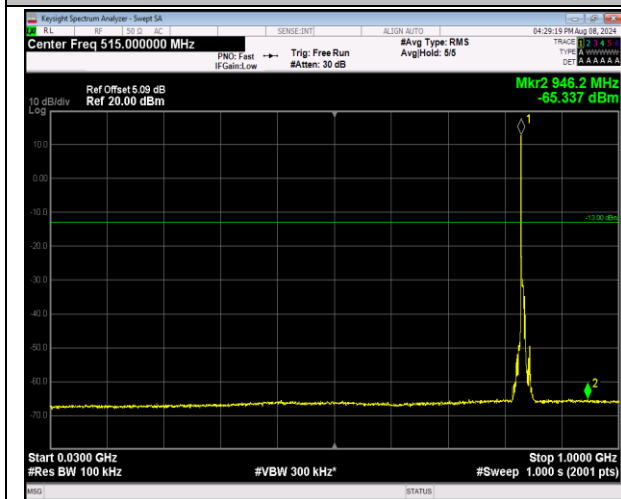
5-5-5MHz-3MHz-16QAM-16QAM-20510-20549-1RB#0-1 RB#15-30~1000MHz-PASS
