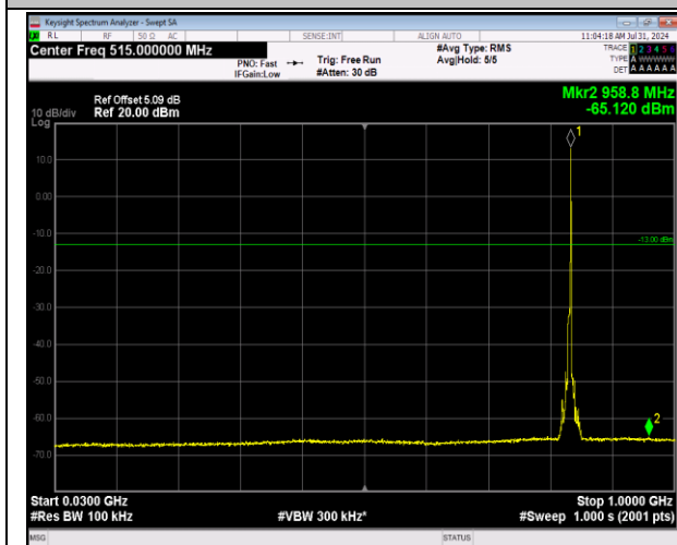
5-5-5MHz-3MHz-64QAM-64QAM-20510-20549-1RB#24- ORB#0-30~1000MHz-PASS
