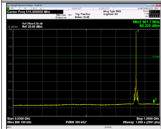
5-5-3MHz-5MHz-64QAM-64QAM-20586-20625-1RB#14- ORB#0-30~1000MHz-PASS
