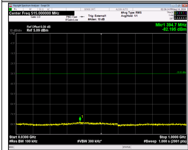
41-41-20MHz-20MHz-16QAM-16QAM-40340-40538-1RB #0-0RB#0-30~1000MHz-PASS
