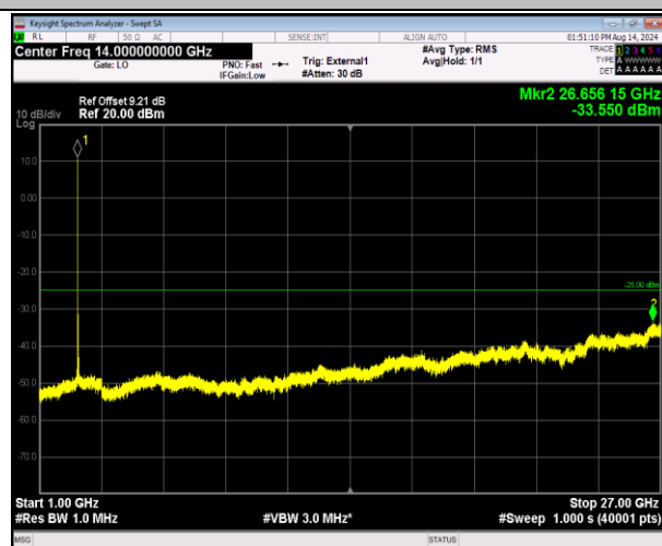
41-41-20MHz-5MHz-16QAM-16QAM-40715-40832-1RB#0- 1RB#24-1000-27000MHz-PASS
