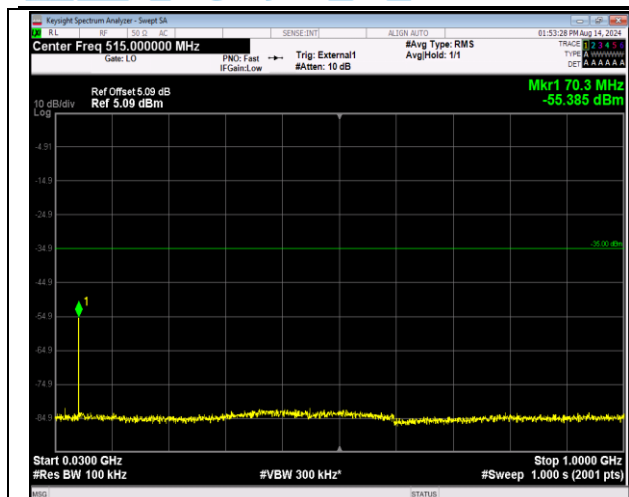
41-41-20MHz-5MHz-QPSK-QPSK-41090-41207-1RB#0-0RB#0-30~1000MHz-PASS
