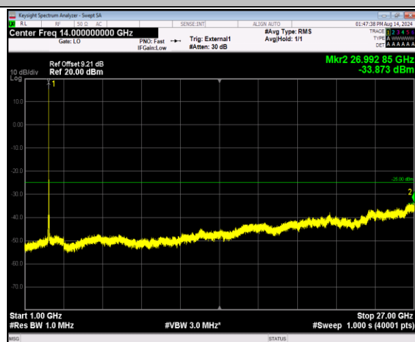
41-41-20MHz-5MHz-16QAM-16QAM-40715-40832-1RB#0- 0RB#0-1000-27000MHz-PASS
