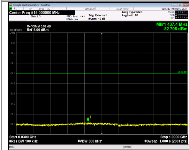
41-41-20MHz-20MHz-64QAM-64QAM-40340-40538-1RB #0-0RB#0-30~1000MHz-PASS
