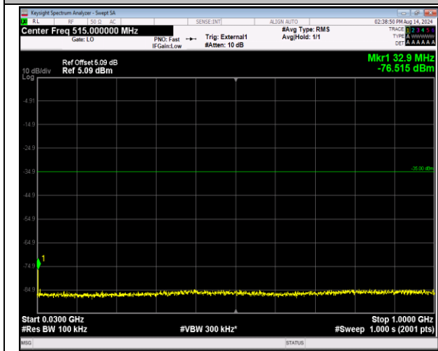
41-41-20MHz-20MHz-QPSK-QPSK-40340-40538-1RB#0 -1RB#99-30~1000MHz-PASS
