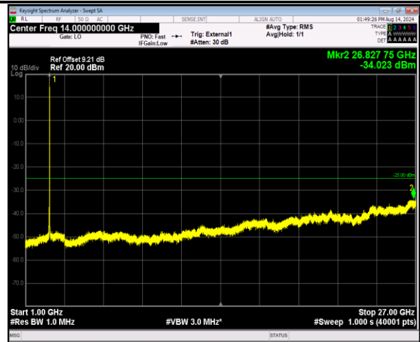
41-41-20MHz-5MHz-16QAM-16QAM-40715-40832-1RB#99 -ORB#0-1000~27000MHz-PASS
