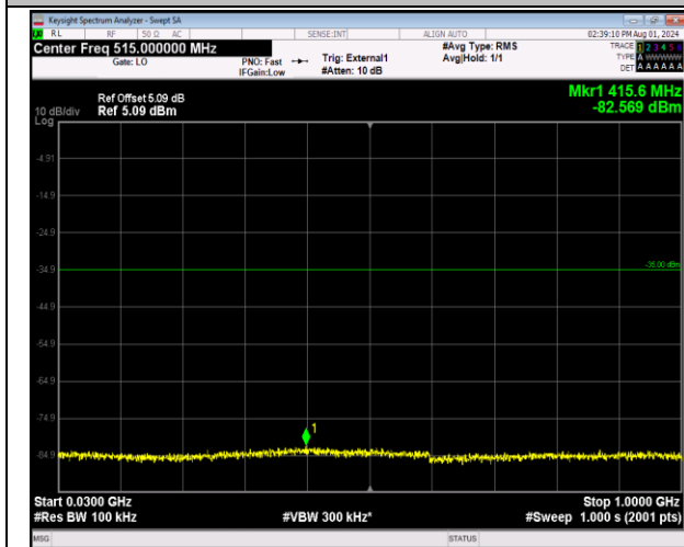
41-41-20MHz-5MHz-64QAM-64QAM-40340-40457-1RB# 0-ORB#0-30~1000MHz-PASS
