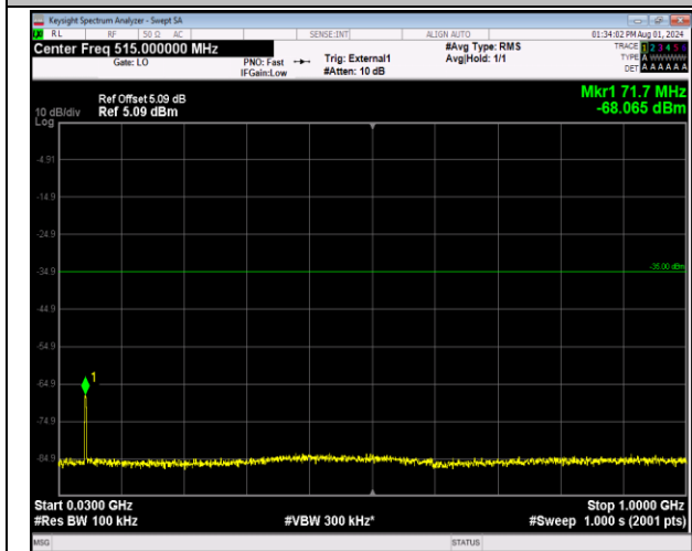
41-41-5MHz-20MHz-64QAM-64QAM-41023-41140-25RB #0-100RB#0-30-1000MHz-PASS
