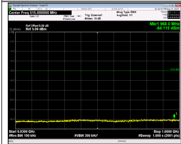
41-41-20MHz-5MHz-QPSK-QPSK-40340-40457-1RB#0-01RB#24-30~1000MHz-PASS
