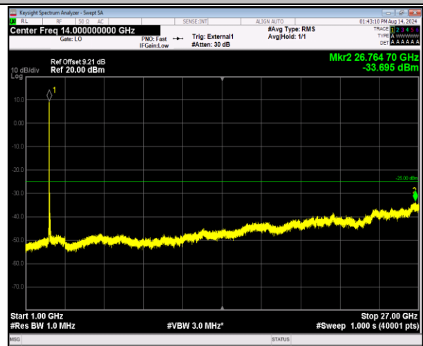
41-41-20MHz-5MHz-QPSK-QPSK-40340-40457-1RB#0-01RB#24-1000~27000MHz-PASS
