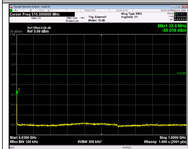
41-41-20MHz-5MHz-16QAM-16QAM-40715-40832-1RB# 0-0RB#0-30-1000MHz-PASS
