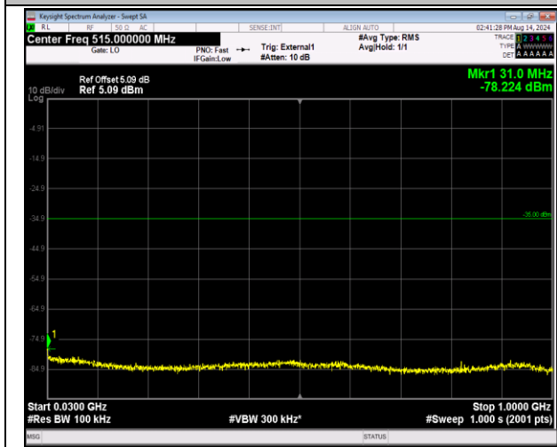
41-41-20MHz-20MHz-16QAM-16QAM-40340-40538-100RB RB#0-100RB#0-30~1000MHz-PASS
