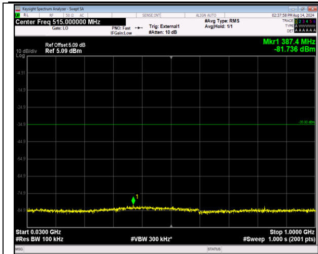
41-41-20MHz-20MHz-16QAM-16QAM-40340-40538-1RB #99-0RB#0-30~1000MHz-PASS
