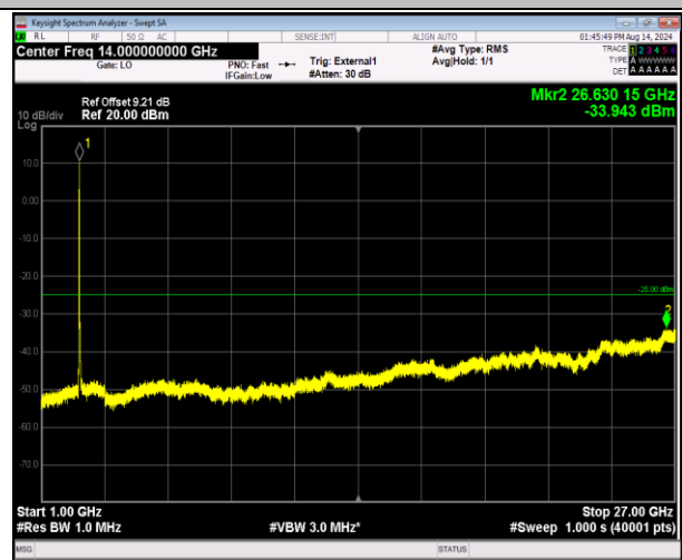
41-41-20MHz-5MHz-16QAM-16QAM-40340-40457-100RB# 0-25RB#0-1000~27000MHz-PASS
