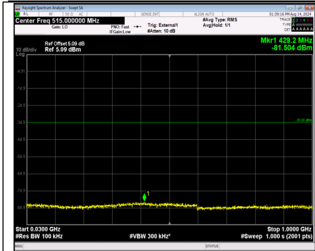
41-41-20MHz-5MHz-QPSK-QPSK-40340-40457-1RB#0-0RB#0-30~1000MHz-PASS
