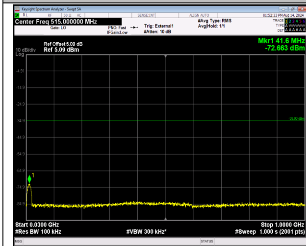
41-41-20MHz-5MHz-16QAM-16QAM-40715-40832-100R B#0-25RB#0-30~1000MHz-PASS
