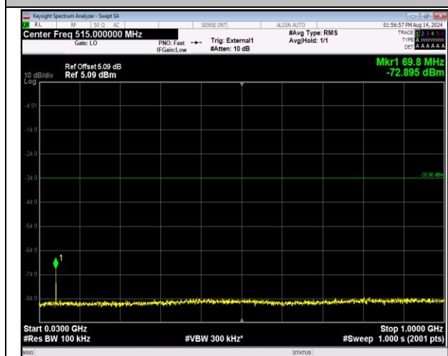
41-41-20MHz-5MHz-QPSK-QPSK-41090-41207-1RB#0-0RB#24-30~1000MHz-PASS
