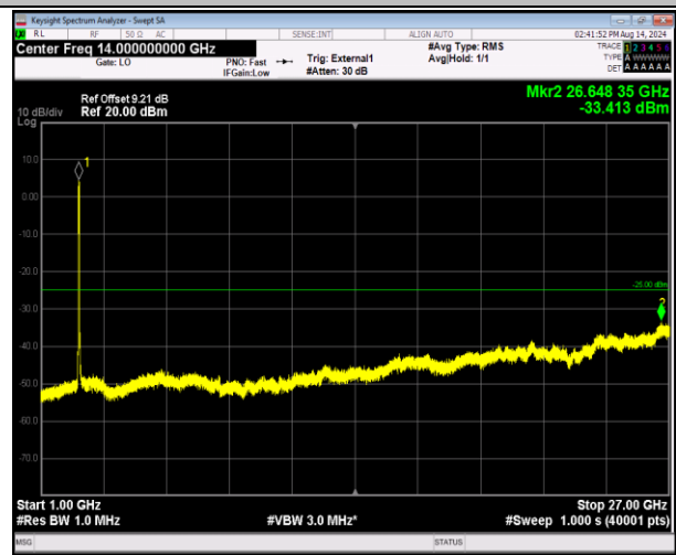
41-41-20MHz-20MHz-16QAM-16QAM-40340-40538-100RB #0-100RB#0-1000~27000MHz-PASS
