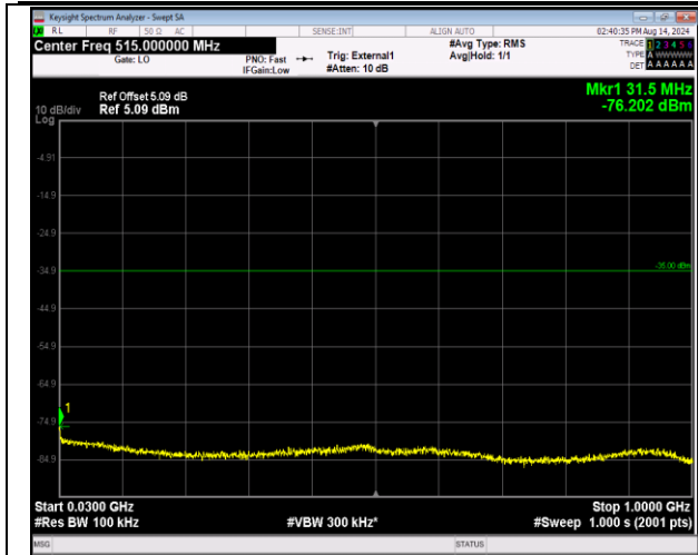
41-41-20MHz-20MHz-QPSK-QPSK-40340-40538-100RB #0-100RB#0-30~1000MHz-PASS
