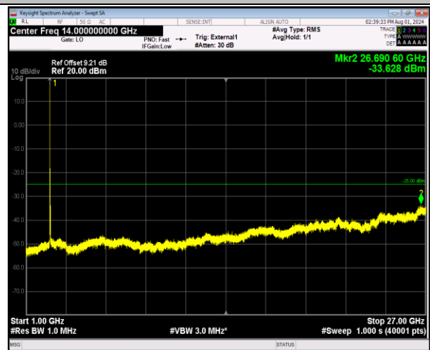
41-41-20MHz-5MHz-64QAM-64QAM-40340-40457-1RB#0- ORB#0-1000~27000MHz-PASS
