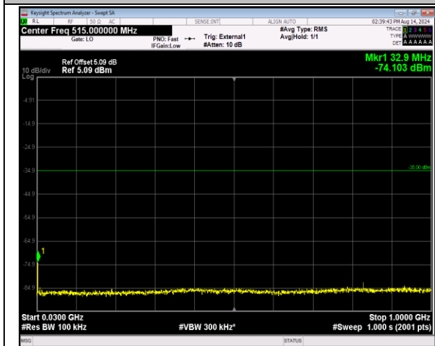
41-41-20MHz-20MHz-16QAM-16QAM-40340-40538-1RB #0-1RB#99-30~1000MHz-PASS
