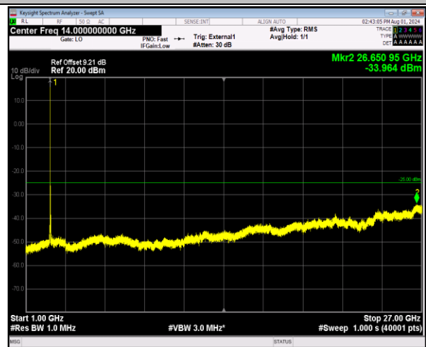
41-41-20MHz-5MHz-64QAM-64QAM-40715-40832-1RB#0- ORB#0-1000~27000MHz-PASS
