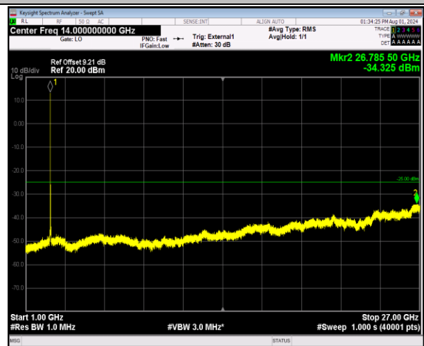
41-41-5MHz-20MHz-64QAM-64QAM-41023-41140-25RB#0 -100RB#0-1000-27000MHz-PASS
