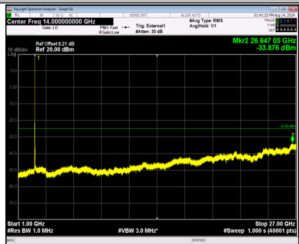
41-41-20MHz-5MHz-QPSK-QPSK-40340-40457-1RB#99-0RB#0-1000~27000MHz-PASS
