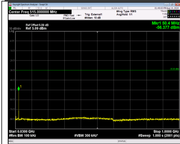
41-41-20MHz-5MHz-16QAM-16QAM-40715-40832-1RB# 99-ORB#0-30~1000MHz-PASS
