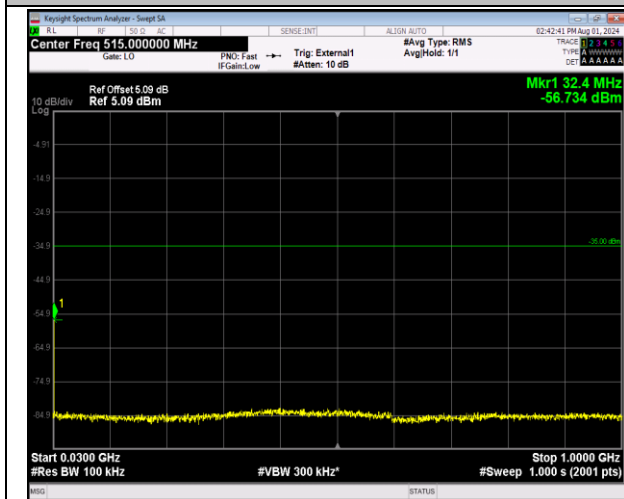
41-41-20MHz-5MHz-64QAM-64QAM-40715-40832-1RB# 0-ORB#0-30~1000MHz-PASS
