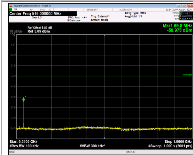
41-41-20MHz-5MHz-16QAM-16QAM-41090-41207-1RB# 0-0RB#0-30-1000MHz-PASS
