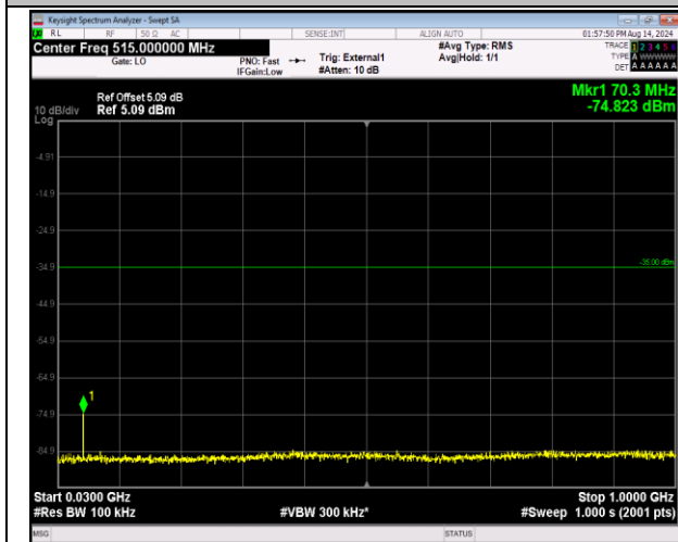
41-41-20MHz-5MHz-16QAM-16QAM-41090-41207-1RB# 0-1RB#24-30-1000MHz-PASS
