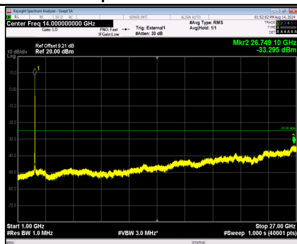
41-41-20MHz-5MHz-QPSK-QPSK-40715-40832-100RB#0- 25RB#0-1000-27000MHz-PASS
