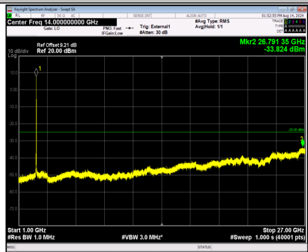
41-41-20MHz-5MHz-16QAM-16QAM-40715-40832-100RB# 0-25RB#0-1000~27000MHz-PASS
