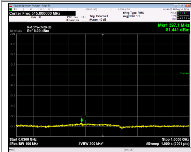
41-41-20MHz-5MHz-QPSK-QPSK-40340-40457-1RB#99-0RB#0-30~1000MHz-PASS
