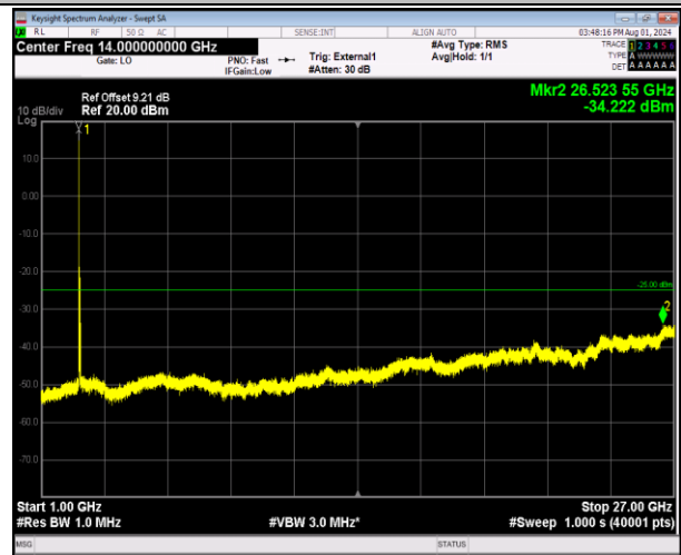
41-41-20MHz-20MHz-64QAM-64QAM-40340-40538-1RB#0 -0RB#0-1000~27000MHz-PASS
