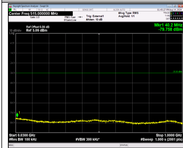
41-41-20MHz-5MHz-16QAM-16QAM-40340-40457-100R B#0-25RB#0-30~1000MHz-PASS
