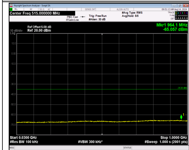
7-7-10MHz-20MHz-QPSK-QPSK-21006-21150-1RB#49-49 ORB#0-30~1000MHz-PASS
