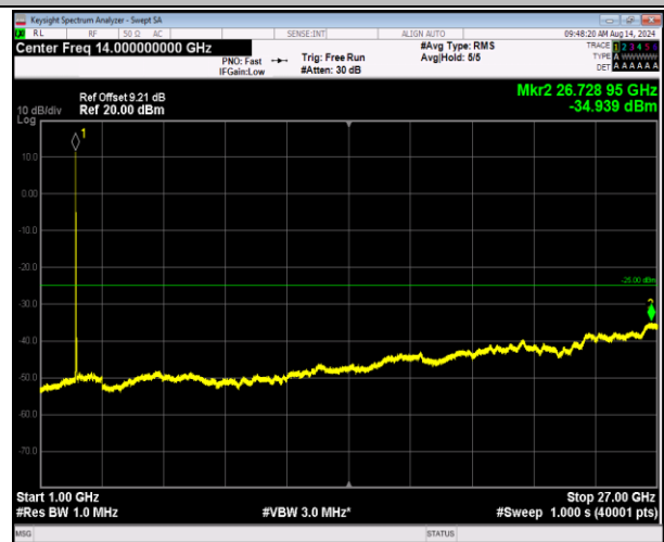
7-7-10MHz-20MHz-16QAM-16QAM-20805-20949-1RB#0-1-99~1000~27000MHz-PASS
