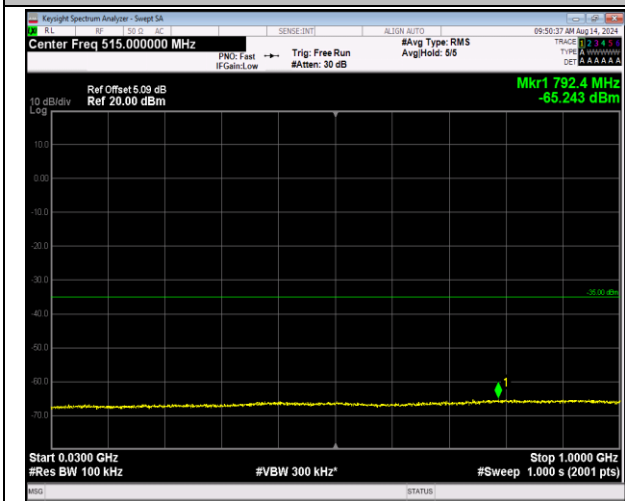
7-7-10MHz-20MHz-16QAM-16QAM-21006-21150-1RB#0-0-30~1000MHz-PASS
