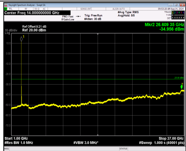
7-7-10MHz-20MHz-16QAM-16QAM-21006-21150-1RB#0-1-99~1000~27000MHz-PASS
