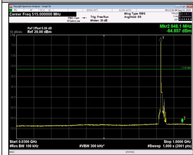
5-5-10MHz-10MHz-16QAM-16QAM-20501-20600-1RB#0-0RB#0-30~1000MHz-PASS
