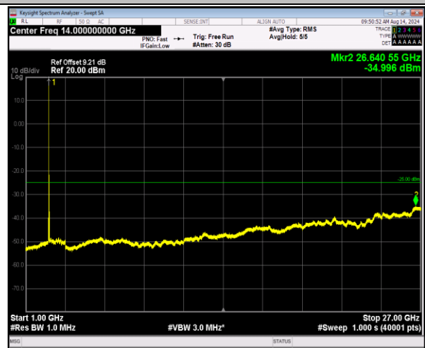
7-7-10MHz-20MHz-16QAM-16QAM-21006-21150-1RB#0-0-1000~27000MHz-PASS
