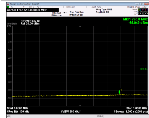
7-7-10MHz-20MHz-16QAM-16QAM-21006-21150-1RB#0-1-99~1000MHz-PASS
