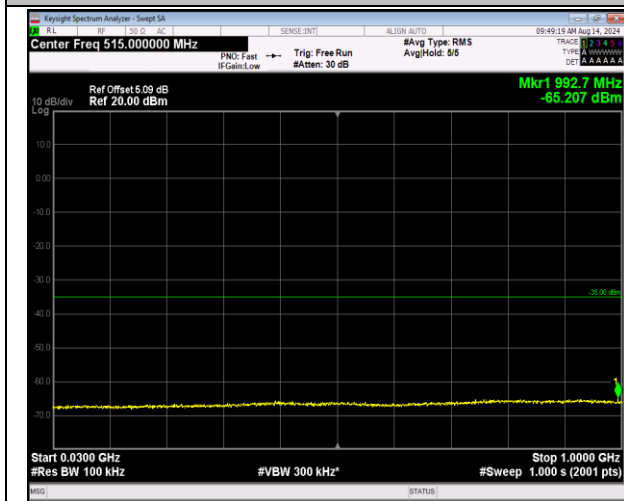
7-7-10MHz-20MHz-16QAM-16QAM-20805-20949-50RB#- 0-100RB#0-30~1000MHz-PASS
