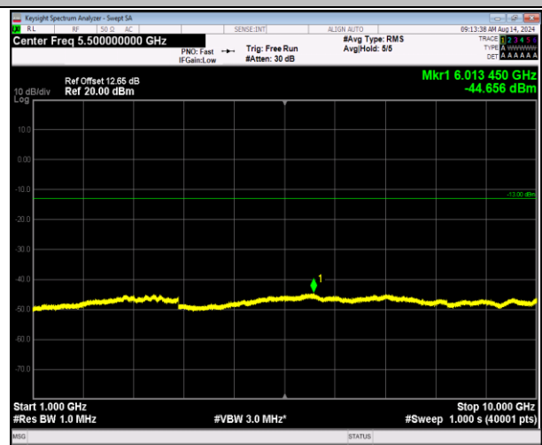
5-5-10MHz-10MHz-16QAM-16QAM-20501-20600-1RB#0-0RB#0-1000~10000MHz-PASS
