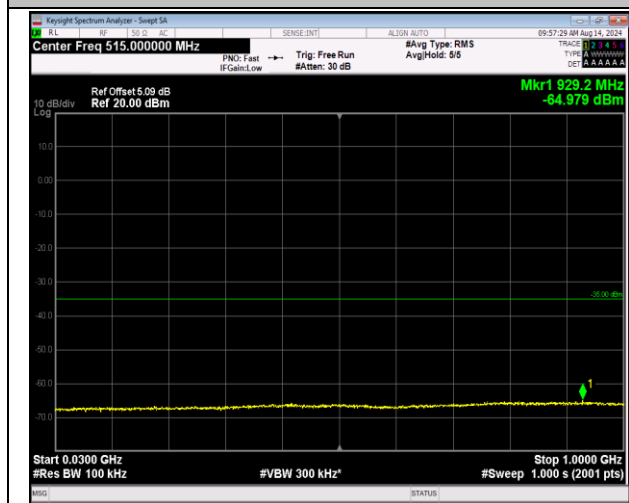
7-7-10MHz-20MHz-QPSK-QPSK-21206-21350-1RB#0-1 RB#99-30~1000MHz-PASS
