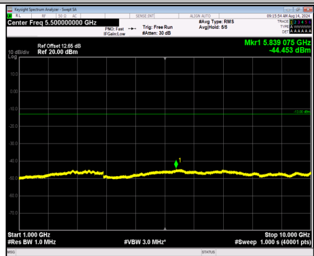
5-5-10MHz-10MHz-16QAM-16QAM-20501-20600-1RB#0-1RB#49-1000~10000MHz-PASS
