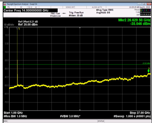
7-7-10MHz-20MHz-64QAM-64QAM-20805-20949-1RB#0-0 RB#0-1000~27000MHz-PASS
