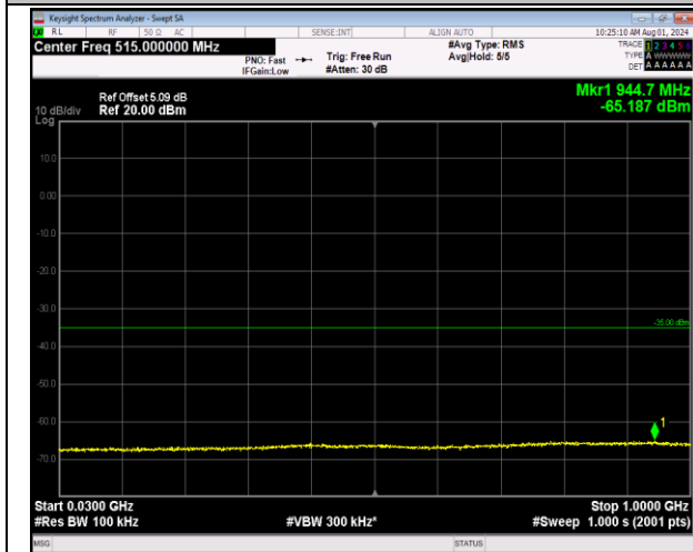
7-7-10MHz-20MHz-64QAM-64QAM-20805-20949-1RB#0- -0RB#0-30~1000MHz-PASS
