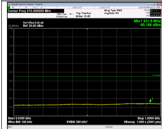
7-7-20MHz-10MHz-QPSK-QPSK-20850-20994-1RB#99-9 ORB#0-30~1000MHz-PASS
