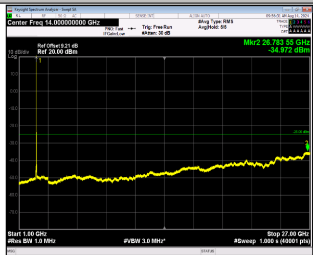
7-7-10MHz-20MHz-QPSK-QPSK-21206-21350-1RB#49-0RB B#0-1000~27000MHz-PASS
