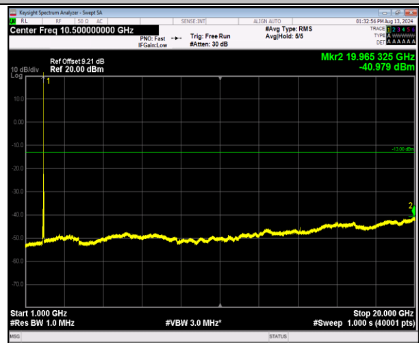
2-2-5MHz-20MHz-16QAM-16QAM-18808-18925-1RB#0-0R B#0-1000~20000MHz-PASS
