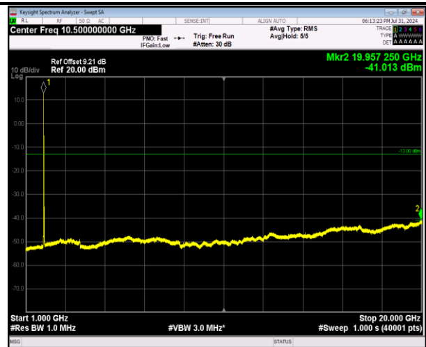
2-2-5MHz-20MHz-64QAM-64QAM-18633-18750-1RB#0-1RB#99-1000~20000MHz-PASS
