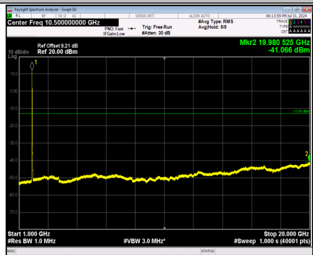
2-2-5MHz-20MHz-64QAM-64QAM-18633-18750-25RB#0-100RB#0-1000~20000MHz-PASS
