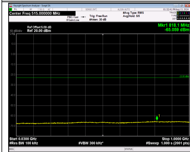
2-2-5MHz-20MHz-16QAM-16QAM-18808-18925-1RB#0-0 0RB#0-30~1000MHz-PASS
