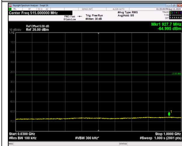
2-2-5MHz-20MHz-16QAM-16QAM-18808-18925-1RB#0-0 1RB#99-30~1000MHz-PASS
