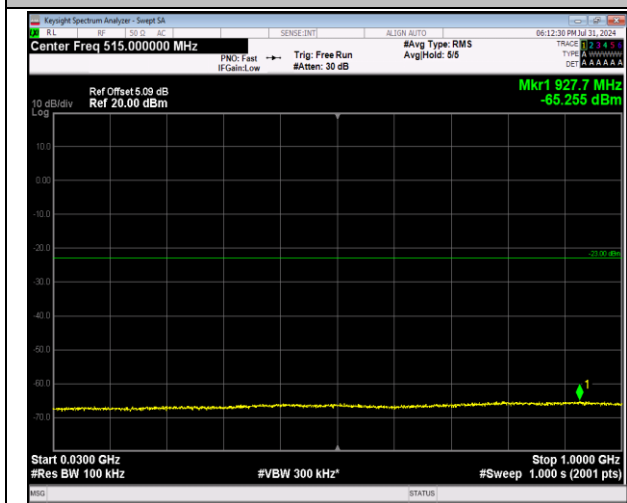
2-2-5MHz-20MHz-64QAM-64QAM-18633-18750-1RB#24-0-0RB#0-30~1000MHz-PASS
