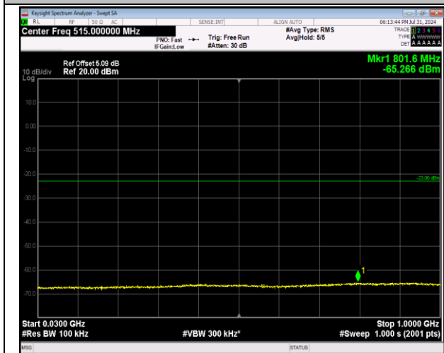
2-2-5MHz-20MHz-64QAM-64QAM-18633-18750-25RB#0-100RB#0-30~1000MHz-PASS
