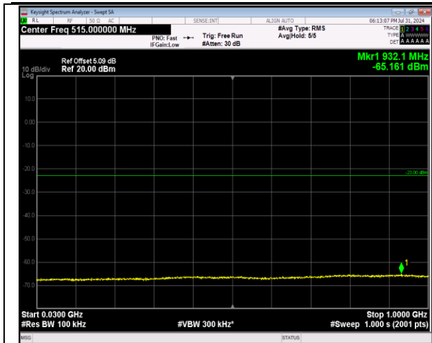
2-2-5MHz-20MHz-64QAM-64QAM-18633-18750-1RB#0-1RB#99-30~1000MHz-PASS
