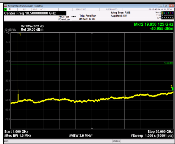
2-2-5MHz-20MHz-64QAM-64QAM-18633-18750-1RB#24-0RB#0-1000~20000MHz-PASS
