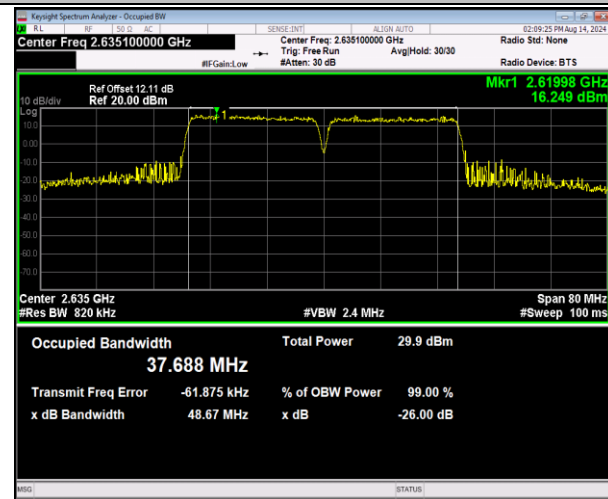
41-41-20MHz-20MHz-16QAM-16QAM-40942-41140-100RB #0-100RB#0-PASS
