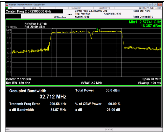
41-41-20MHz-15MHz-16QAM-16QAM-40340-40511-100RB #0-75RB#0-PASS
