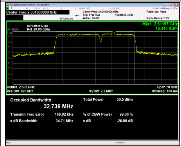
41-41-20MHz-15MHz-QPSK-QPSK-40666-40837-100RB #0-75RB#0-PASS
