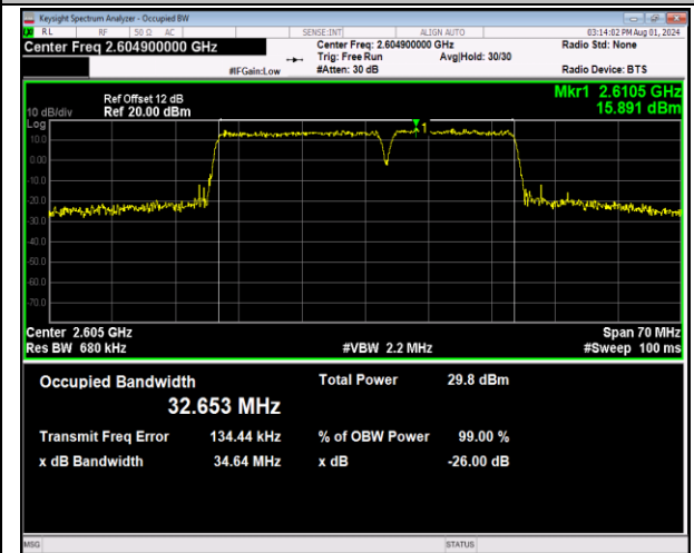
41-41-20MHz-15MHz-64QAM-64QAM-40666-40837-100RB #0-75RB#0-PASS
