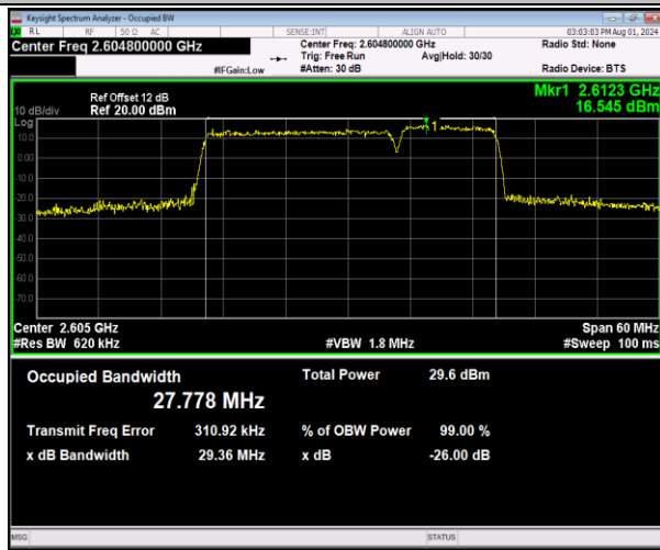
41-41-20MHz-10MHz-64QAM-64QAM-40691-40835-100RB #0-50RB#0-PASS
