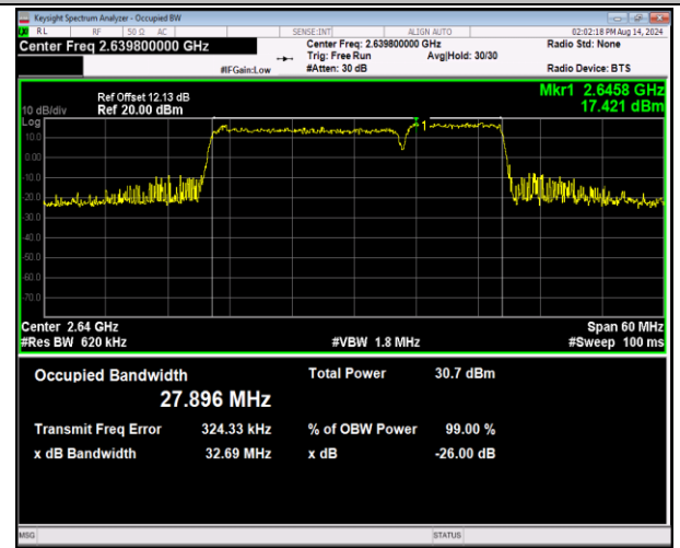
41-41-20MHz-10MHz-QPSK-QPSK-41041-41185-100RB #0-50RB#0-PASS
