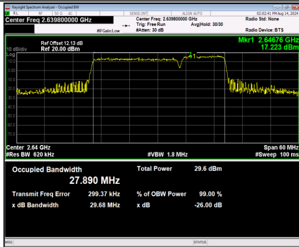
41-41-20MHz-10MHz-16QAM-16QAM-41041-41185-100RB #0-50RB#0-PASS
