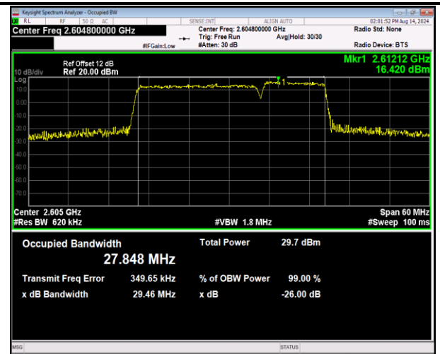
41-41-20MHz-10MHz-16QAM-16QAM-40691-40835-100RB #0-50RB#0-PASS
