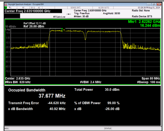
41-41-20MHz-20MHz-64QAM-64QAM-40942-41140-100RB #0-100RB#0-PASS
