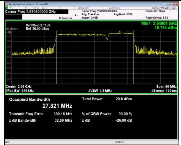
41-41-20MHz-10MHz-64QAM-64QAM-41041-41185-100RB #0-50RB#0-PASS
