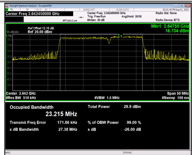
41-41-15MHz-10MHz-64QAM-64QAM-41067-41187-75RB#0-50RB#0-PASS
