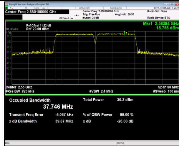
7-7-20MHz-20MHz-16QAM-16QAM-21152-21350-100RB#0-100RB#0-PASS
