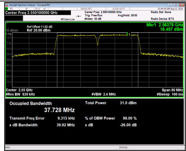
7-7-20MHz-20MHz-QPSK-QPSK-21152-21350-100RB#0-100RB#0-PASS
