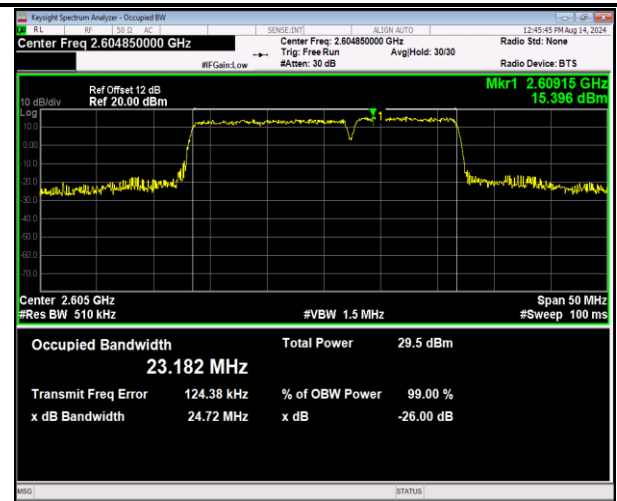
41-41-15MHz-10MHz-16QAM-16QAM-40691-40811-75RB#0-50RB#0-PASS
