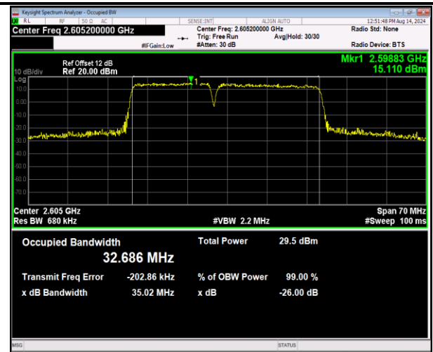
41-41-15MHz-20MHz-16QAM-16QAM-40644-40815-75RB#0-100RB#0-PASS
