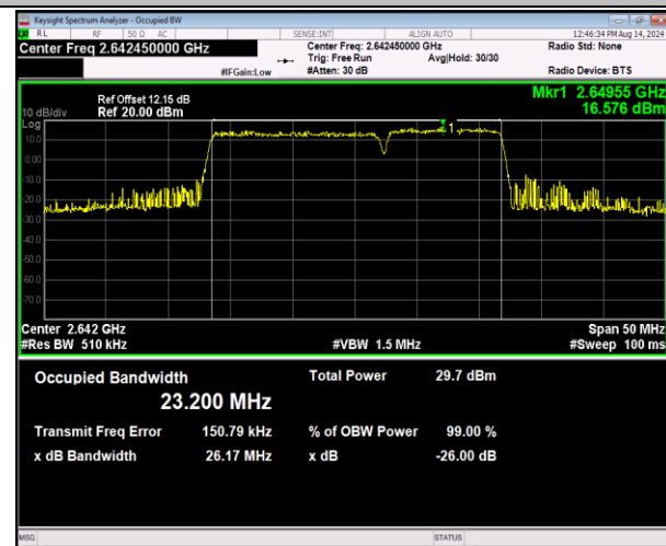
41-41-15MHz-10MHz-16QAM-16QAM-41067-41187-75RB#0-50RB#0-PASS
