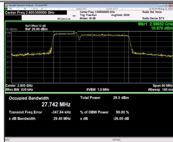
41-41-10MHz-20MHz-16QAM-16QAM-40646-40790-50RB#0-100RB#0-PASS
