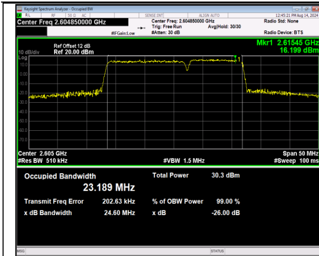
41-41-15MHz-10MHz-QPSK-QPSK-40691-40811-75RB#0-50RB#0-PASS
