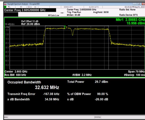
41-41-15MHz-20MHz-64QAM-64QAM-40644-40815-75RB#0-100RB#0-PASS
