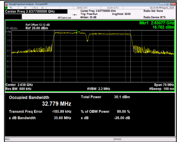
41-41-15MHz-20MHz-64QAM-64QAM-40969-41140-75RB#0-100RB#0-PASS
