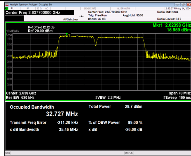
41-41-15MHz-20MHz-16QAM-16QAM-40969-41140-75RB#0-100RB#0-PASS
