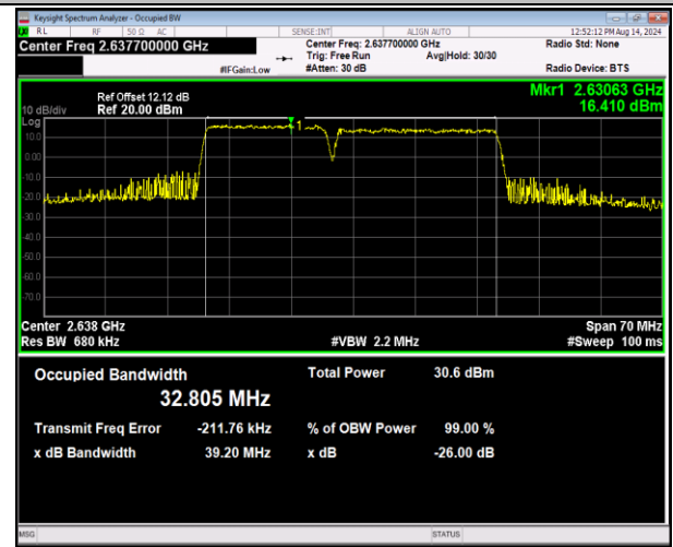
41-41-15MHz-20MHz-QPSK-QPSK-40969-41140-75RB#0-100RB#0-PASS
