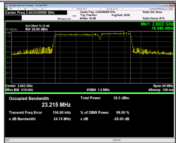
41-41-15MHz-10MHz-QPSK-QPSK-41067-41187-75RB#0-50RB#0-PASS
