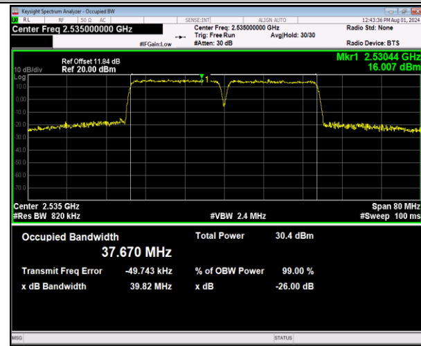
7-7-20MHz-20MHz-64QAM-64QAM-21001-21199-100RB#0-100RB#0-PASS
