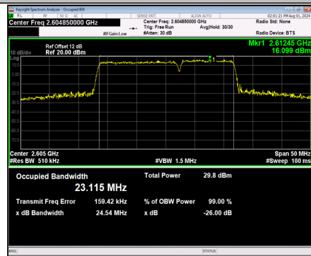
41-41-15MHz-10MHz-64QAM-64QAM-40691-40811-75RB#0-50RB#0-PASS
