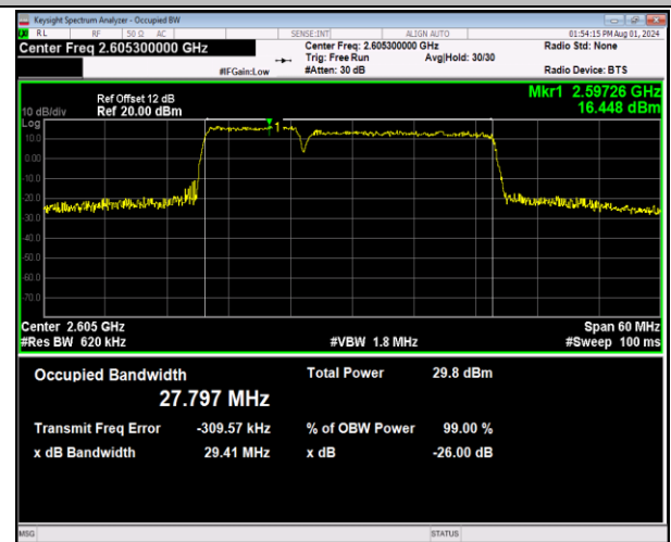
41-41-10MHz-20MHz-64QAM-64QAM-40646-40790-50RB#0-100RB#0-PASS
