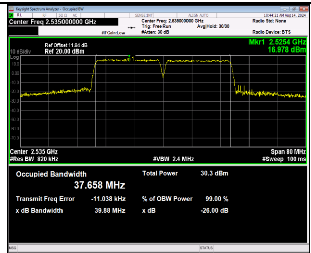
7-7-20MHz-20MHz-16QAM-16QAM-21001-21199-100RB#0-100RB#0-PASS
