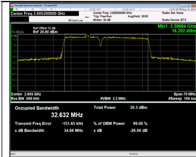
41-41-15MHz-20MHz-QPSK-QPSK-40644-40815-75RB#0-100RB#0-PASS
