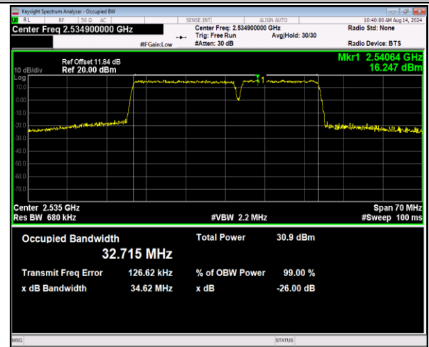
7-7-20MHz-15MHz-QPSK-QPSK-21026-21197-100RB#0-75RB#0-PASS
