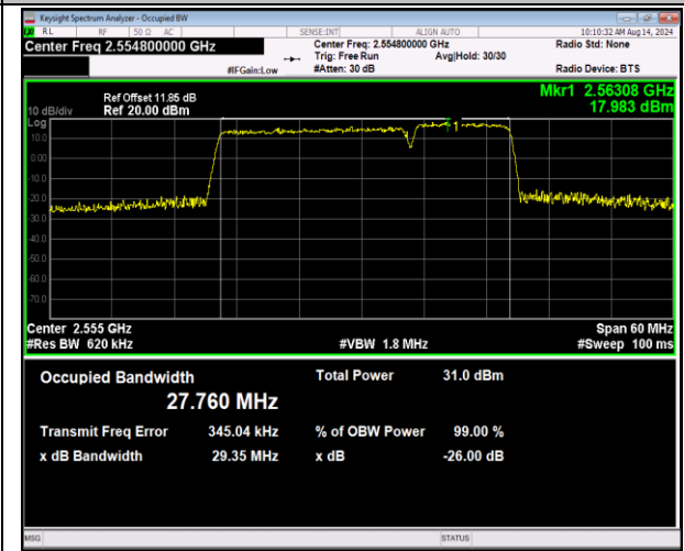
7-7-20MHz-10MHz-QPSK-QPSK-21251-21395-100RB#0-50RB#0-PASS
