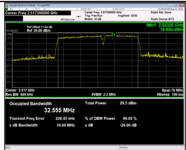
7-7-20MHz-15MHz-16QAM-16QAM-20850-21021-100RB#0-75RB#0-PASS
