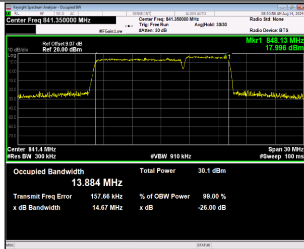
5-5-10MHz-5MHz-16QAM-16QAM-20550-20622-50RB#0- 25RB#0-PASS
