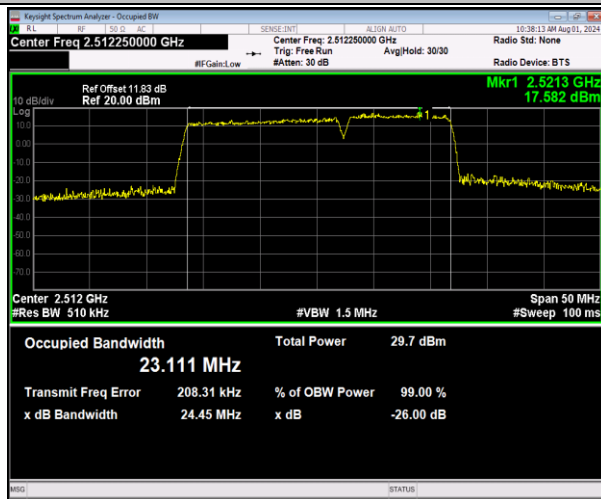
7-7-15MHz-10MHz-64QAM-64QAM-20825-20945-75RB# 0-50RB#0-PASS
