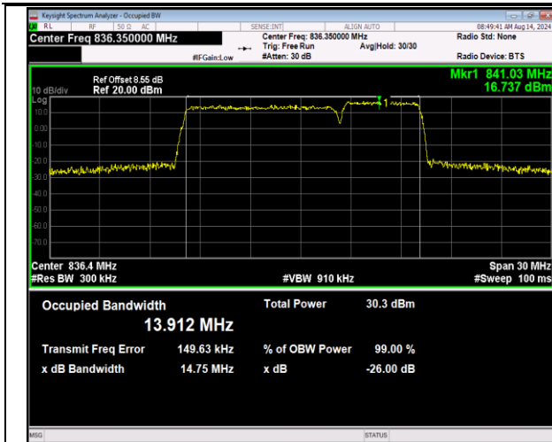
5-5-10MHz-5MHz-QPSK-QPSK-20500-20572-50RB#0-25 RB#0-PASS
