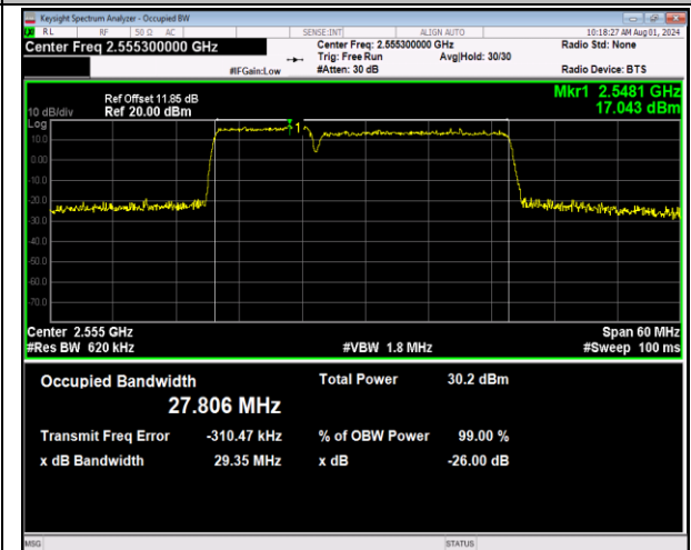
7-7-10MHz-20MHz-64QAM-64QAM-21206-21350-50RB #0-100RB#0-PASS
