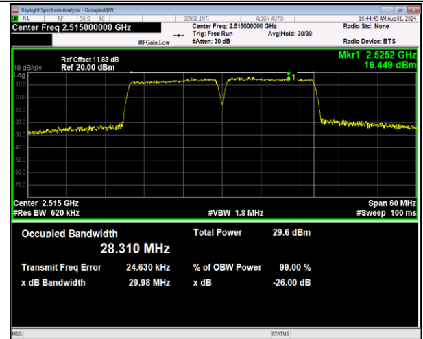
7-7-15MHz-15MHz-64QAM-64QAM-20825-20975-75RB#0-75RB#0-PASS
