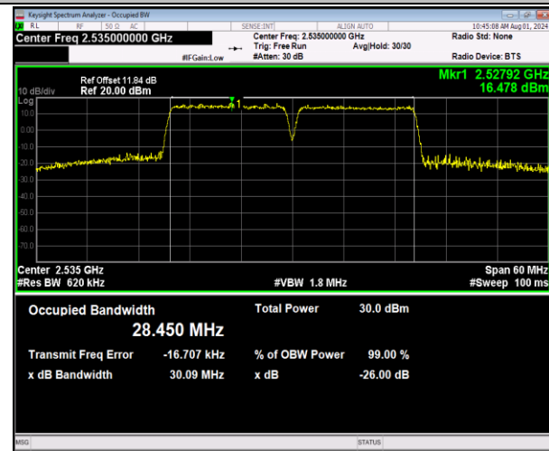
7-7-15MHz-15MHz-64QAM-64QAM-21025-21175-75RB#0-75RB#0-PASS
