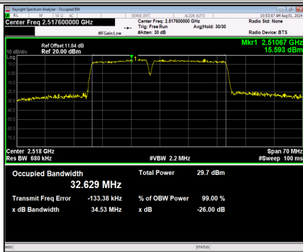
7-7-15MHz-20MHz-64QAM-64QAM-20828-20999-75RB# 0-100RB#0-PASS
