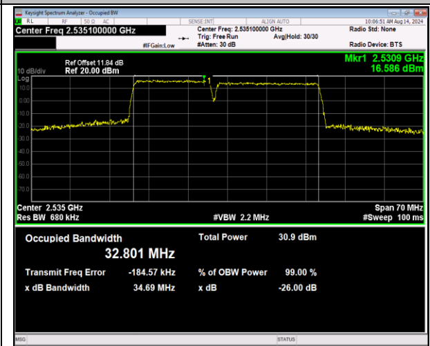
7-7-15MHz-20MHz-QPSK-QPSK-21003-21174-75RB#0- 100RB#0-PASS
