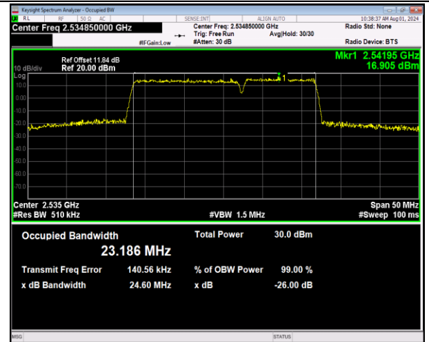
7-7-15MHz-10MHz-64QAM-64QAM-21051-21171-75RB #0-50RB#0-PASS
