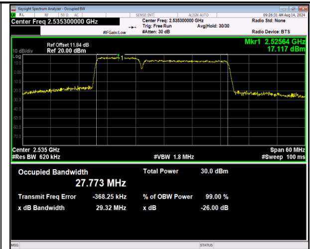
7-7-10MHz-20MHz-16QAM-16QAM-21006-21150-50RB #0-100RB#0-PASS
