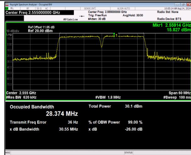
7-7-15MHz-15MHz-16QAM-16QAM-21225-21375-75RB#0-75RB#0-PASS
