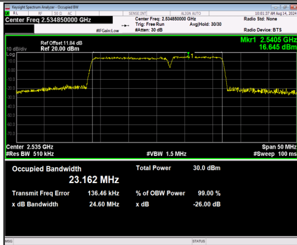
7-7-15MHz-10MHz-16QAM-16QAM-21051-21171-75RB# 0-50RB#0-PASS
