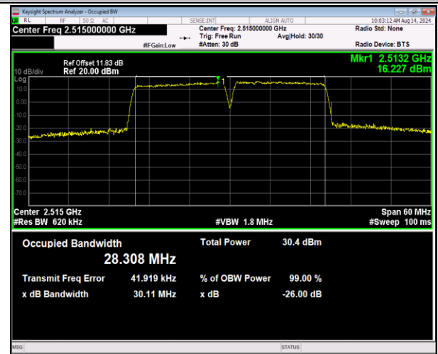
7-7-15MHz-15MHz-QPSK-QPSK-20825-20975-75RB#0-75RB#0-PASS
