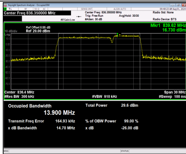
5-5-10MHz-5MHz-64QAM-64QAM-20500-20572-50RB#0- 25RB#0-PASS
