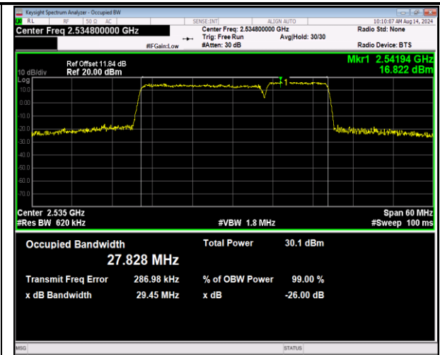
7-7-20MHz-10MHz-16QAM-16QAM-21051-21195-100RB#0-50RB#0-PASS
