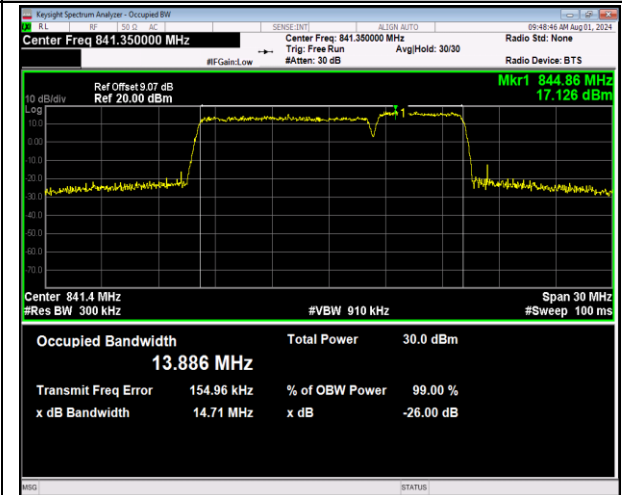
5-5-10MHz-5MHz-64QAM-64QAM-20550-20622-50RB# 0-25RB#0-PASS
