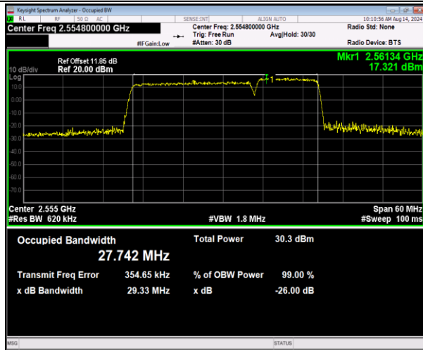
7-7-20MHz-10MHz-16QAM-16QAM-21251-21395-100RB#0-50RB#0-PASS
