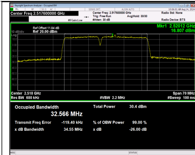
7-7-15MHz-20MHz-QPSK-QPSK-20828-20999-75RB#0-1 00RB#0-PASS
