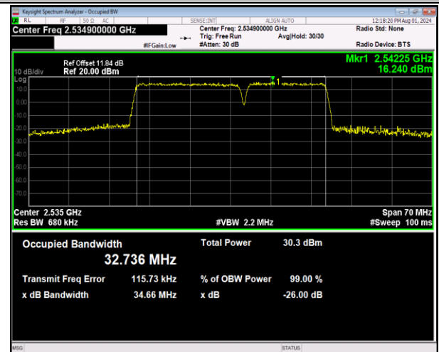
7-7-20MHz-15MHz-64QAM-64QAM-21026-21197-100RB#0-75RB#0-PASS
