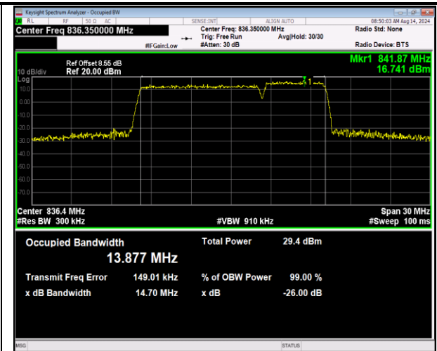
5-5-10MHz-5MHz-16QAM-16QAM-20500-20572-50RB# 0-25RB#0-PASS
