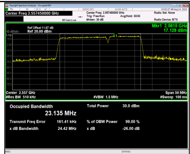
7-7-15MHz-10MHz-16QAM-16QAM-21277-21397-75RB#0-50RB#0-PASS
