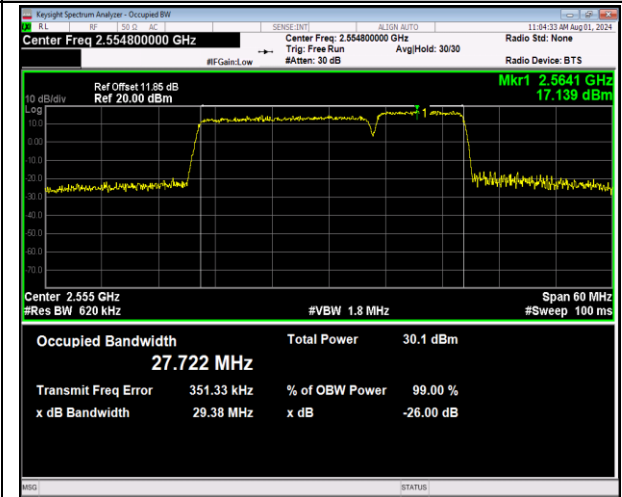
7-7-20MHz-10MHz-64QAM-64QAM-21251-21395-100RB#0-50RB#0-PASS
