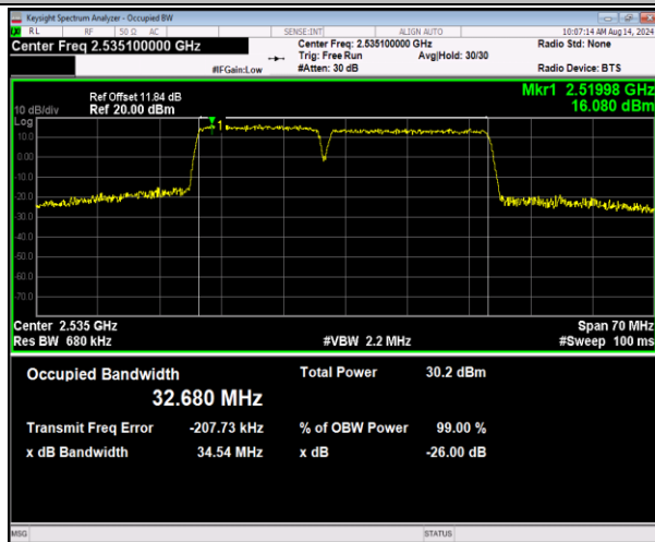
7-7-15MHz-20MHz-16QAM-16QAM-21003-21174-75RB# 0-100RB#0-PASS
