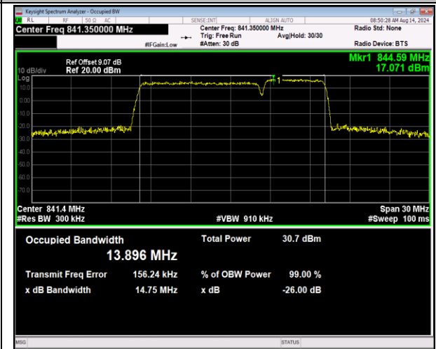
5-5-10MHz-5MHz-QPSK-QPSK-20550-20622-50RB#0-2 5RB#0-PASS
