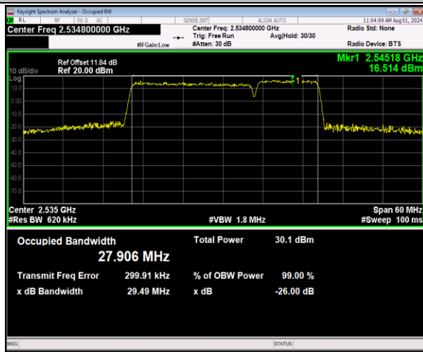
7-7-20MHz-10MHz-64QAM-64QAM-21051-21195-100RB#0-50RB#0-PASS
