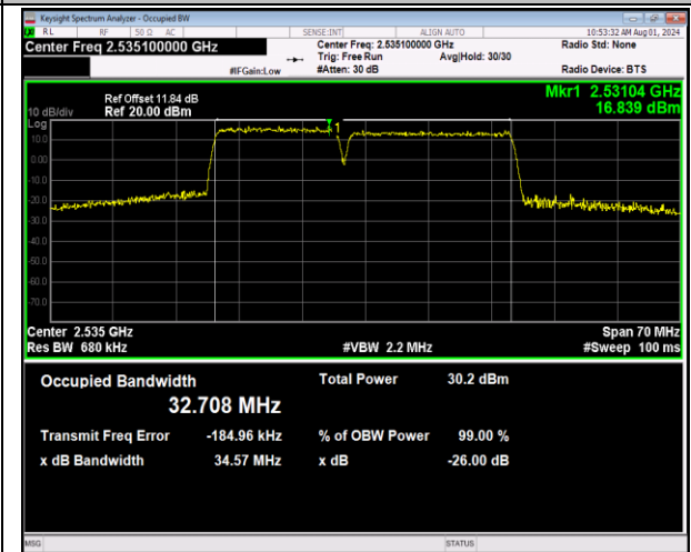
7-7-15MHz-20MHz-64QAM-64QAM-21003-21174-75RB #0-100RB#0-PASS
