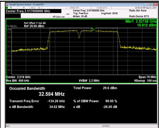
7-7-15MHz-20MHz-16QAM-16QAM-20828-20999-75RB #0-100RB#0-PASS
