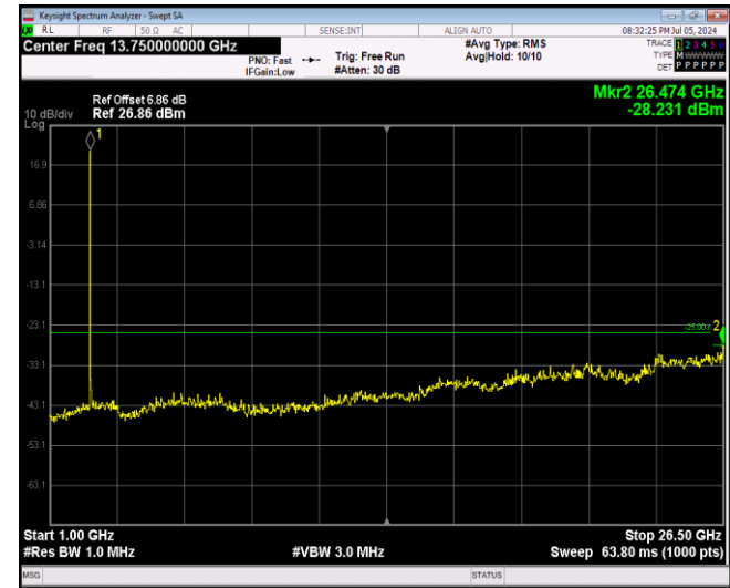
Band41-5MHz-16QAM-40640-1RB#0-Range2:1000~26500MHz
