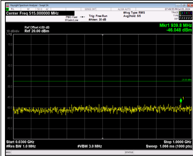
Band7-5MHz-16QAM-21425-1RB#0-Range1:30~100 OMHz
