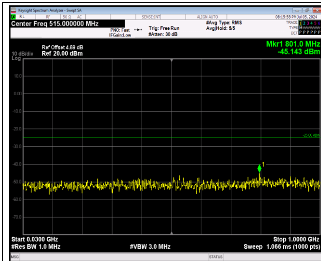
Band7-20MHz-16QAM-21350-1RB#0-Range1:30~1000MHz
