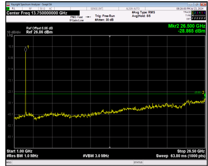
Band7-20MHz-64QAM-21350-1RB#0-Range2:1000~26500MHz
