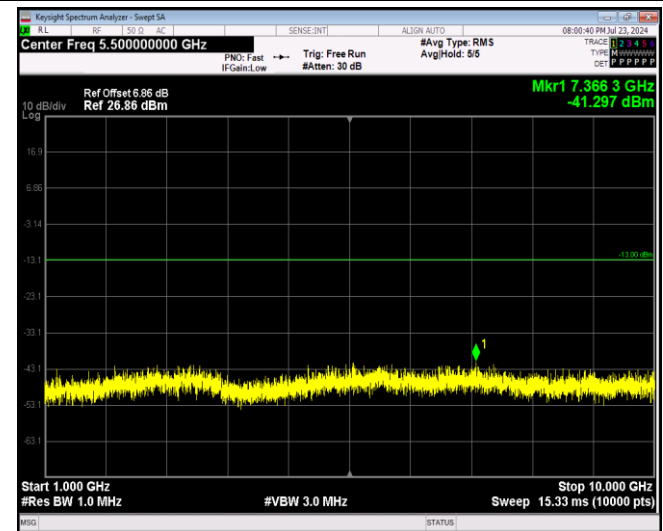
Band5-10MHz-64QAM-20525-1RB#0-Range2:1000~10 00MHz
