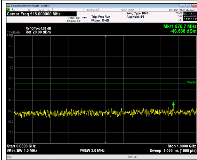
Band7-20MHz-64QAM-20850-1RB#0-Range1:30~1000MHz
