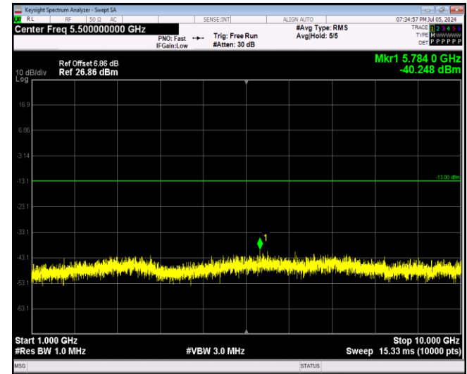
Band5-10MHz-64QAM-20450-1RB#0-Range2:1000~10 00MHz
