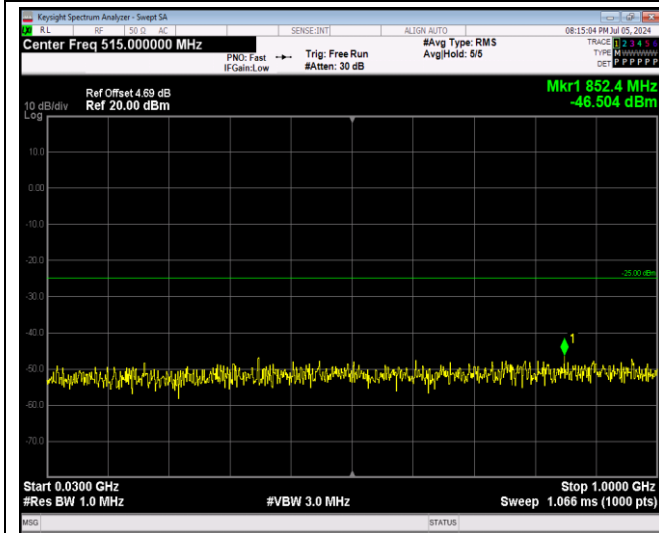
Band7-20MHz-QPSK-21100-1RB#0-Range1:30~100 OMHz
