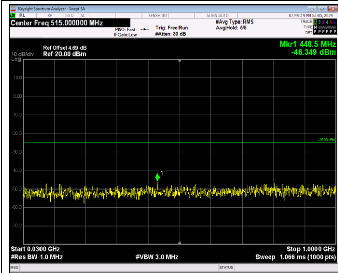
Band7-5MHz-16QAM-21425-1RB#0-Range1:30~100 OMHz
