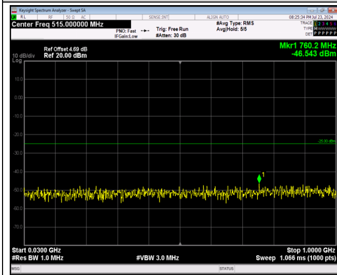
Band7-20MHz-64QAM-20850-1RB#0-Range1:30~1000MHz
