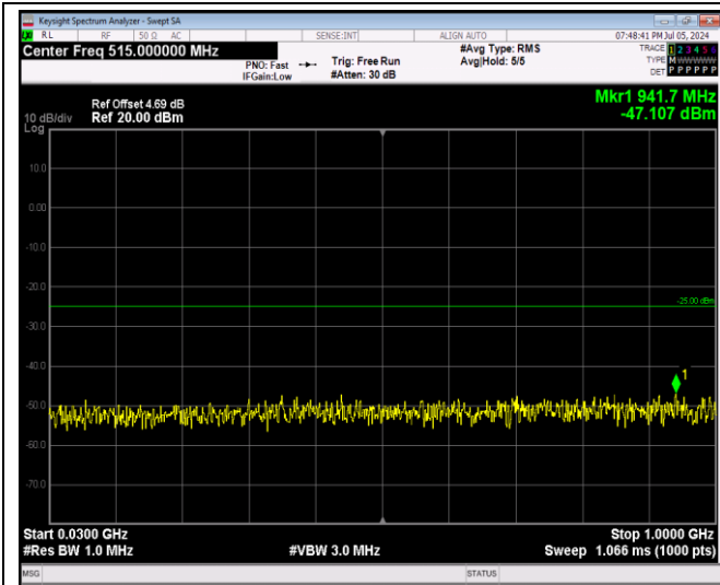
Band7-5MHz-16QAM-21100-1RB#0-Range1:30~100 OMHz
