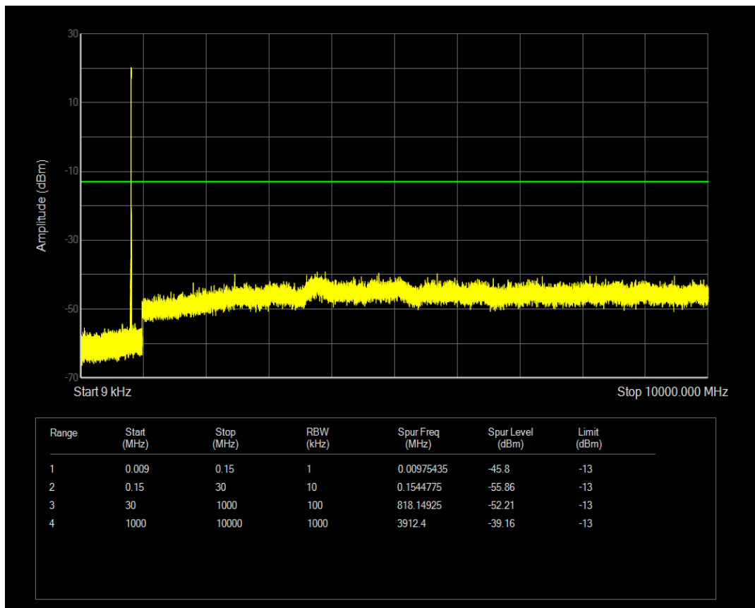
Band5 QAM64 BW=5MHz Channel=20425 RB Size=25 Position=#0
