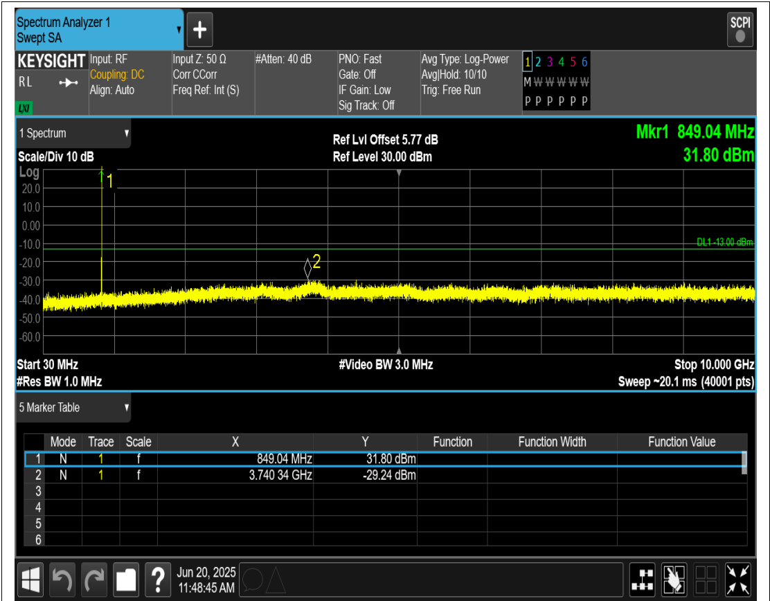
GSM850 Channel=251
