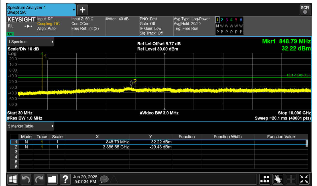
GPRS850 Channel=251
