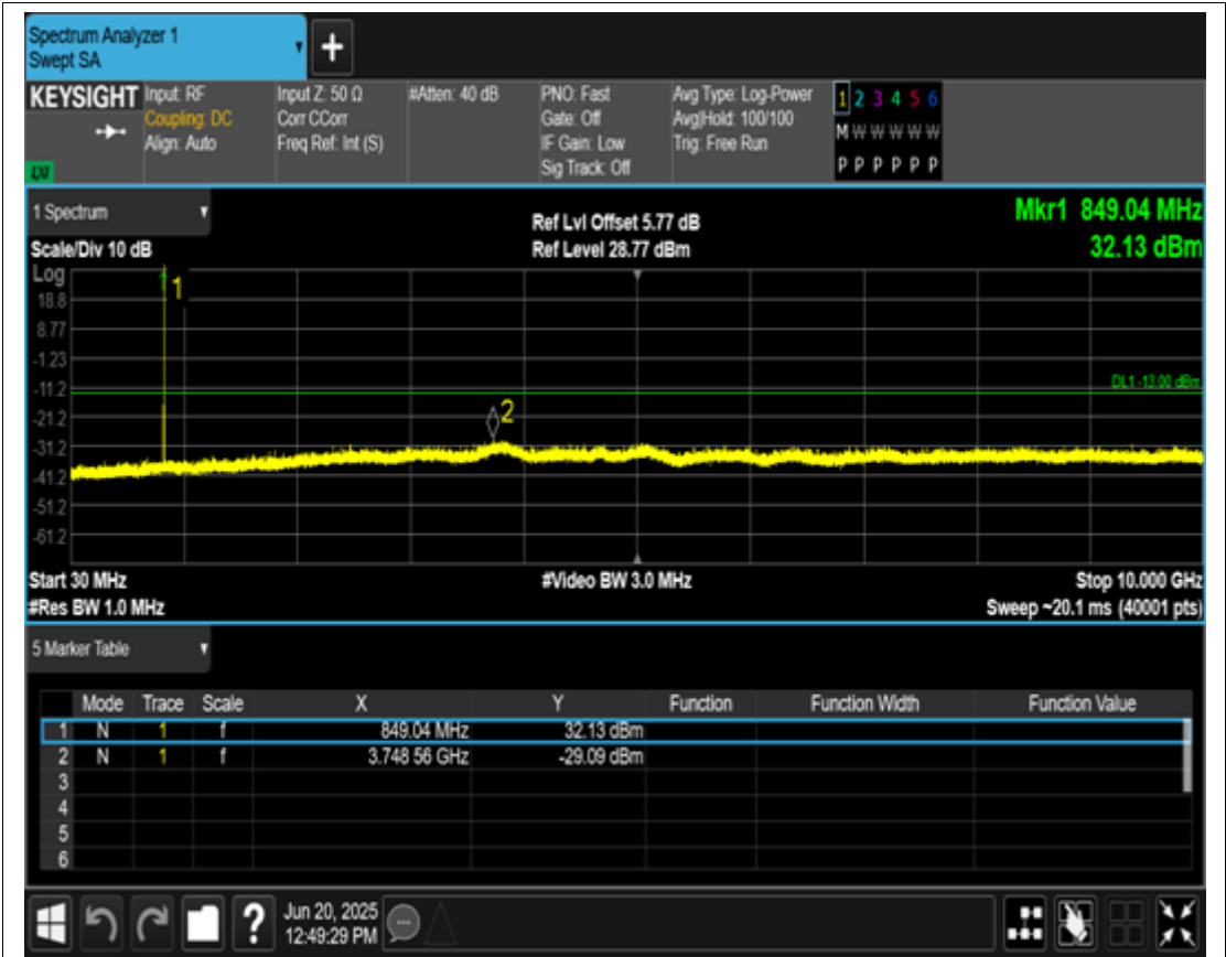
EGPRS850 Channel=251
