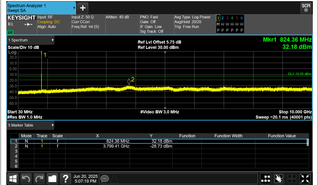
GPRS850 Channel=128
