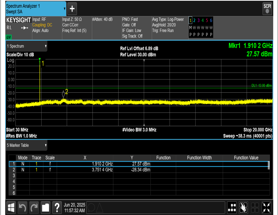
GSM1900 Channel=810
