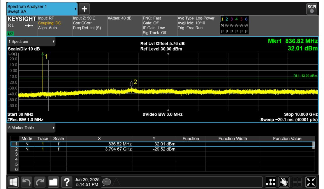
GSM850 Channel=190
