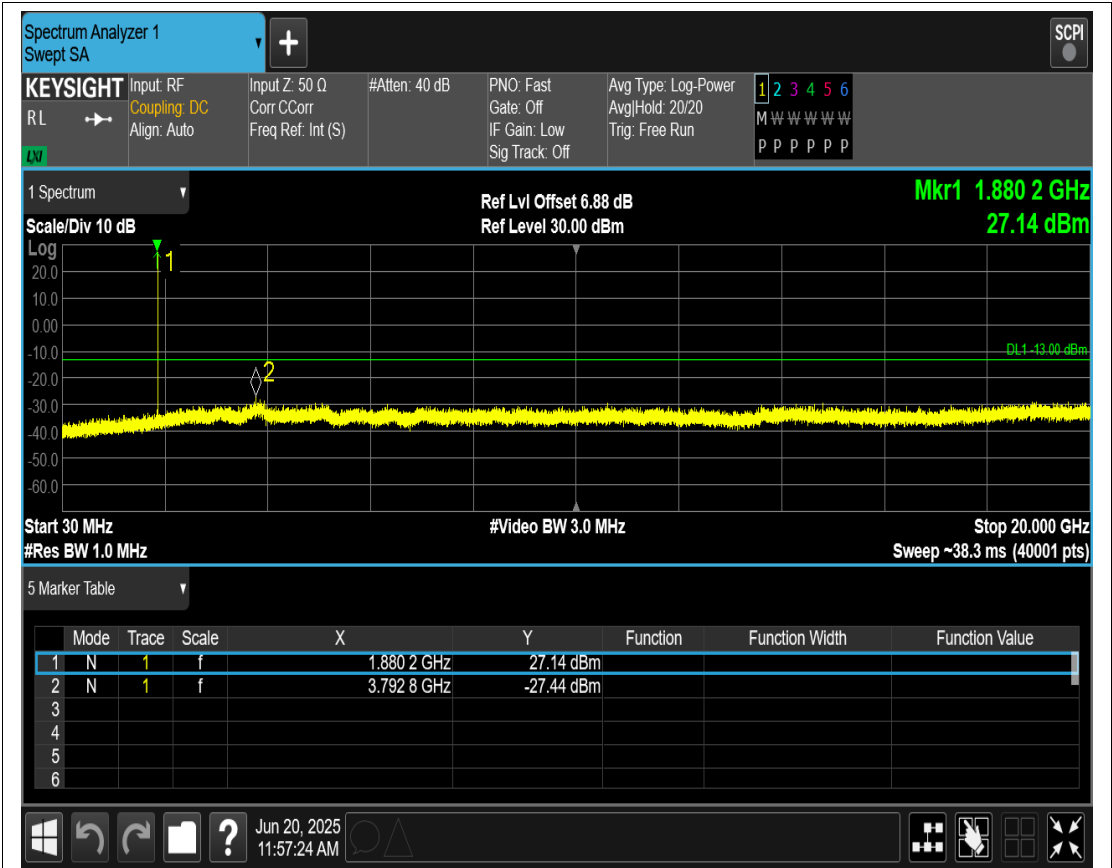
GSM1900 Channel=661
