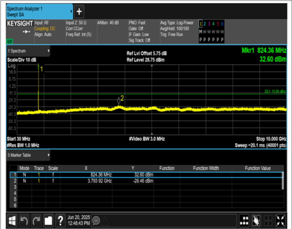
EGPRS850 Channel=128
