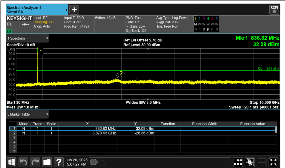
GPRS850 Channel=190
