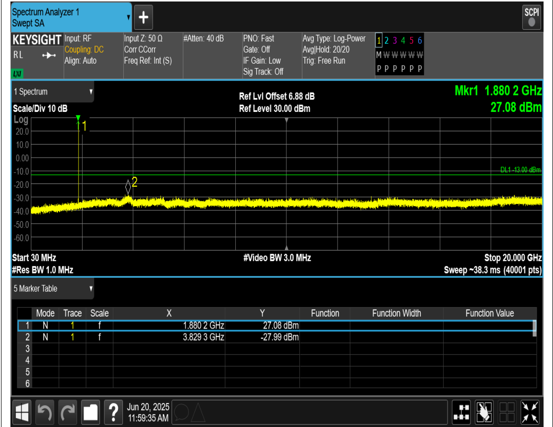
GPRS1900 Channel=661
