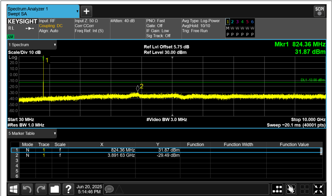
GSM850 Channel=128
