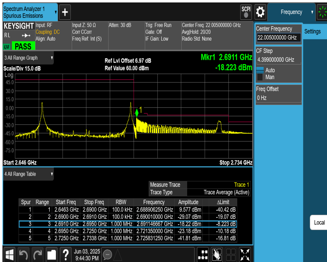
41C 16QAM PCC BW=15MHz Ch=41365 RB=1@0,SCC BW=15MHz Ch=41515 RB=1@74
