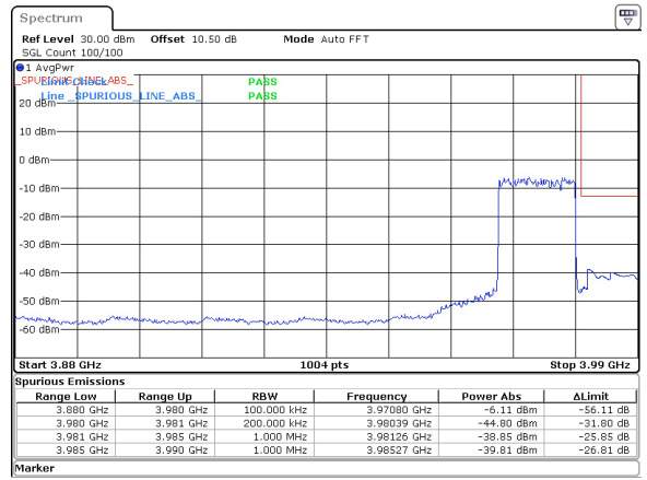
15MHz_15kHz_3972.5MHz_DFT-s-OFDM QPSK_RB75@0 -38.85 dBm
