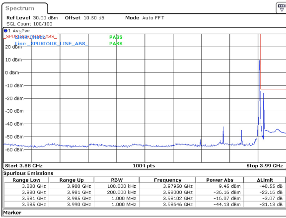
15MHz_15kHz_3972.5MHz_DFT-s-OFDM QPSK_RB1@78 -16.07 dBm
