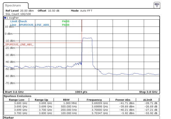
15MHz_30kHz_3707.5MHz_DFT-s-OFDM QPSK_RB36@0 -39.69 dBm
