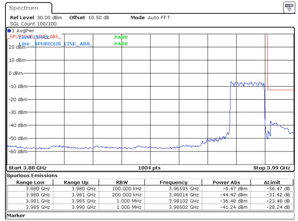
15MHz_30kHz_3972.5MHz_DFT-s-OFDM QPSK_RB36@0 -36.48 dBm
