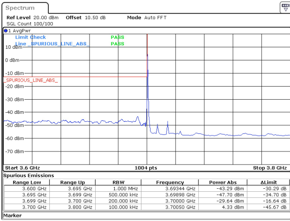
15MHz_15kHz_3707.5MHz_DFT-s-OFDM QPSK_RB1@0 -29.64 dBm
