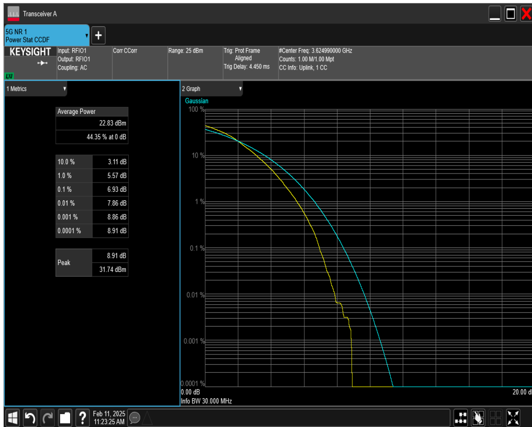
n77(3550-3700) SCS=30kHz DFT_BPSK BW=40MHz Channel=641666 RB=100@0
