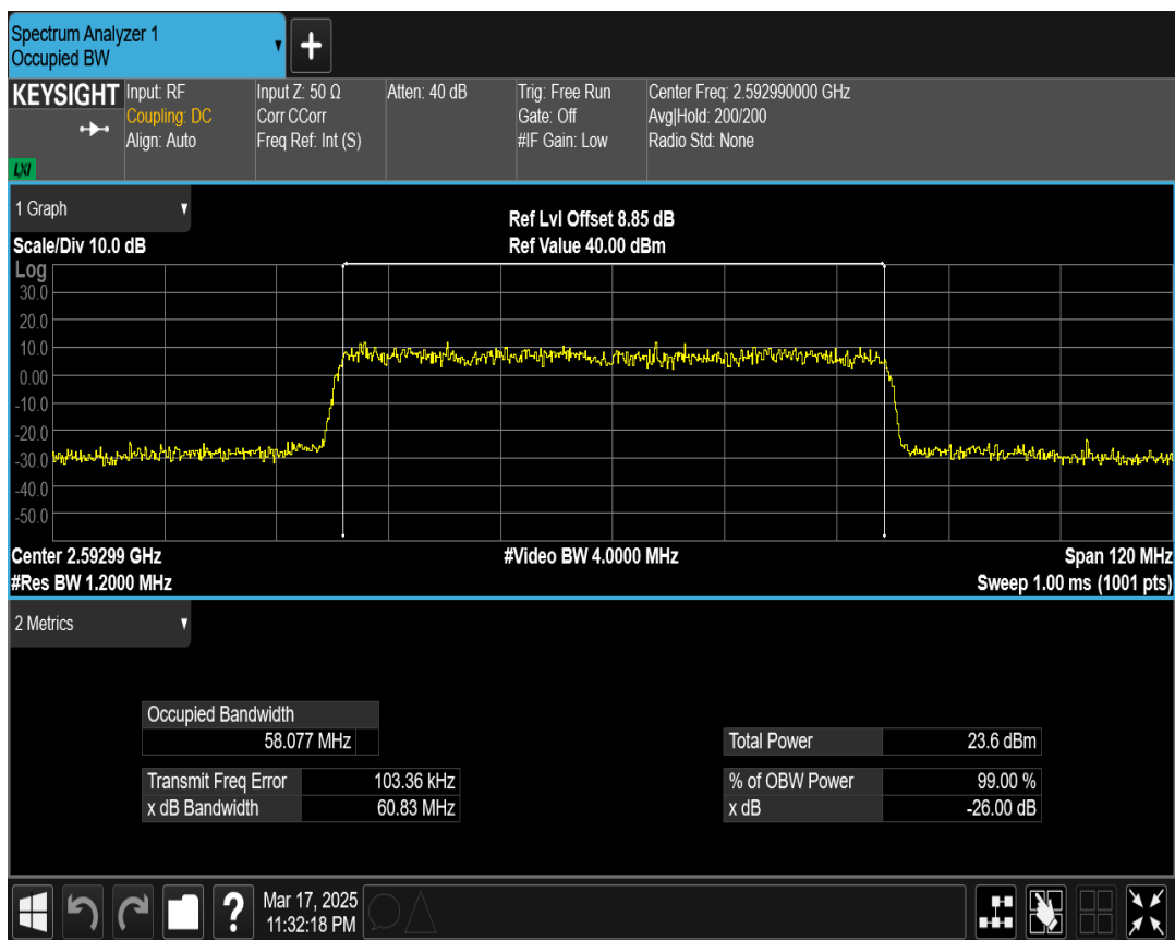
n41 SCS=30kHz CP_QPSK BW=60MHz Channel=518598 RB=162@0
