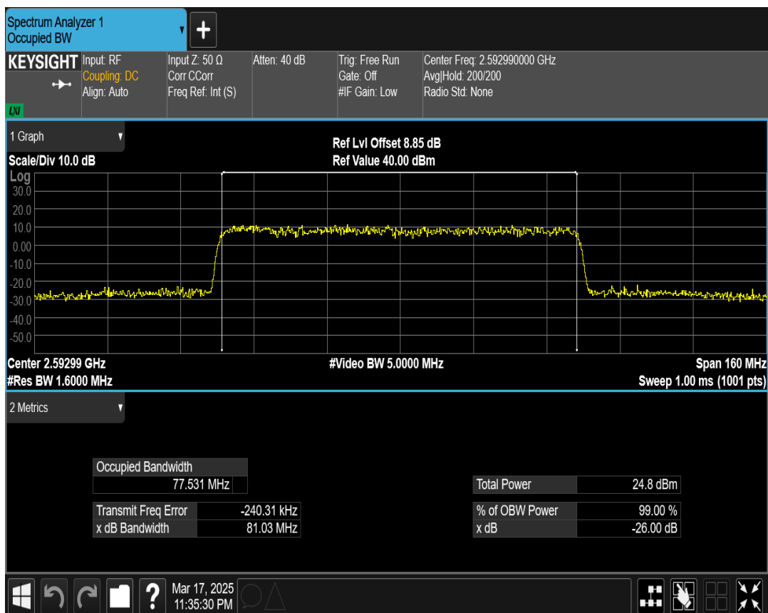
n41 SCS=30kHz CP_QPSK BW=80MHz Channel=518598 RB=217@0
