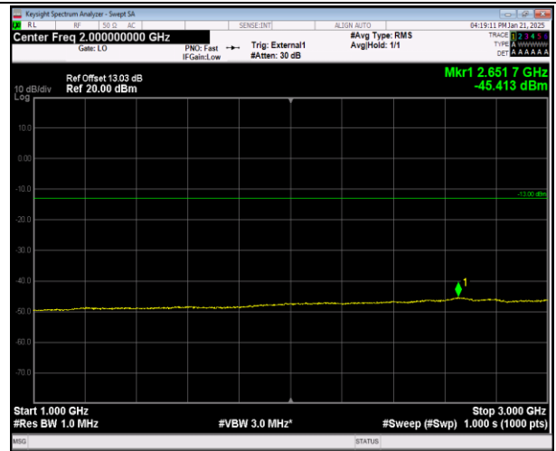
Band42(3450-3550)-5MHz-64QAM-43065-1RB#0-6000~40
