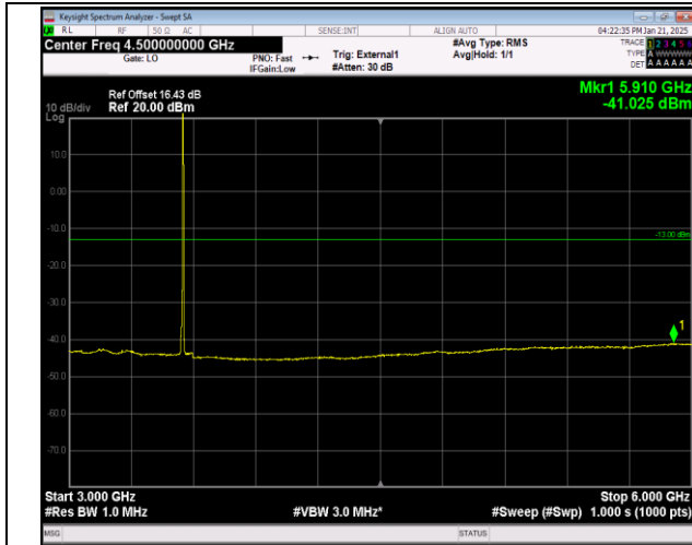
Band42(3450-3550)-5MHz-16QAM-43065-25RB#0-30~100
