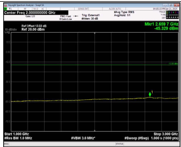
Band42(3450-3550)-5MHz-64QAM-42590-1RB#0-6000~40
