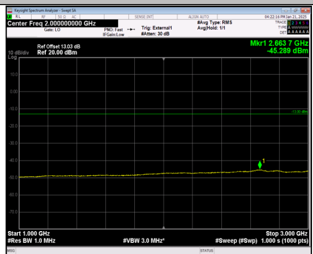
Band42(3450-3550)-5MHz-16QAM-43065-1RB#24-6000~4
