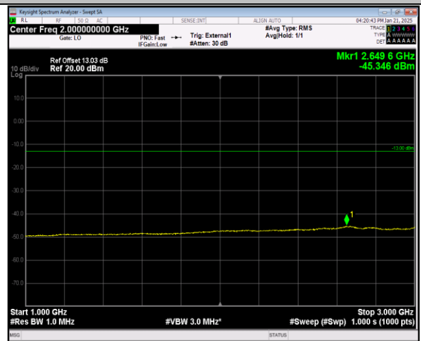
Band42(3450-3550)-5MHz-QPSK-43065-1RB#24-6000~40
