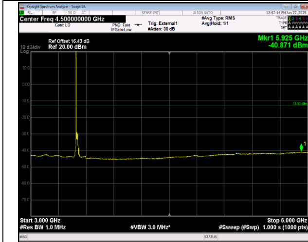
Band42(3450-3550)-20MHz-QPSK-42590-1RB#99-30~100 0
