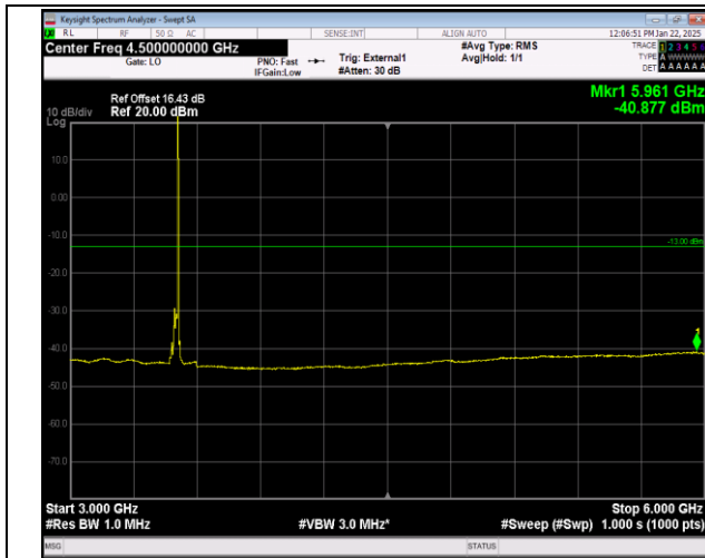
Band42(3450-3550)-20MHz-QPSK-42590-100RB#0-30~10 00
