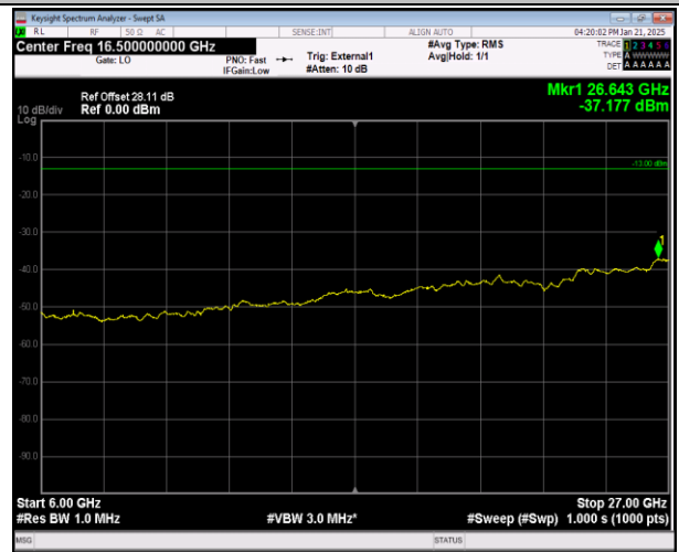
Band42(3450-3550)-5MHz-64QAM-43065-1RB#24-1000~3
