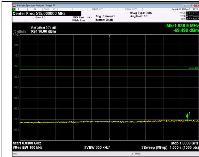
Band42(3450-3550)-5MHz-64QAM-42590-1RB#0-3000~60
