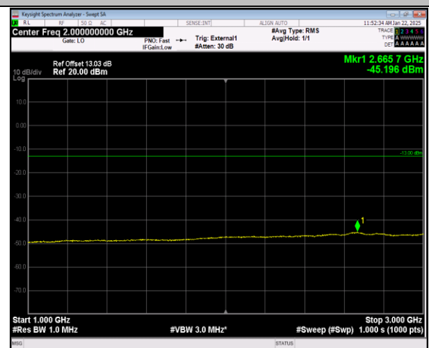
Band42(3450-3550)-20MHz-QPSK-42190-1RB#99-6000~4
