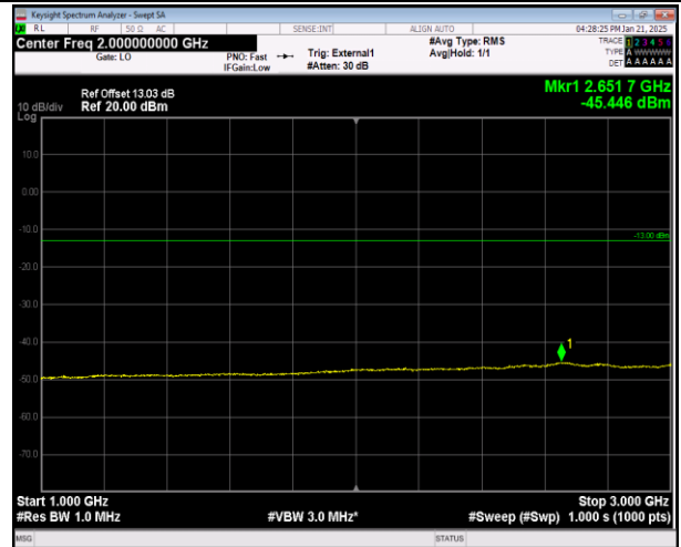
Band42(3450-3550)-5MHz-64QAM-43065-25RB#0-6000~4
