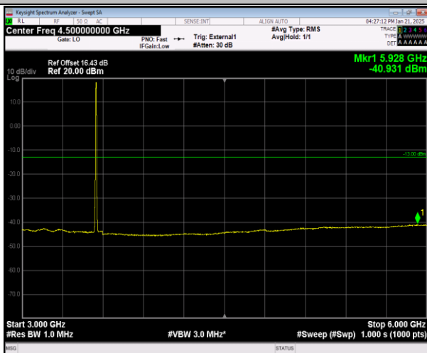
Band42(3450-3550)-20MHz-QPSK-42190-1RB#0-30~1000
