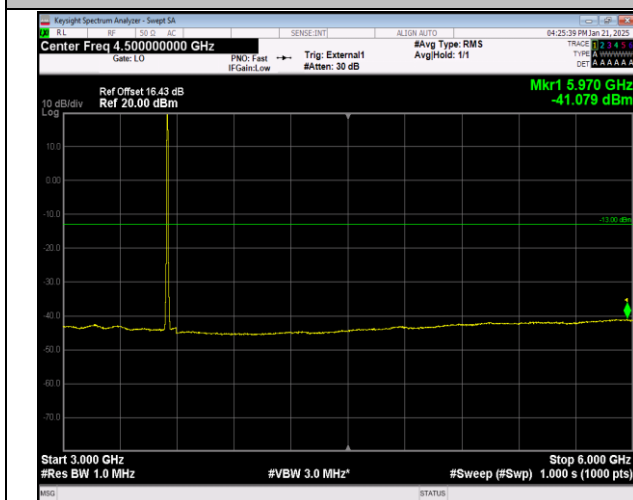
Band42(3450-3550)-5MHz-QPSK-43065-25RB#0-3000~60 00
