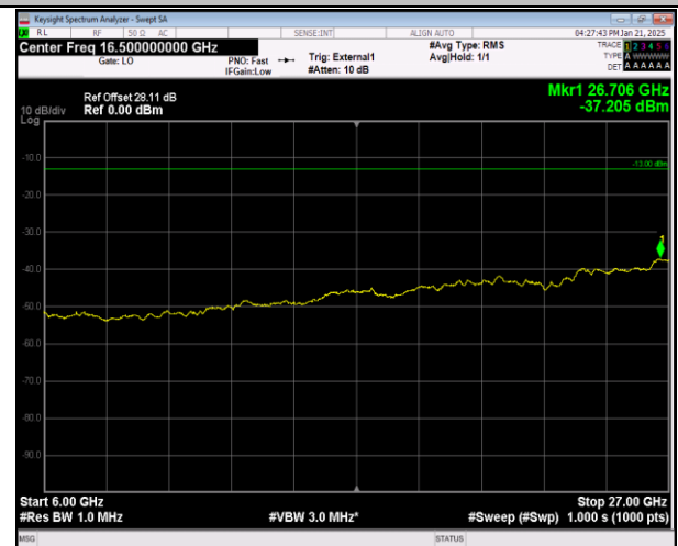
Band42(3450-3550)-20MHz-QPSK-42190-1RB#0-1000~30
