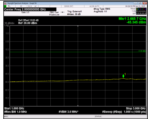
Band42(3450-3550)-5MHz-16QAM-43065-25RB#0-6000~4
