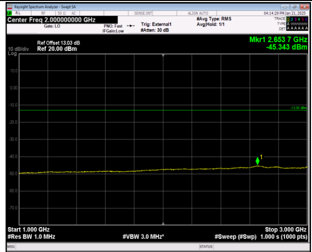
Band42(3450-3550)-5MHz-64QAM-42590-25RB#0-6000~4
