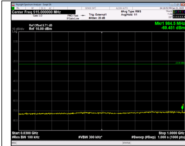
Band42(3450-3550)-5MHz-64QAM-43065-1RB#0-3000~60
