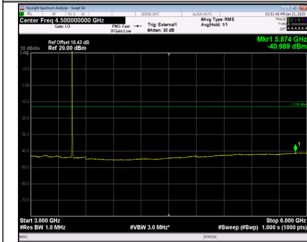
Band42(3450-3550)-5MHz-64QAM-42115-1RB#24-30~100
