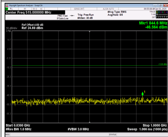
Band66-20MHz-QPSK-132322-1RB#0-Range1:30~1000MHz
