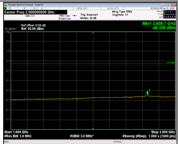
Band42(3450-3550)-5MHz-16QAM-42115-25RB#0-6000~4
