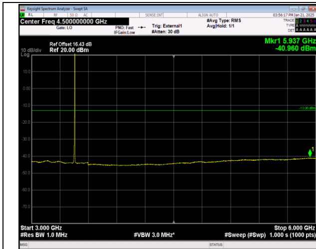
Band42(3450-3550)-5MHz-64QAM-42115-25RB#0-30~100
