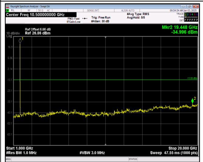
Band66-20MHz-64QAM-132072-1RB#0-Range2:1000~20000MHz
