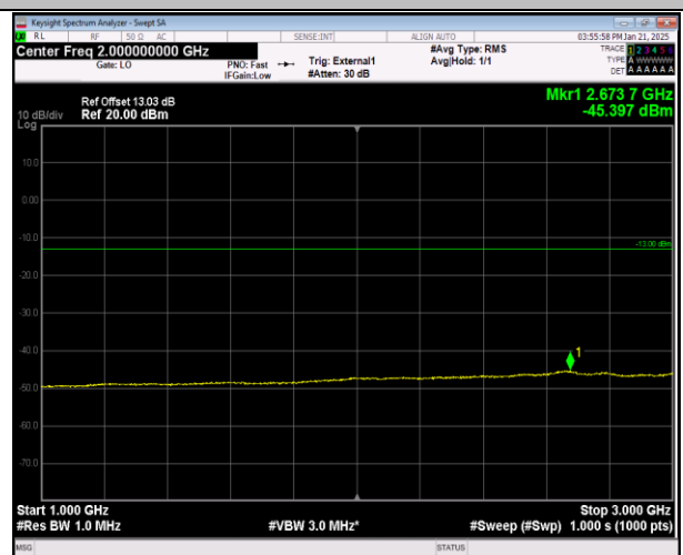
Band42(3450-3550)-5MHz-64QAM-42115-1RB#24-6000~4
