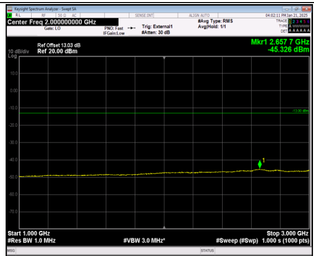
Band42(3450-3550)-5MHz-QPSK-42590-1RB#0-6000~400
