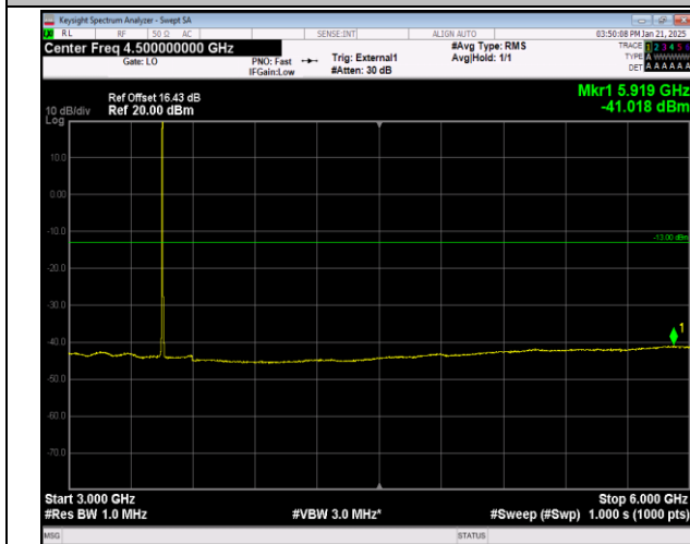
Band42(3450-3550)-5MHz-16QAM-42115-1RB#24-30~100
