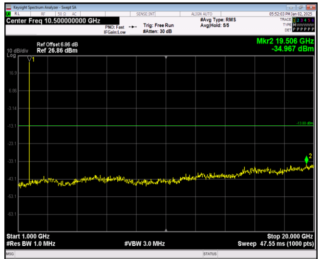
Band66-1.4MHz-QPSK-132665-1RB#0-Range2:1000 ~20000MHz
