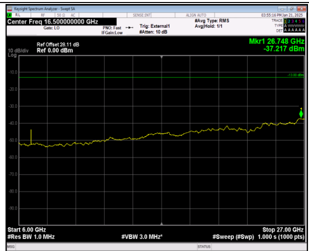
Band42(3450-3550)-5MHz-16QAM-42115-25RB#0-1000~3
