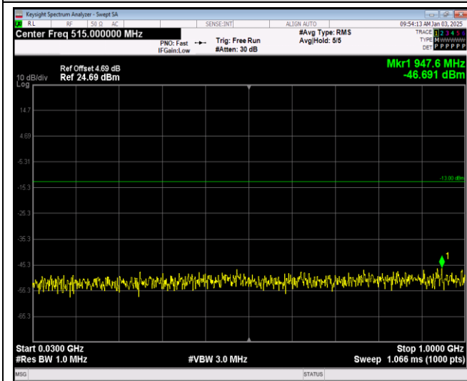
Band66-20MHz-QPSK-132322-1RB#0-Range1:30~1000MHz
