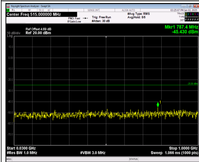
Band38-5MHz-QPSK-38000-1RB#0-Range1:30~100 0MHz
