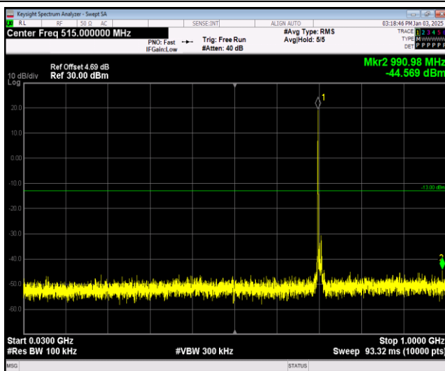
Band17-10MHz-64QAM-23800-1RB#0-Range1:30~1 000MHz
