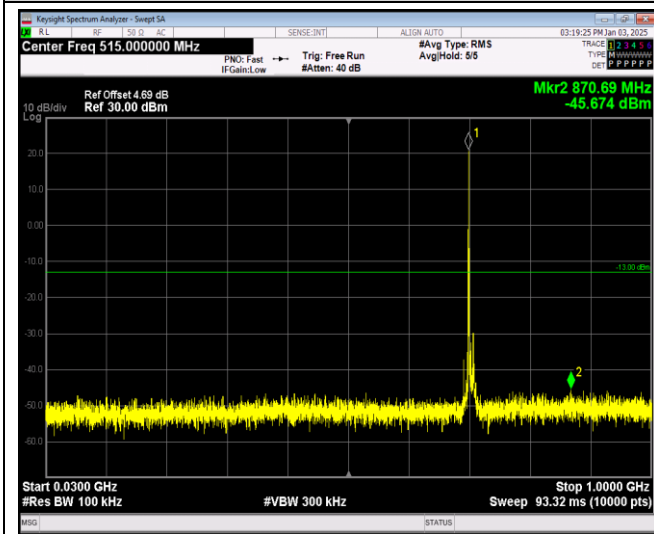
Band17-10MHz-16QAM-23800-1RB#0-Range1:30~1000MHz
