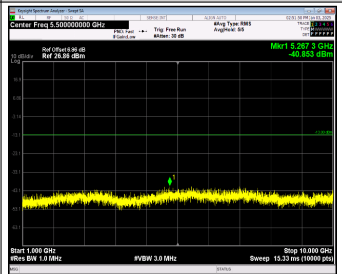
Band17-5MHz-16QAM-23790-1RB#0-Range2:1000~10000MHz
