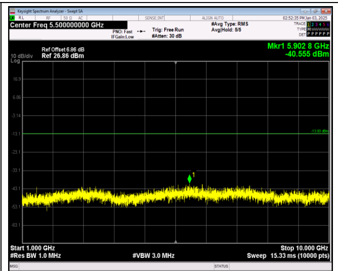
Band17-5MHz-16QAM-23755-1RB#0-Range2:1000~10000MHz
