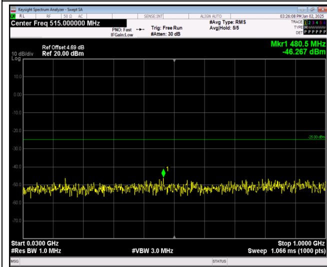
Band38-5MHz-QPSK-38000-1RB#0-Range1:30~100 0MHz
