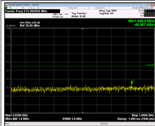
Band41-5MHz-16QAM-39675-1RB#0-Range1:30~10 00MHz
