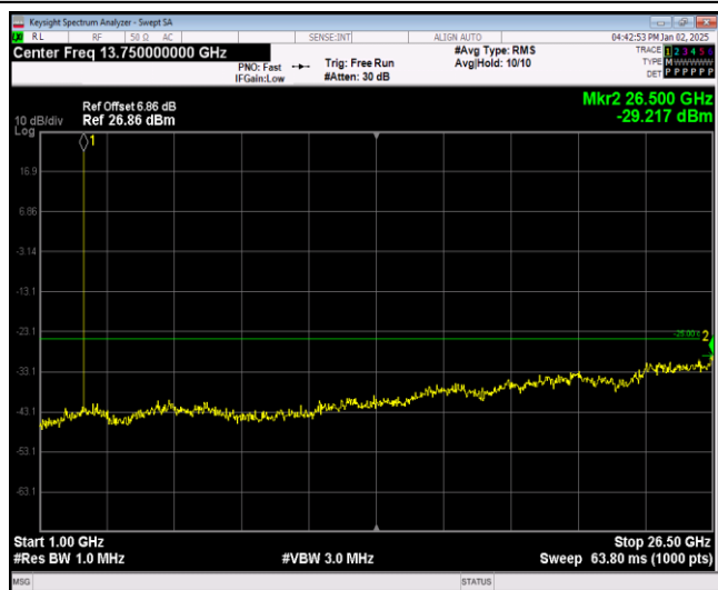
Band41-5MHz-64QAM-39675-1RB#0-Range2:1000~26500MHz
