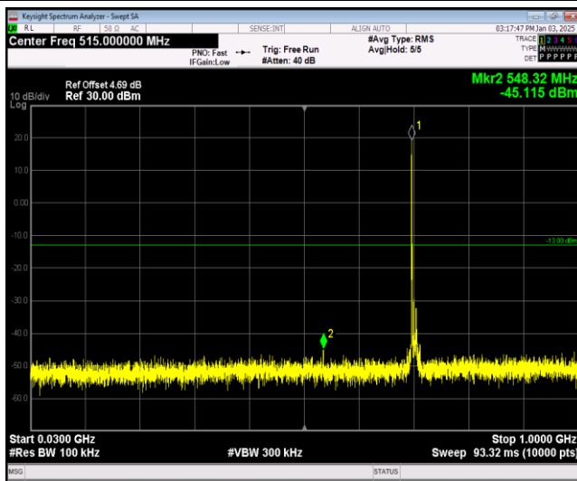
Band17-10MHz-64QAM-23790-1RB#0-Range1:30~1 000MHz
