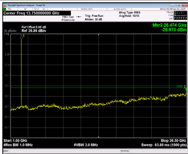
Band41-5MHz-16QAM-41565-1RB#0-Range2:1000~26500MHz
