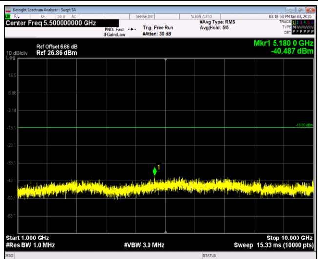
Band17-10MHz-64QAM-23800-1RB#0-Range2:1000 ~10000MHz
