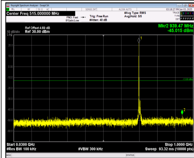
Band17-10MHz-16QAM-23800-1RB#0-Range1:30~1000MHz
