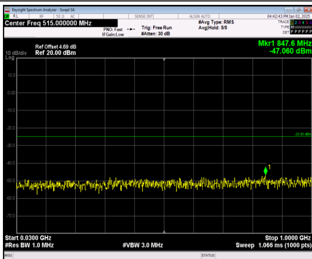
Band41-5MHz-64QAM-39675-1RB#0-Range1:30~1000MHz
