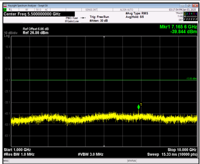
Band17-10MHz-64QAM-23790-1RB#0-Range2:1000 ~10000MHz
