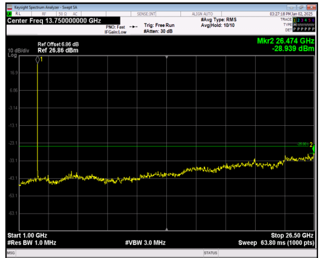
Band38-5MHz-16QAM-37775-1RB#0-Range2:1000~ 26500MHz
