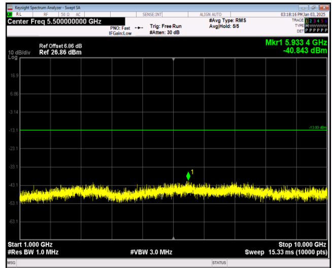
Band17-10MHz-QPSK-23800-1RB#0-Range2:1000~10000MHz
