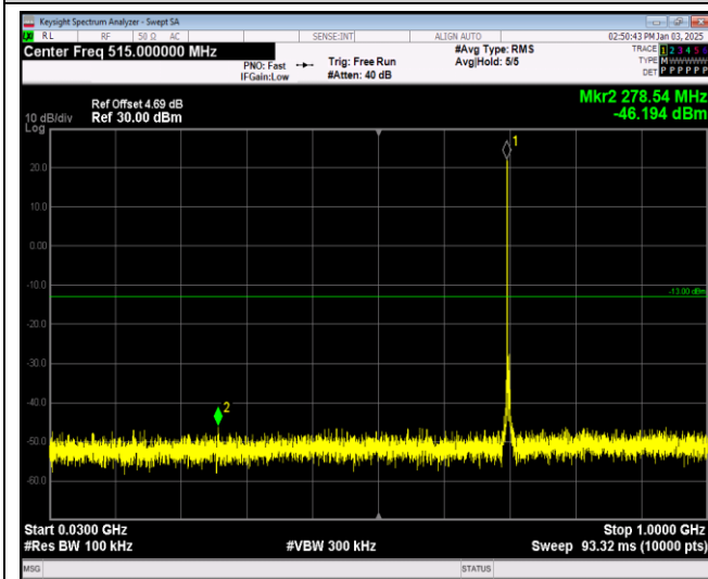
Band17-5MHz-16QAM-23790-1RB#0-Range1:30~1000MHz
