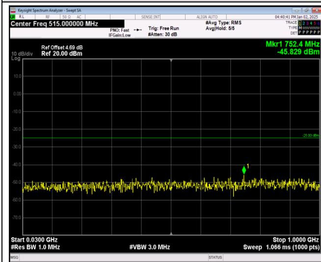
Band41-5MHz-16QAM-39675-1RB#0-Range1:30~10 00MHz
