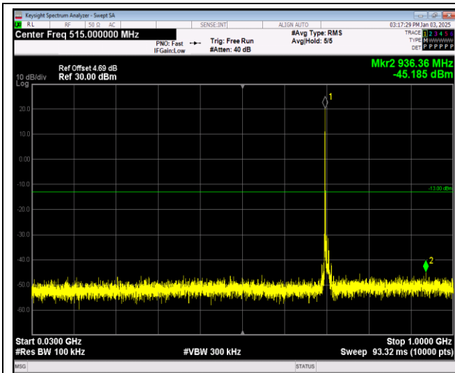
Band17-10MHz-16QAM-23790-1RB#0-Range1:30~1000MHz
