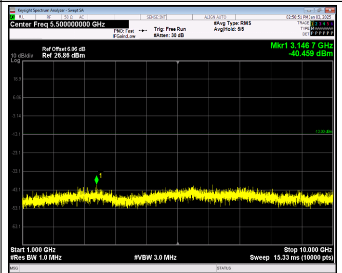
Band17-5MHz-16QAM-23790-1RB#0-Range2:1000~10000MHz
