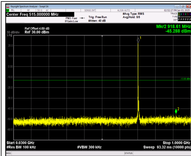
Band17-5MHz-16QAM-23755-1RB#0-Range1:30~1000MHz
