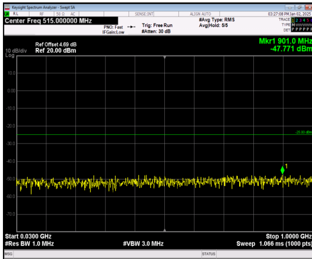
Band38-5MHz-16QAM-37775-1RB#0-Range1:30~10 00MHz
