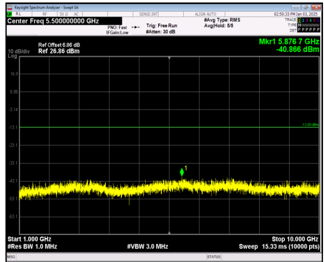
Band17-5MHz-QPSK-23790-1RB#0-Range2:1000~1 0000MHz
