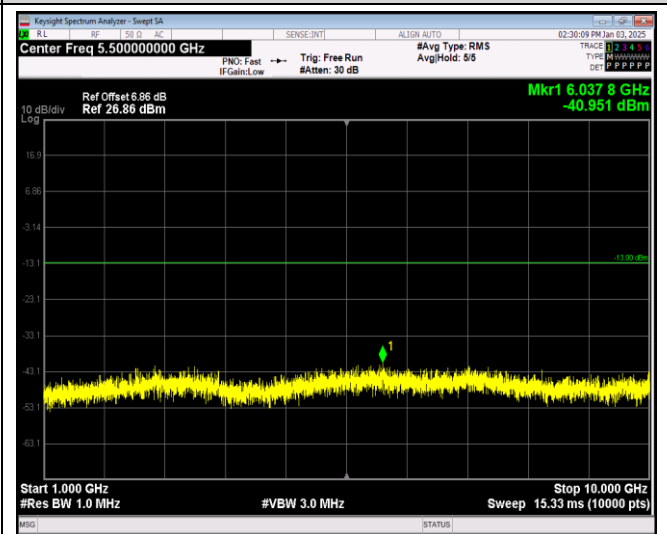
Band12-10MHz-64QAM-23130-1RB#0-Range2:1000~10000MHz
