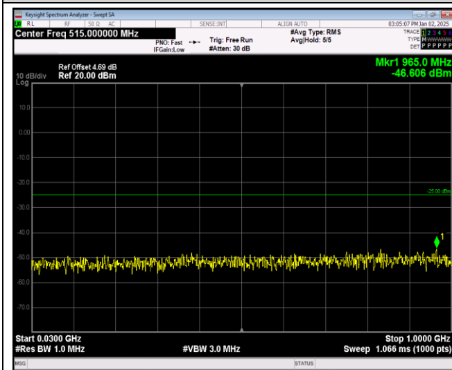
Band7-20MHz-QPSK-21100-1RB#0-Range1:30~100 OMHz
