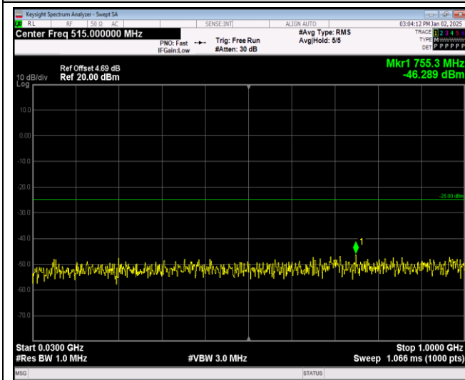
Band7-20MHz-QPSK-21100-1RB#0-Range1:30~100 OMHz
