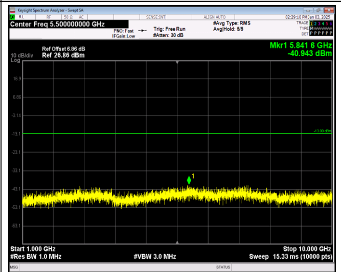
Band12-10MHz-64QAM-23130-1RB#0-Range2:1000~10000MHz
