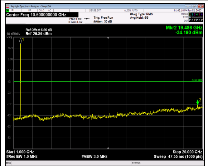
Band4-20MHz-64QAM-20175-1RB#0-Range2:1000~20000MHz
