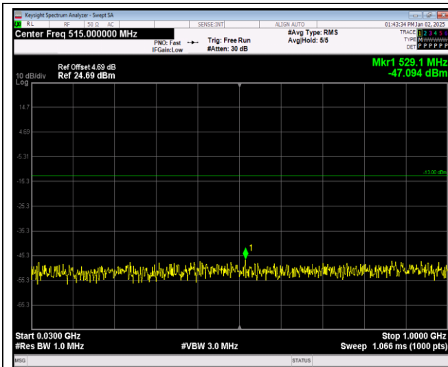
Band4-20MHz-64QAM-20050-1RB#0-Range1:30~1000MHz
