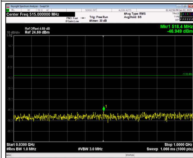
Band4-20MHz-64QAM-20175-1RB#0-Range1:30~1000MHz
