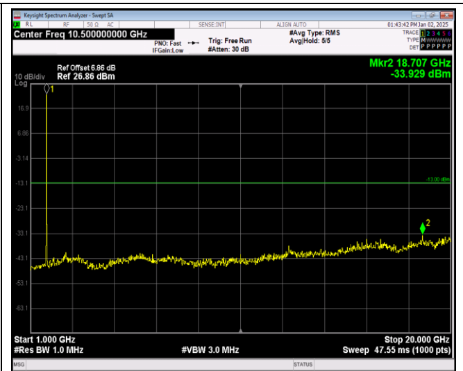
Band4-20MHz-64QAM-20050-1RB#0-Range2:1000~20000MHz
