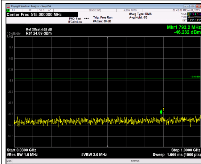
Band4-20MHz-64QAM-20175-1RB#0-Range1:30~1000MHz
