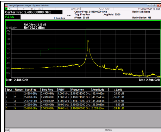
Band41-5MHz-16QAM-39675-25RB#0
