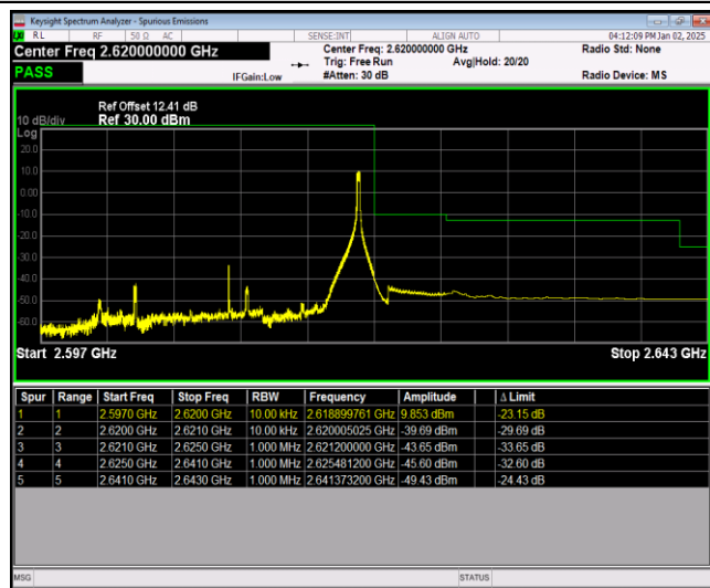
Band38-20MHz-64QAM-37850-1RB#0
