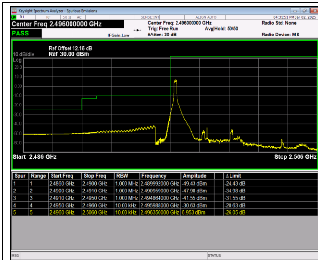
Band41-5MHz-64QAM-39675-25RB#0
