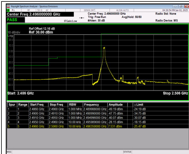
Band41-5MHz-QPSK-39675-25RB#0
