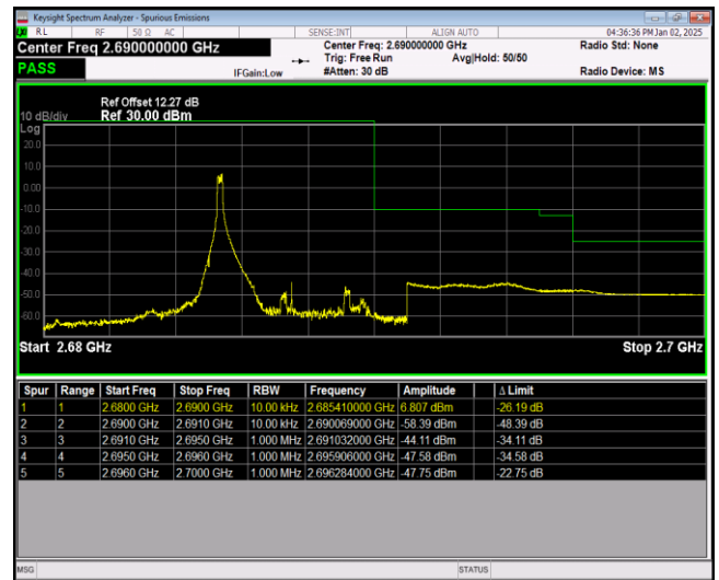
Band41-5MHz-64QAM-41565-25RB#0
