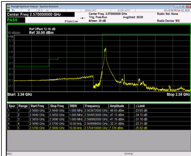
Band38-5MHz-64QAM-37775-25RB#0
