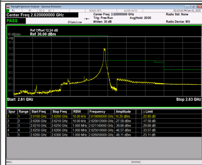
Band38-5MHz-16QAM-37775-1RB#0
