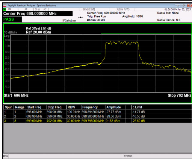
Band12-1.4MHz-64QAM-23173-1RB#5
