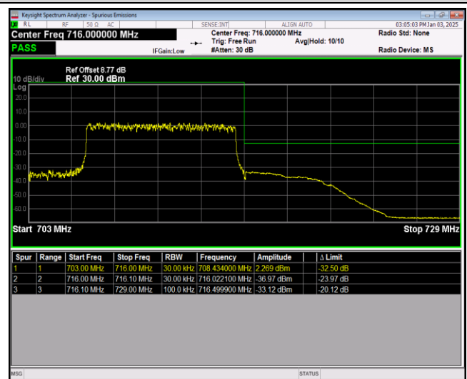
Band17-10MHz-16QAM-23780-1RB#49
