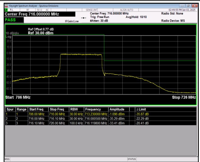
Band17-10MHz-QPSK-23780-1RB#49
