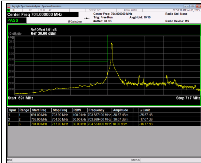
Band17-10MHz-16QAM-23780-50RB#0
