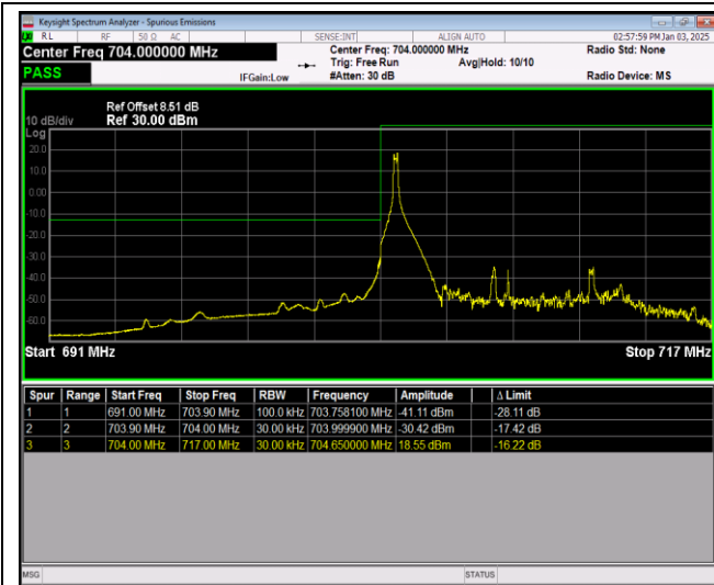
Band17-10MHz-QPSK-23780-50RB#0
