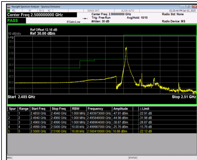
Band7-5MHz-64QAM-20775-25RB#0
