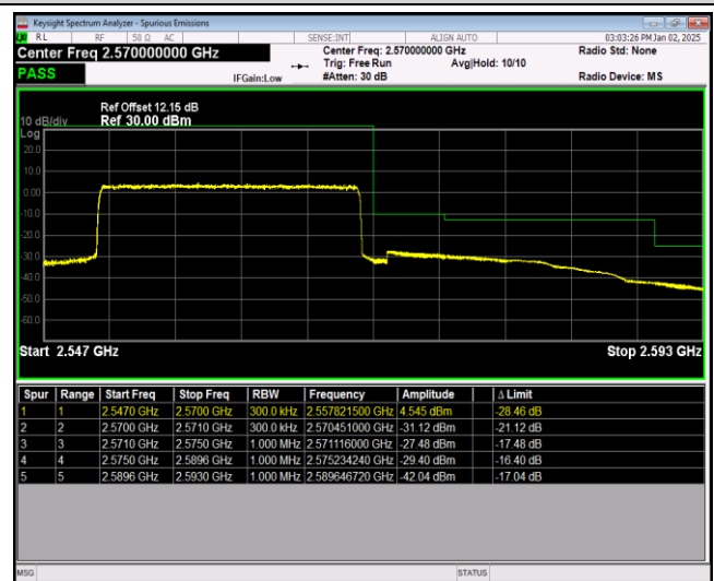
Band7-20MHz-64QAM-20850-1RB#99
