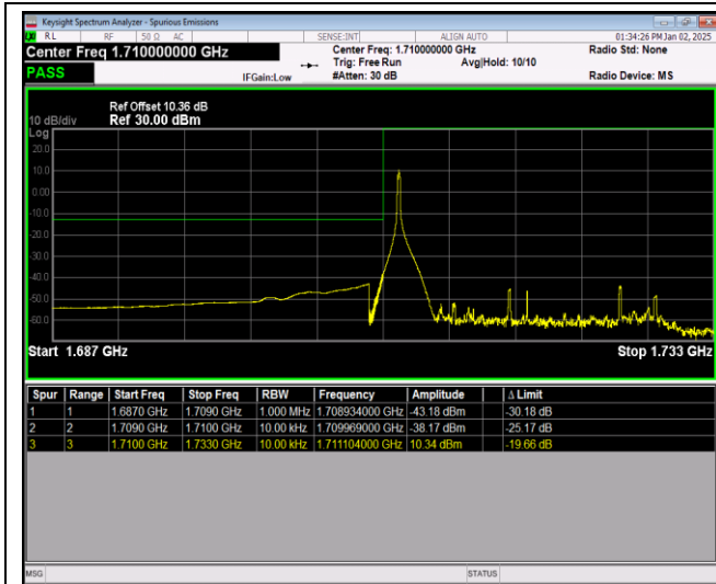
Band4-20MHz-64QAM-20050-100RB#0
