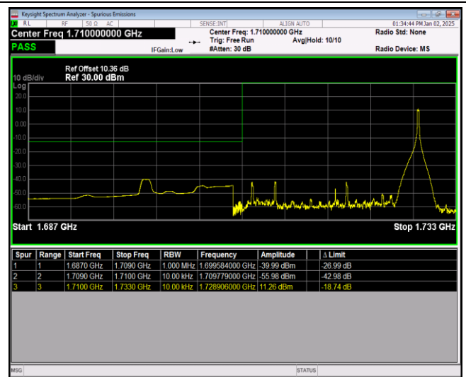
Band4-20MHz-QPSK-20300-1RB#0
