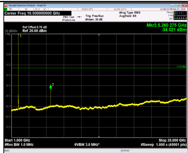
66-66-5MHz-20MHz-16QAM-16QAM-132428-132572-1RB# 0-0RB#0-1000~20000MHz-PASS
