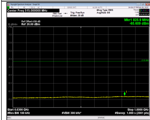
66-66-20MHz-5MHz-16QAM-16QAM-132072-132189-1R B#0-0RB#0-30~1000MHz-PASS
