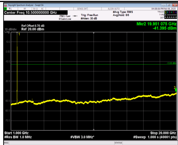
66-66-20MHz-5MHz-16QAM-16QAM-132072-132189-1RB# 99-ORB#0-1000~20000MHz-PASS
