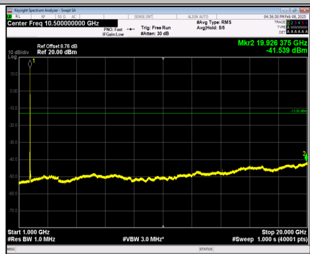
66-66-20MHz-5MHz-16QAM-16QAM-132397-132514-1RB# 0-1RB#24-1000~20000MHz-PASS
