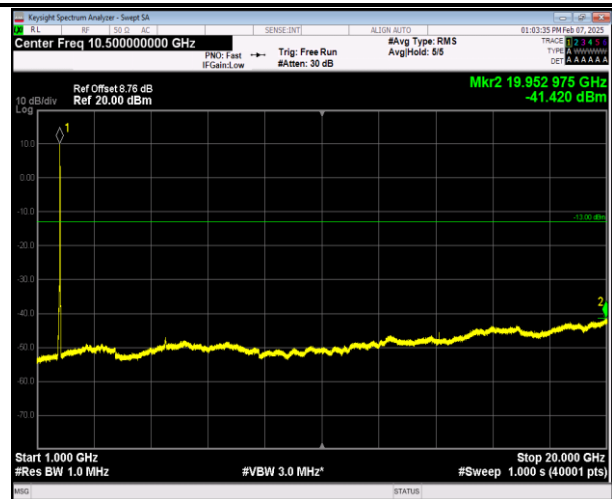
66-66-5MHz-20MHz-16QAM-16QAM-132428-132572-25RB #0-100RB#0-1000~20000MHz-PASS
