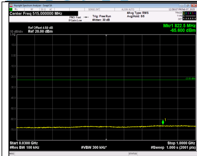
66-66-5MHz-20MHz-16QAM-16QAM-132428-132572-1R B#0-0RB#0-30~1000MHz-PASS
