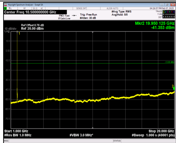
66-66-5MHz-20MHz-16QAM-16QAM-132455-132572-1RB# 0-ORB#0-1000~20000MHz-PASS
