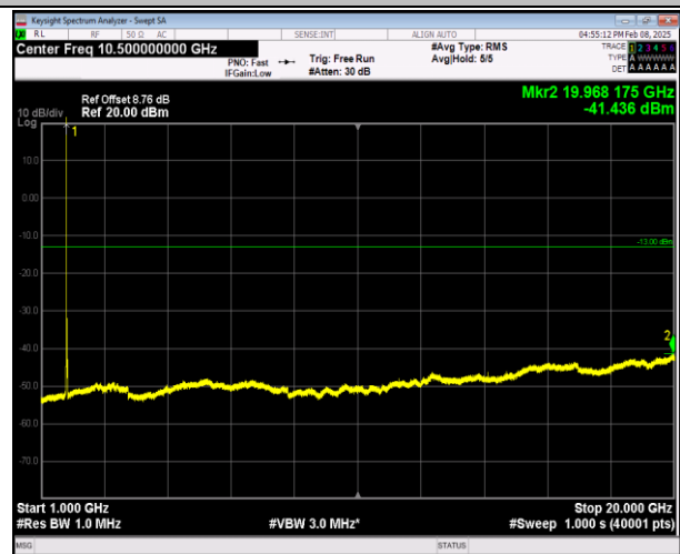
66-66-20MHz-5MHz-16QAM-16QAM-132522-132639-1RB# 0-ORB#0-1000~20000MHz-PASS
