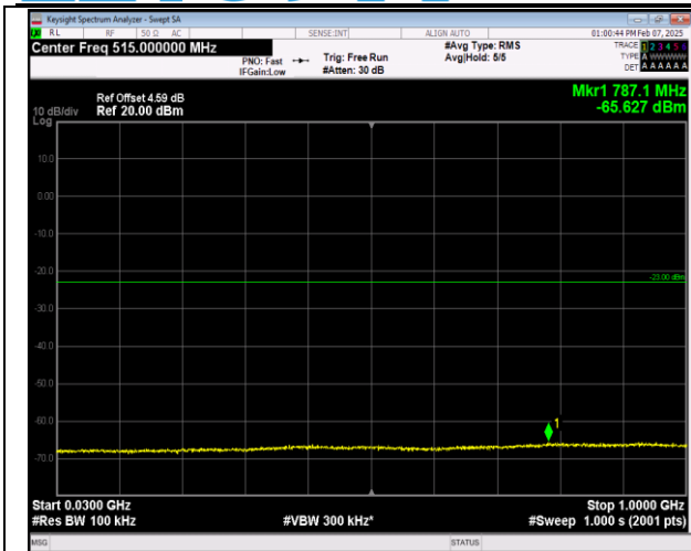
66-66-5MHz-20MHz-QPSK-QPSK-132428-132572-1RB# 0-1RB#99-30~1000MHz-PASS
