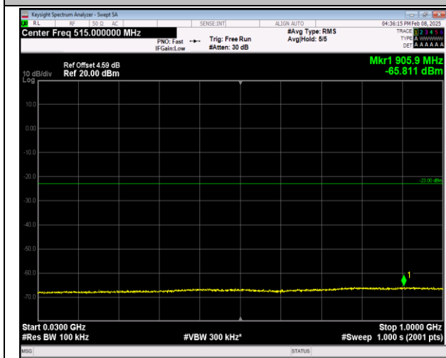
66-66-20MHz-5MHz-16QAM-16QAM-132397-132514-1R B#0-1RB#24-30~1000MHz-PASS
