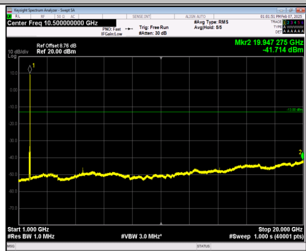
66-66-5MHz-20MHz-16QAM-16QAM-132428-132572-1RB# 0-1RB#99-1000~20000MHz-PASS
