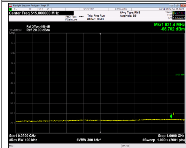
66-66-20MHz-5MHz-16QAM-16QAM-132522-132639-1RB# B#0-ORB#0-30~1000MHz-PASS
