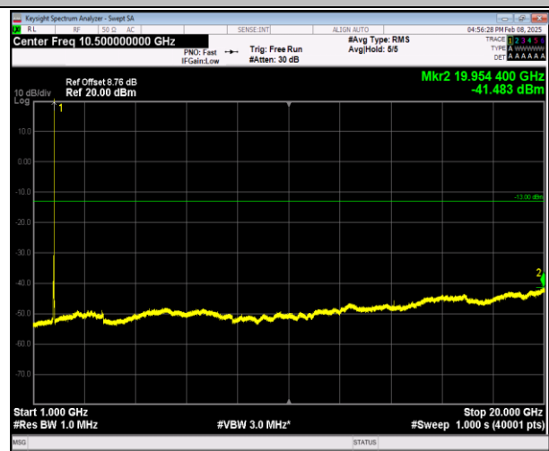
66-66-20MHz-5MHz-16QAM-16QAM-132522-132639-1RB# 99-0RB#0-1000~20000MHz-PASS
