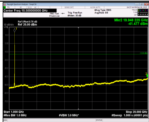
66-66-20MHz-5MHz-16QAM-16QAM-132522-132639-1RB# 0-1RB#24-1000~20000MHz-PASS
