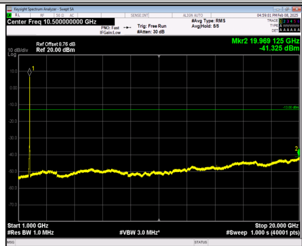
66-66-20MHz-5MHz-16QAM-16QAM-132522-132639-100R B#0-25RB#0-1000~20000MHz-PASS
