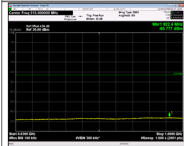
66-66-5MHz-20MHz-16QAM-16QAM-132428-132572-1R B#24-0RB#0-30~1000MHz-PASS
