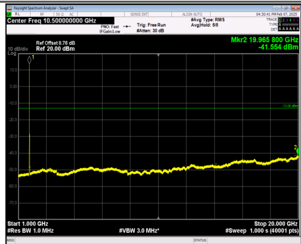
66-66-5MHz-20MHz-16QAM-16QAM-132455-132572-25RB #0-100RB#0-1000~20000MHz-PASS
