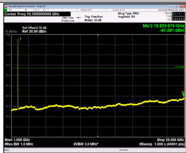
66-66-20MHz-5MHz-16QAM-16QAM-132072-132189-100R B#0-25RB#0-1000~20000MHz-PASS
