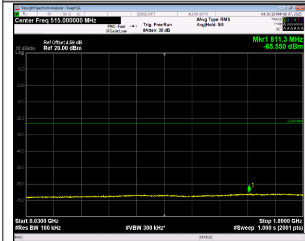
66-66-5MHz-20MHz-16QAM-16QAM-132455-132572-25 RB#0-100RB#0-30~1000MHz-PASS
