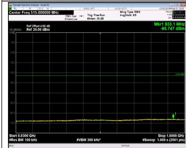
66-66-5MHz-20MHz-16QAM-16QAM-132027-132171-1R B#24-ORB#0-30~1000MHz-PASS
