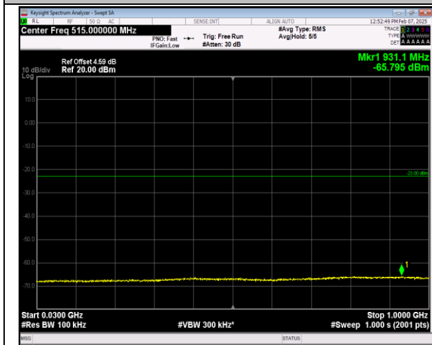
66-66-5MHz-20MHz-16QAM-16QAM-132328-132472-1R B#24-0RB#0-30~1000MHz-PASS
