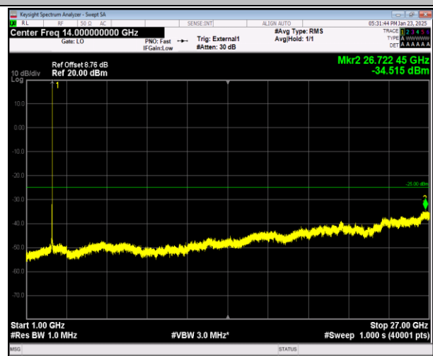
41-41-20MHz-20MHz-16QAM-16QAM-41292-41490-1RB#9 9-0RB#0-1000~27000MHz-PASS
