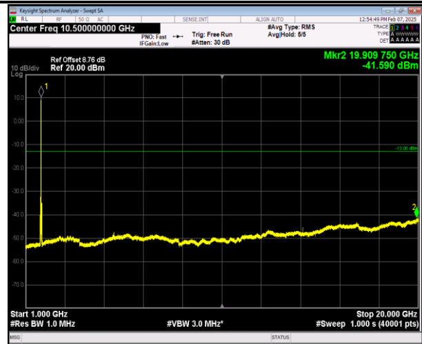
66-66-5MHz-20MHz-16QAM-16QAM-132328-132472-1RB# 0-1RB#99-1000~20000MHz-PASS
