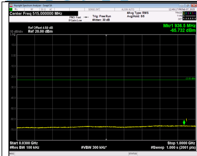
66-66-5MHz-20MHz-16QAM-16QAM-132027-132171-25 RB#0-100RB#0-30~1000MHz-PASS
