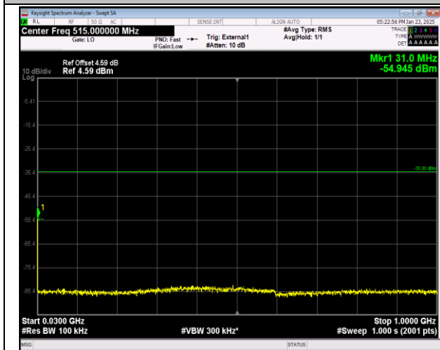
41-41-20MHz-20MHz-16QAM-16QAM-40521-40719-1RB #99-ORB#0-30~1000MHz-PASS
