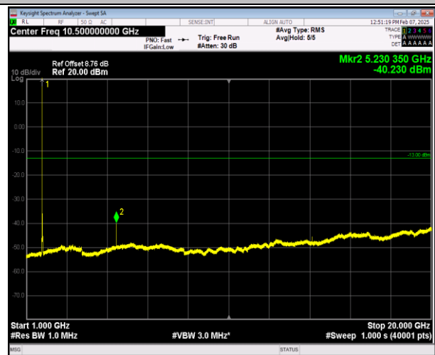
66-66-5MHz-20MHz-16QAM-16QAM-132328-132472-1RB# 0-ORB#0-1000~20000MHz-PASS
