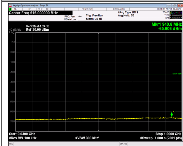
66-66-5MHz-20MHz-16QAM-16QAM-132328-132472-1R B#0-ORB#0-30~1000MHz-PASS
