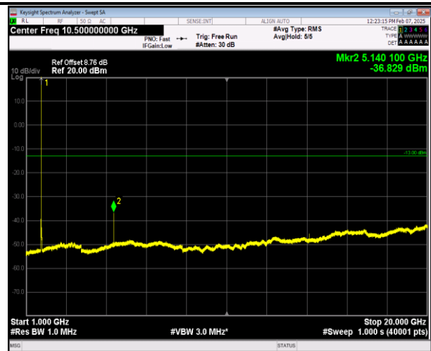
66-66-5MHz-20MHz-16QAM-16QAM-132027-132171-1RB# 0-ORB#0-1000~20000MHz-PASS
