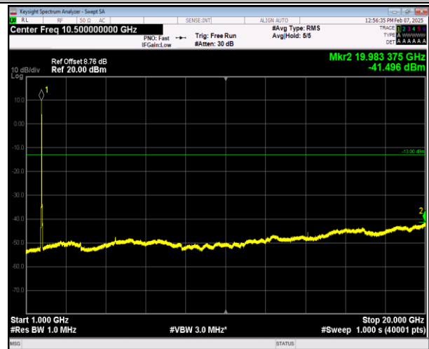
66-66-5MHz-20MHz-16QAM-16QAM-132328-132472-25RB #0-100RB#0-1000~20000MHz-PASS
