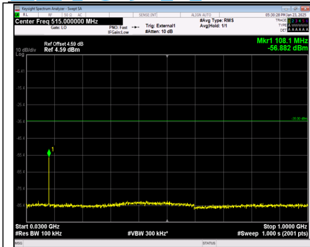
41-41-20MHz-20MHz-QPSK-QPSK-41292-41490-1RB#9 9-ORB#0-30~1000MHz-PASS
