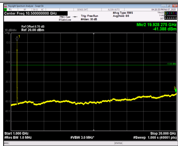
66-66-5MHz-20MHz-16QAM-16QAM-132005-132122-25RB #0-100RB#0-1000~20000MHz-PASS
