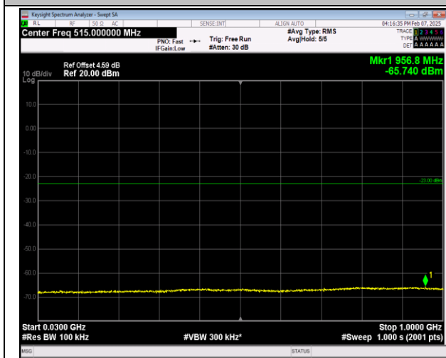
66-66-5MHz-20MHz-16QAM-16QAM-132005-132122-1RB B#0-0RB#0-30~1000MHz-PASS
