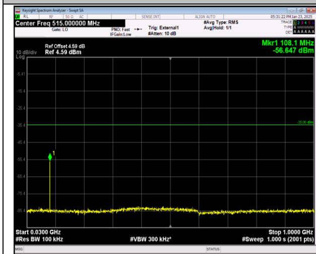
41-41-20MHz-20MHz-16QAM-16QAM-41292-41490-1RB #99-0RB#0-30~1000MHz-PASS
