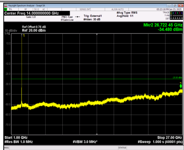
41-41-20MHz-20MHz-16QAM-16QAM-40521-40719-1RB#9 9-ORB#0-1000~27000MHz-PASS
