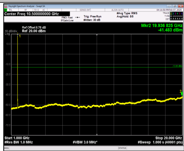
66-66-5MHz-20MHz-16QAM-16QAM-132005-132122-1RB# 0-0RB#0-1000~20000MHz-PASS
