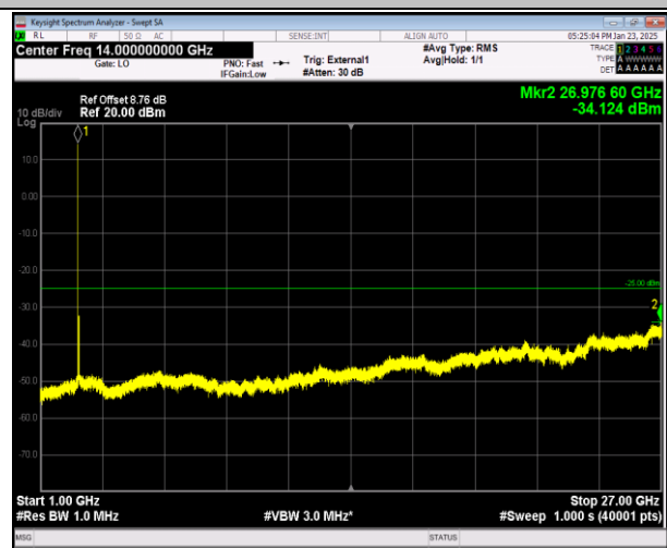
41-41-20MHz-20MHz-16QAM-16QAM-40521-40719-1RB#0 -1RB#99-1000~27000MHz-PASS
