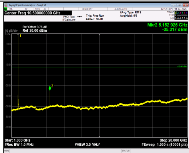
66-66-5MHz-20MHz-16QAM-16QAM-132027-132171-1RB# 24-ORB#0-1000~20000MHz-PASS
