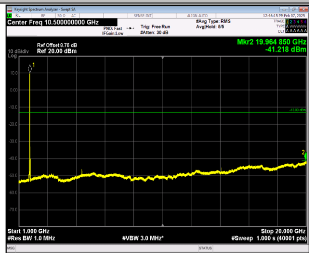
66-66-5MHz-20MHz-16QAM-16QAM-132027-132171-1RB# 0-1RB#99-1000~20000MHz-PASS
