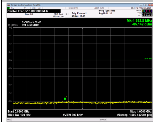
41-41-20MHz-20MHz-16QAM-16QAM-40521-40719-1RB #0-1RB#99-30~1000MHz-PASS
