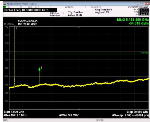
66-66-5MHz-20MHz-QPSK-QPSK-132005-132122-1RB#0- ORB#0-1000~20000MHz-PASS
