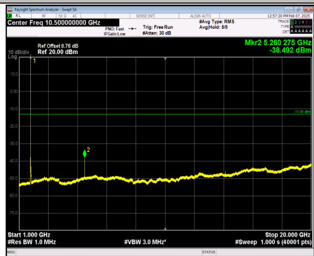
66-66-5MHz-20MHz-QPSK-QPSK-132428-132572-1RB#0- ORB#0-1000~20000MHz-PASS
