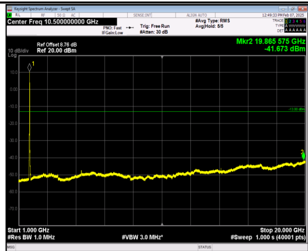
66-66-5MHz-20MHz-16QAM-16QAM-132027-132171-25RB #0-100RB#0-1000~20000MHz-PASS
