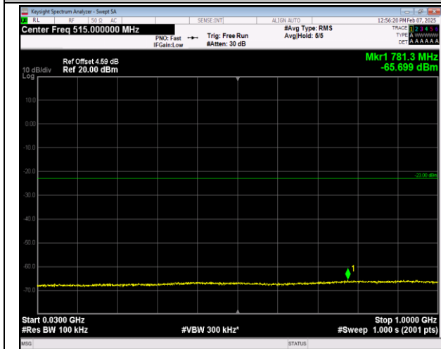
66-66-5MHz-20MHz-16QAM-16QAM-132328-132472-25 RB#0-100RB#0-30~1000MHz-PASS
