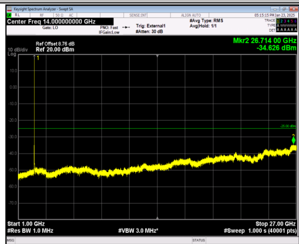
41-41-20MHz-20MHz-QPSK-QPSK-39750-39948-1RB#99- ORB#0-1000~27000MHz-PASS
