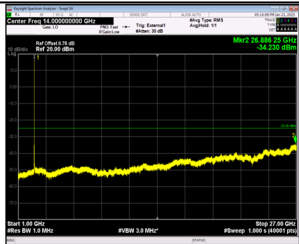
41-41-20MHz-20MHz-16QAM-16QAM-39750-39948-1RB#9 9-0RB#0-1000~27000MHz-PASS
