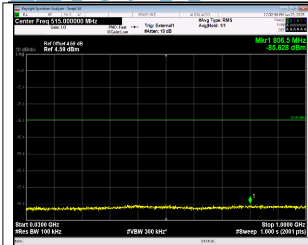
41-41-20MHz-5MHz-QPSK-QPSK-40595-40712-1RB#0-1RB#24-30~1000MHz-PASS
