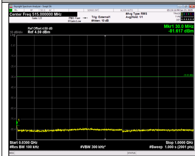
41-41-20MHz-20MHz-16QAM-16QAM-39750-39948-100 RB#0-100RB#0-30~1000MHz-PASS
