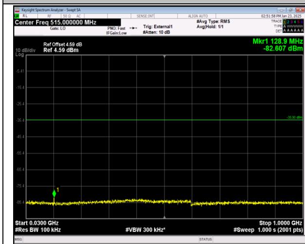
41-41-20MHz-10MHz-16QAM-16QAM-39750-39894-1RB #0-0RB#0-30~1000MHz-PASS
