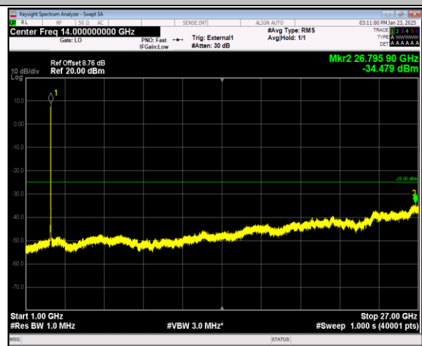
41-41-20MHz-10MHz-QPSK-QPSK-41391-41535-100RB#0 -50RB#0-1000~27000MHz-PASS
