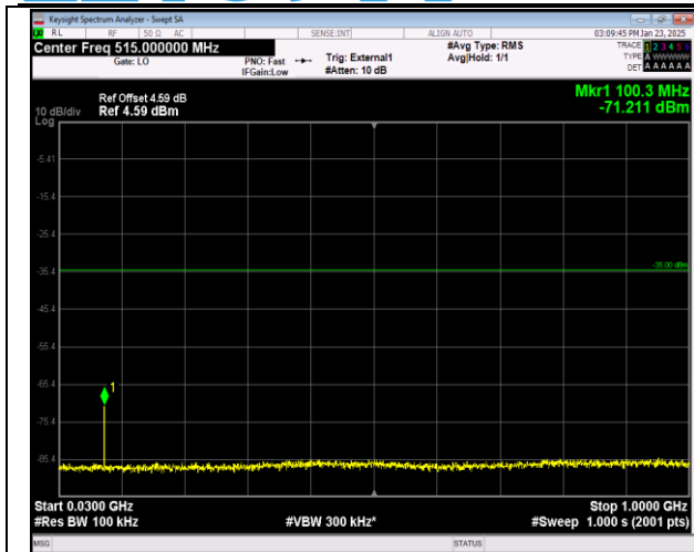
41-41-20MHz-10MHz-16QAM-16QAM-41391-41535-1RB #0-1RB#49-30~1000MHz-PASS
