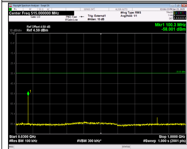
41-41-20MHz-10MHz-16QAM-16QAM-41391-41535-1RB #0-ORB#0-30~1000MHz-PASS
