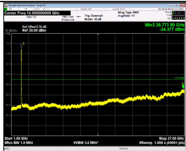
41-41-20MHz-20MHz-QPSK-QPSK-39750-39948-100RB#0 -100RB#0-1000~27000MHz-PASS
