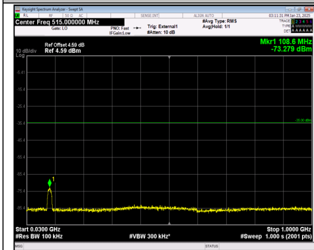
41-41-20MHz-10MHz-16QAM-16QAM-41391-41535-100 RB#0-50RB#0-30~1000MHz-PASS
