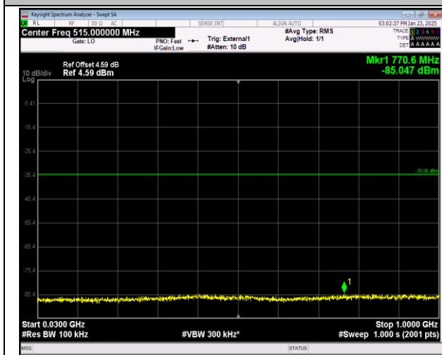
41-41-20MHz-10MHz-16QAM-16QAM-40571-40715-1RB #0-1RB#49-30~1000MHz-PASS
