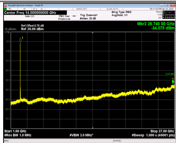
41-41-20MHz-20MHz-16QAM-16QAM-39750-39948-1RB#0 -1RB#99-1000~27000MHz-PASS
