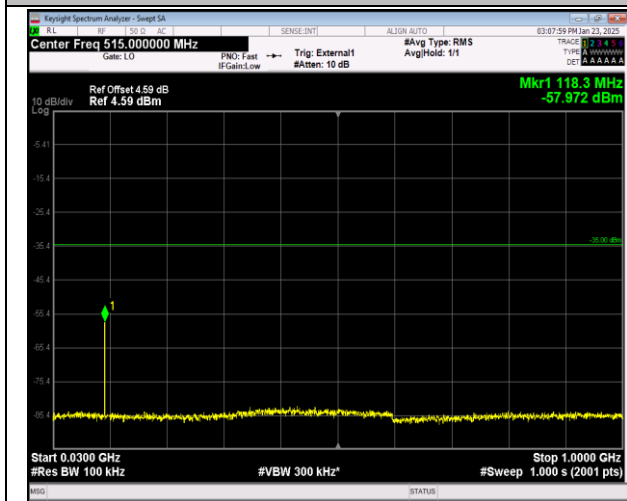
41-41-20MHz-10MHz-16QAM-16QAM-41391-41535-1RB #99-0RB#0-30~1000MHz-PASS
