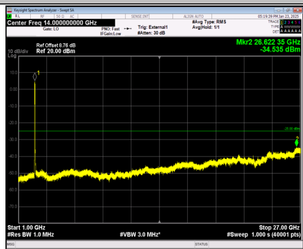
41-41-20MHz-20MHz-16QAM-16QAM-39750-39948-100RB #0-100RB#0-1000~27000MHz-PASS
