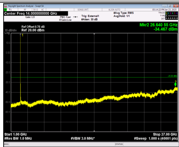
41-41-20MHz-20MHz-16QAM-16QAM-39750-39948-1RB#0 -0RB#0-1000~27000MHz-PASS
