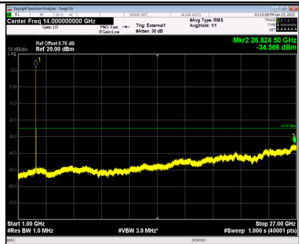
41-41-20MHz-10MHz-16QAM-16QAM-41391-41535-1RB#0 -1RB#49-1000~27000MHz-PASS
