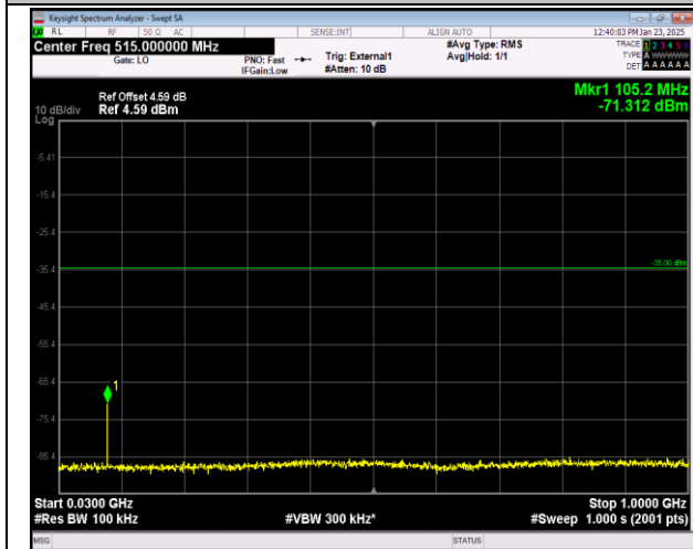
41-41-20MHz-5MHz-QPSK-QPSK-41440-41557-1RB#0-01RB#24-30~1000MHz-PASS
