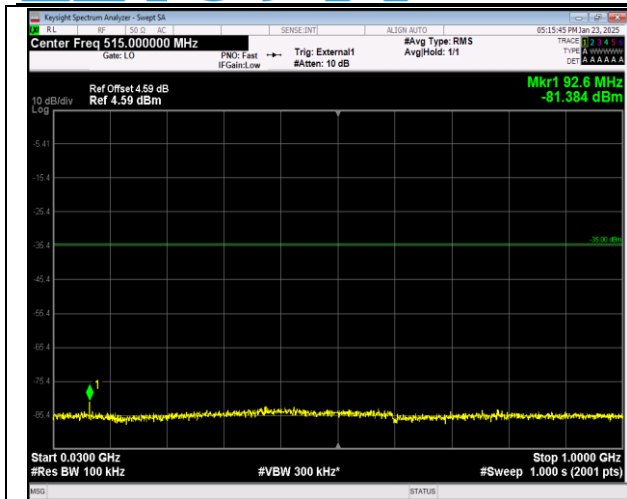
41-41-20MHz-20MHz-16QAM-16QAM-39750-39948-1RB #99-0RB#0-30~1000MHz-PASS
