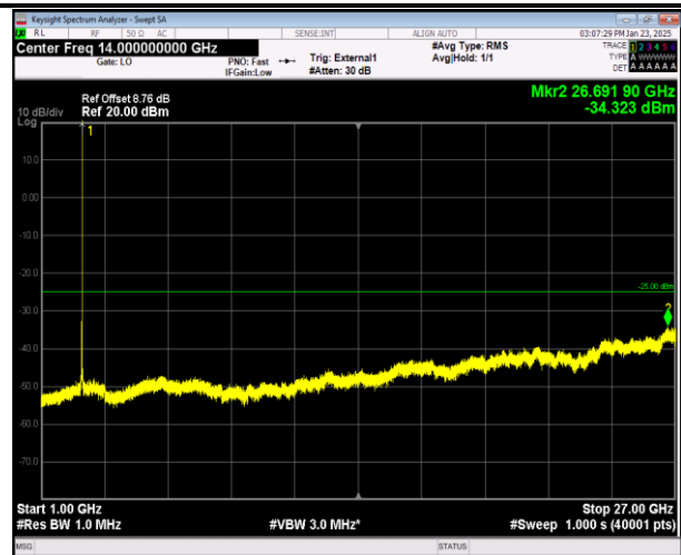
41-41-20MHz-10MHz-QPSK-QPSK-41391-41535-1RB#99- ORB#0-1000~27000MHz-PASS
