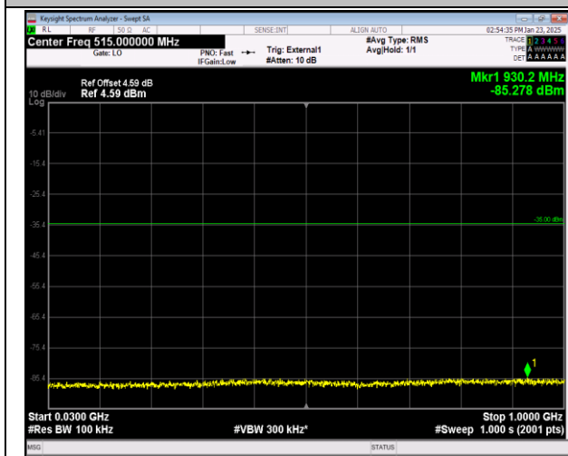
41-41-20MHz-10MHz-QPSK-QPSK-39750-39894-1RB#0 -1RB#49-30~1000MHz-PASS
