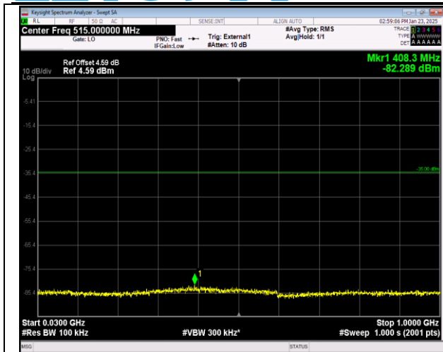
41-41-20MHz-10MHz-16QAM-16QAM-40571-40715-1RB #0-ORB#0-30~1000MHz-PASS
