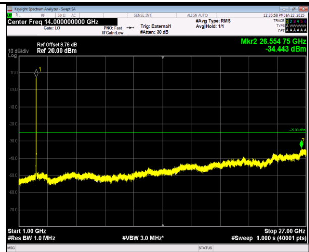
41-41-20MHz-5MHz-16QAM-16QAM-40595-40712-100RB# 0-25RB#0-1000~27000MHz-PASS
