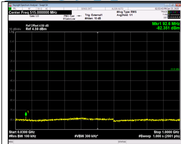
41-41-20MHz-10MHz-16QAM-16QAM-39750-39894-1RB #99-0RB#0-30~1000MHz-PASS
