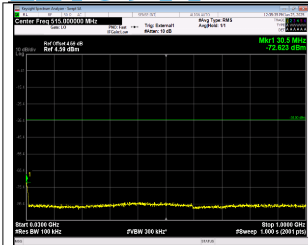
41-41-20MHz-5MHz-16QAM-16QAM-40595-40712-100R B#0-25RB#0-30~1000MHz-PASS
