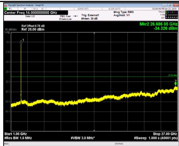
41-41-20MHz-10MHz-16QAM-16QAM-40571-40715-100RB #0-50RB#0-1000~27000MHz-PASS
