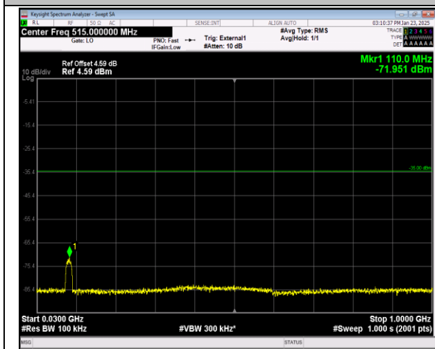
41-41-20MHz-10MHz-QPSK-QPSK-41391-41535-100RB #0-50RB#0-30~1000MHz-PASS
