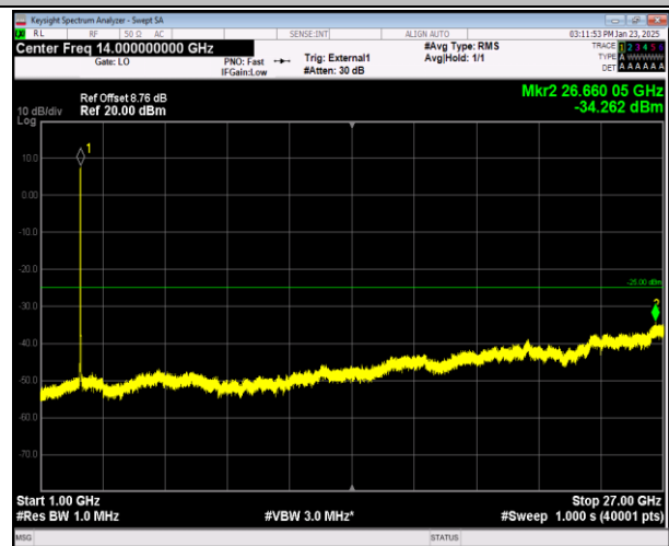
41-41-20MHz-10MHz-16QAM-16QAM-41391-41535-100RB #0-50RB#0-1000~27000MHz-PASS
