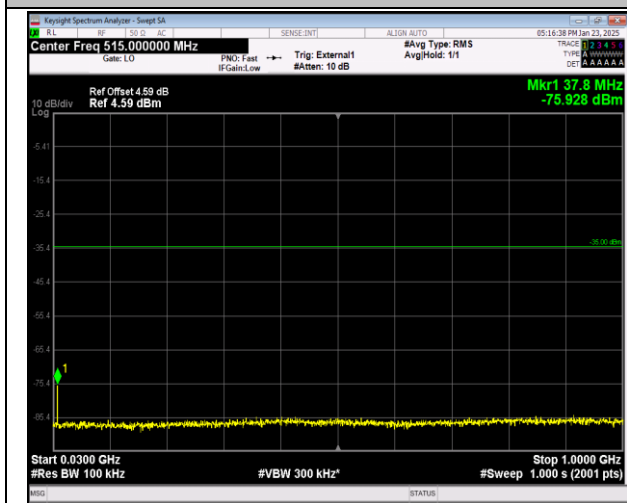
41-41-20MHz-20MHz-QPSK-QPSK-39750-39948-1RB#0 -1RB#99-30~1000MHz-PASS
