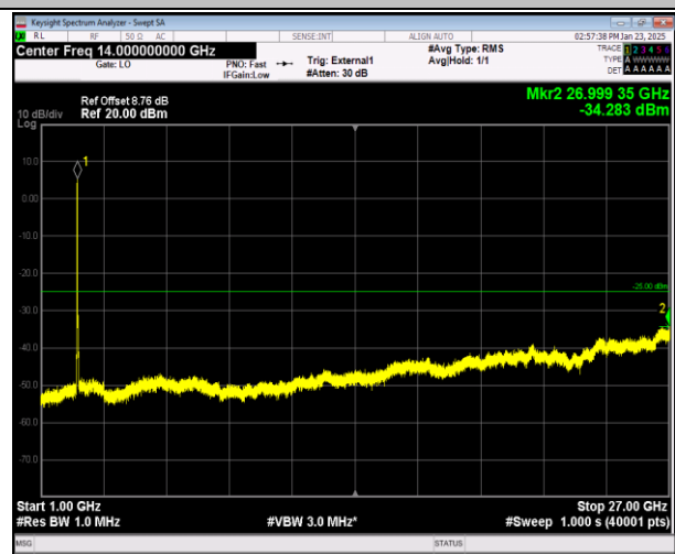
41-41-20MHz-10MHz-16QAM-16QAM-39750-39894-100RB #0-50RB#0-1000~27000MHz-PASS
