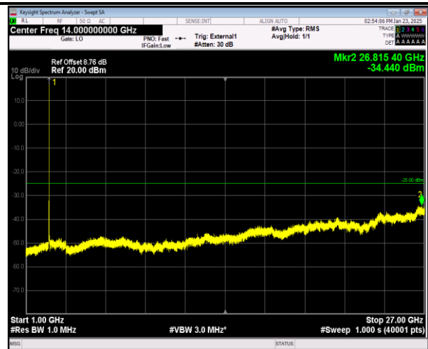
41-41-20MHz-10MHz-16QAM-16QAM-39750-39894-1RB#9 9-0RB#0-1000~27000MHz-PASS
