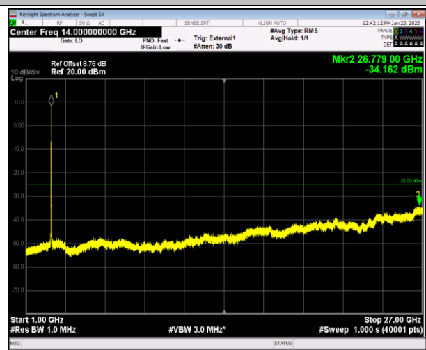
41-41-20MHz-5MHz-QPSK-QPSK-41440-41557-100RB#0- 25RB#0-1000~27000MHz-PASS
