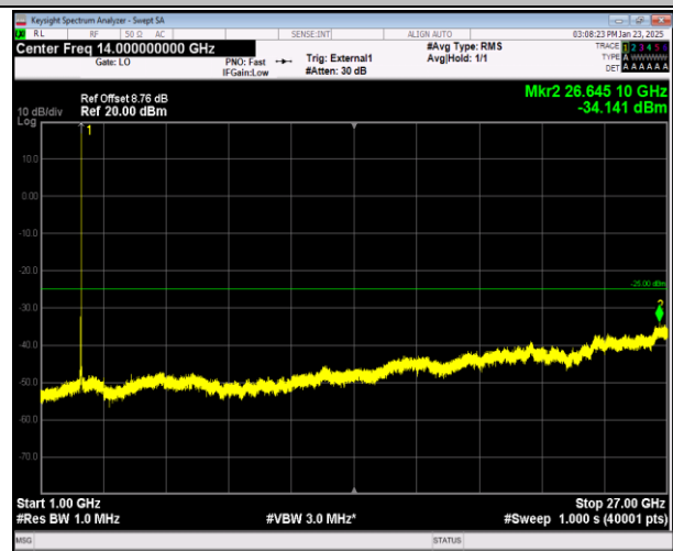
41-41-20MHz-10MHz-16QAM-16QAM-41391-41535-1RB#9 9-0RB#0-1000~27000MHz-PASS
