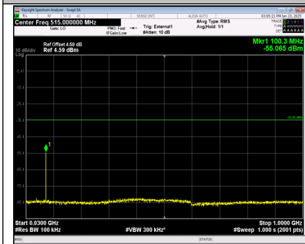
41-41-20MHz-10MHz-QPSK-QPSK-41391-41535-1RB#0 -0RB#0-30~1000MHz-PASS
