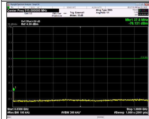
41-41-20MHz-20MHz-16QAM-16QAM-39750-39948-1RB #0-1RB#99-30~1000MHz-PASS
