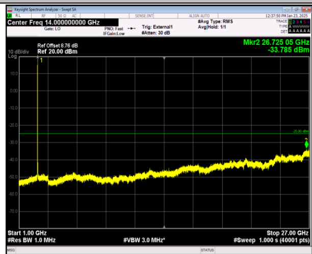
41-41-20MHz-5MHz-16QAM-16QAM-41440-41557-1RB#0- ORB#0-1000~27000MHz-PASS
