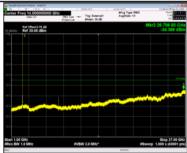
41-41-20MHz-5MHz-QPSK-QPSK-41440-41557-1RB#99-0 RB#0-1000~27000MHz-PASS
