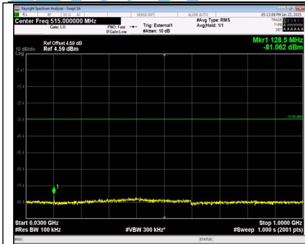
41-41-20MHz-20MHz-QPSK-QPSK-39750-39948-1RB#0 -ORB#0-30~1000MHz-PASS
