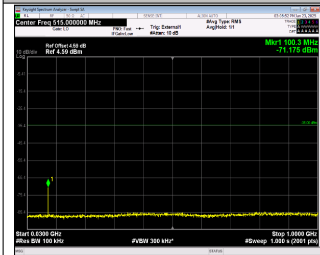
41-41-20MHz-10MHz-QPSK-QPSK-41391-41535-1RB#0 -1RB#49-30~1000MHz-PASS
