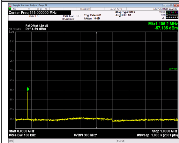
41-41-20MHz-5MHz-16QAM-16QAM-41440-41557-1RB# 0-ORB#0-30~1000MHz-PASS
