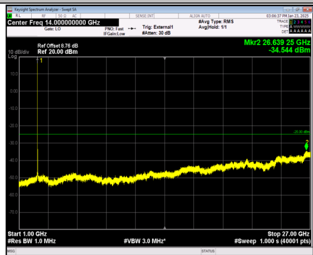
41-41-20MHz-10MHz-16QAM-16QAM-41391-41535-1RB#0 -ORB#0-1000~27000MHz-PASS
