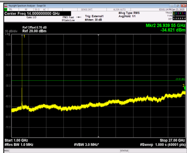
41-41-20MHz-10MHz-16QAM-16QAM-40571-40715-1RB#9 9-ORB#0-1000~27000MHz-PASS
