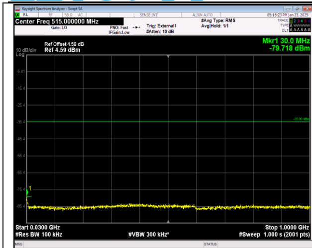
41-41-20MHz-20MHz-QPSK-QPSK-39750-39948-100RB #0-100RB#0-30~1000MHz-PASS
