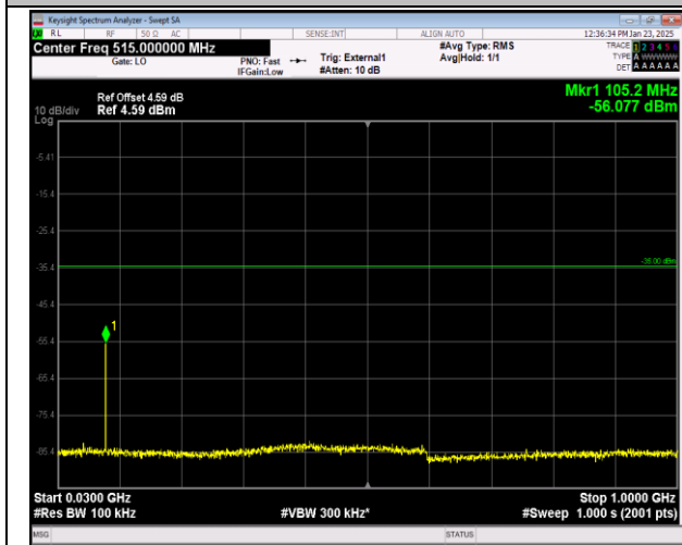
41-41-20MHz-5MHz-QPSK-QPSK-41440-41557-1RB#0-0RB#0-30~1000MHz-PASS
