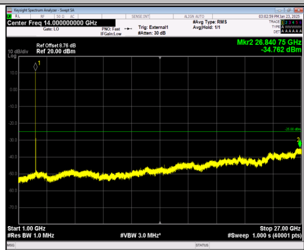
41-41-20MHz-10MHz-16QAM-16QAM-40571-40715-1RB#0 -1RB#49-1000~27000MHz-PASS
