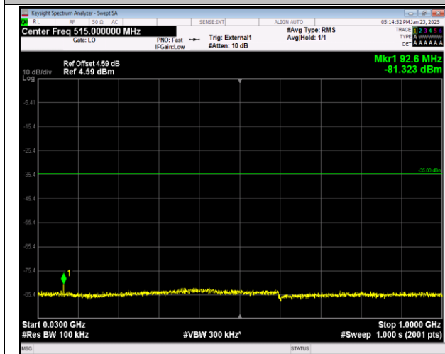
41-41-20MHz-20MHz-QPSK-QPSK-39750-39948-1RB#99 9-ORB#0-30~1000MHz-PASS
