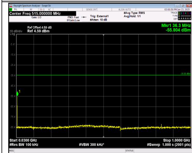
41-41-20MHz-10MHz-16QAM-16QAM-40571-40715-1RB #99-ORB#0-30~1000MHz-PASS
