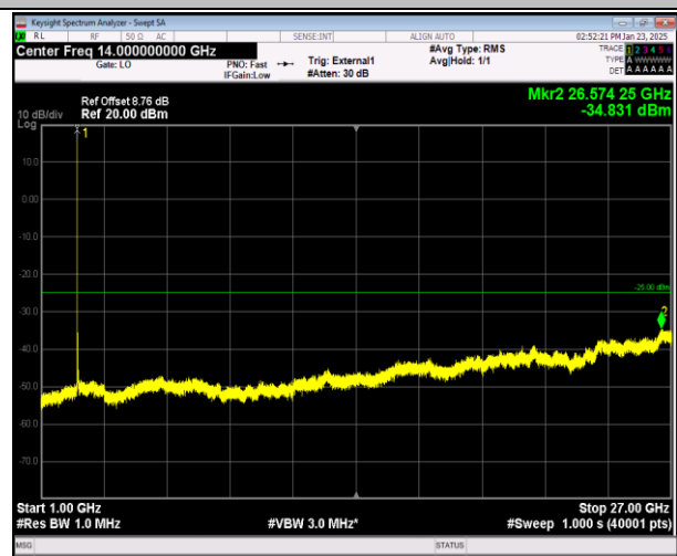
41-41-20MHz-10MHz-16QAM-16QAM-39750-39894-1RB#0 -0RB#0-1000~27000MHz-PASS
