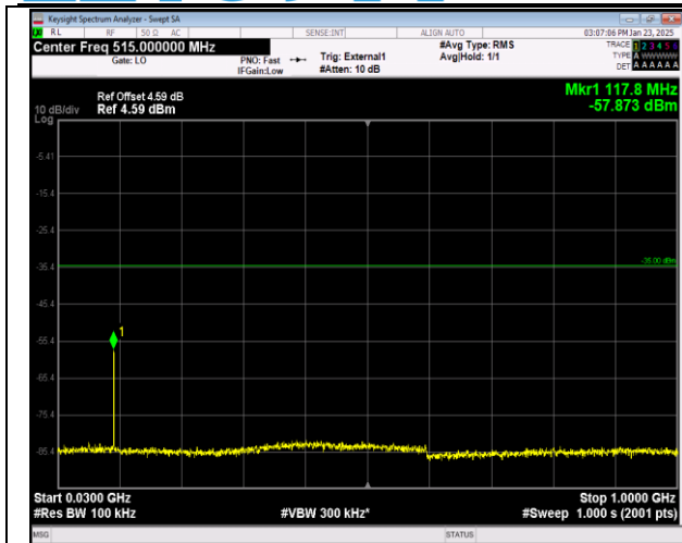
41-41-20MHz-10MHz-QPSK-QPSK-41391-41535-1RB#9 9-ORB#0-30~1000MHz-PASS
