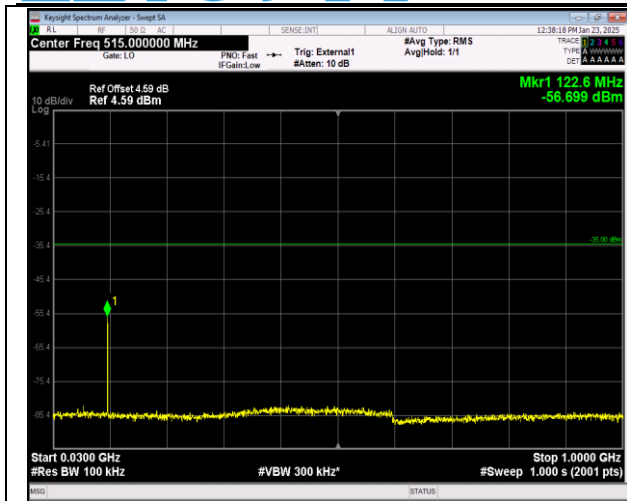
41-41-20MHz-5MHz-QPSK-QPSK-41440-41557-1RB#99 -ORB#0-30~1000MHz-PASS
