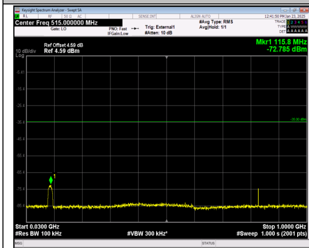
41-41-20MHz-5MHz-QPSK-QPSK-41440-41557-100RB# 0-25RB#0-30~1000MHz-PASS
