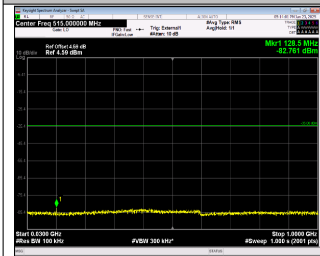
41-41-20MHz-20MHz-16QAM-16QAM-39750-39948-1RB #0-0RB#0-30~1000MHz-PASS
