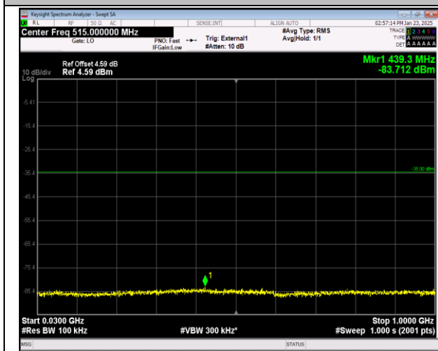
41-41-20MHz-10MHz-16QAM-16QAM-39750-39894-100RB RB#0-50RB#0-30~1000MHz-PASS
