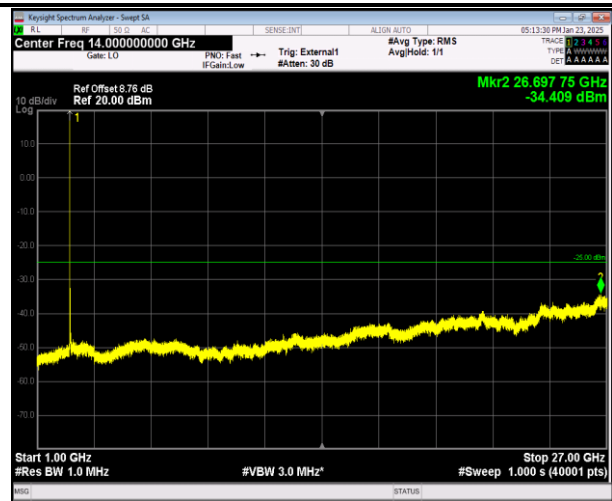
41-41-20MHz-20MHz-QPSK-QPSK-39750-39948-1RB#0-0 RB#0-1000~27000MHz-PASS
