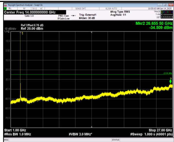
38-38-20MHz-20MHz-16QAM-16QAM-37901-38099-1RB#0 -ORB#0-1000~27000MHz-PASS
