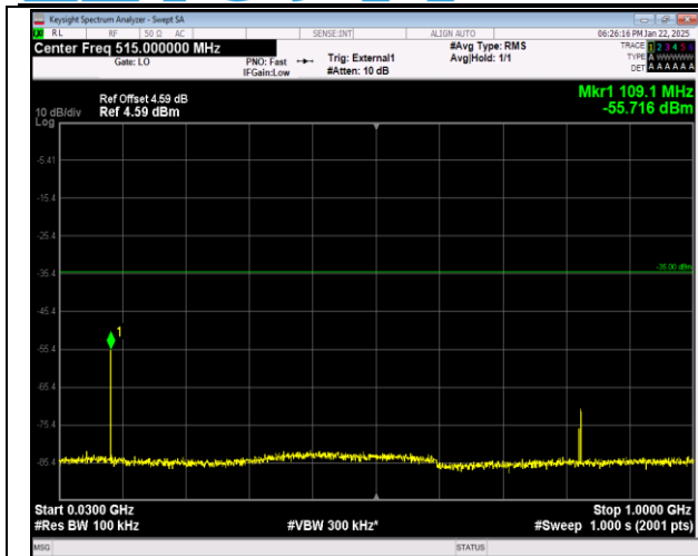
41-41-5MHz-20MHz-QPSK-QPSK-41373-41490-1RB#24 -ORB#0-30~1000MHz-PASS
