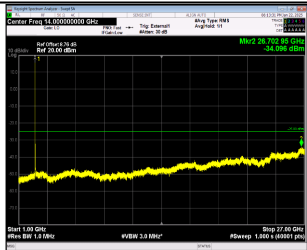
41-41-5MHz-20MHz-16QAM-16QAM-39683-39800-1RB#24 -ORB#0-1000~27000MHz-PASS
