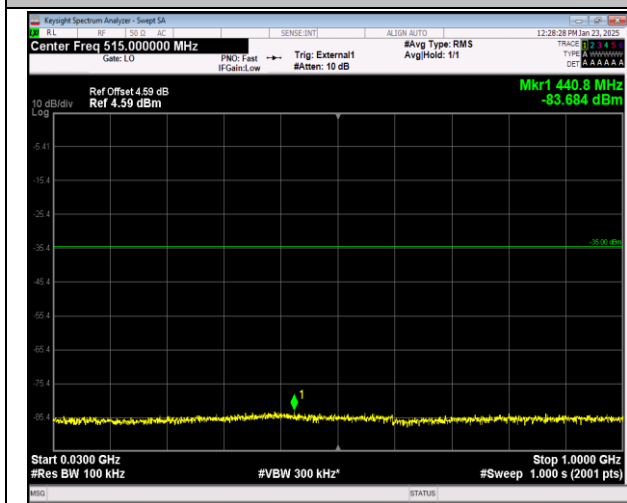
41-41-20MHz-5MHz-16QAM-16QAM-39750-39867-100RB# B#0-25RB#0-30~1000MHz-PASS
