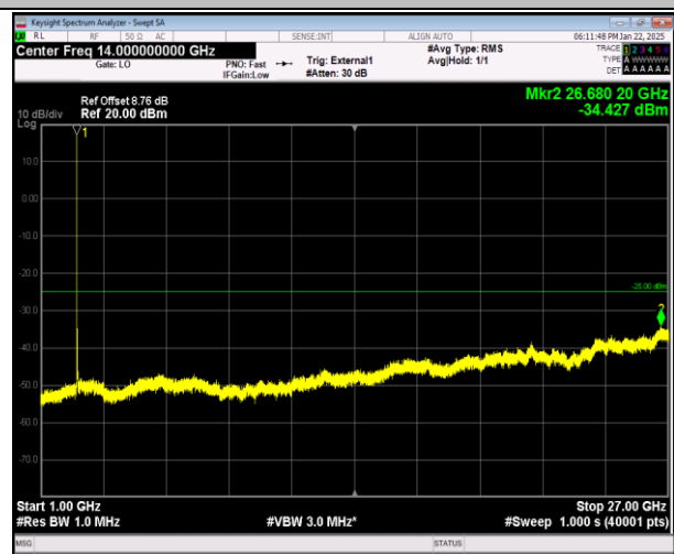
41-41-5MHz-20MHz-16QAM-16QAM-39683-39800-1RB#0- 0RB#0-1000~27000MHz-PASS
