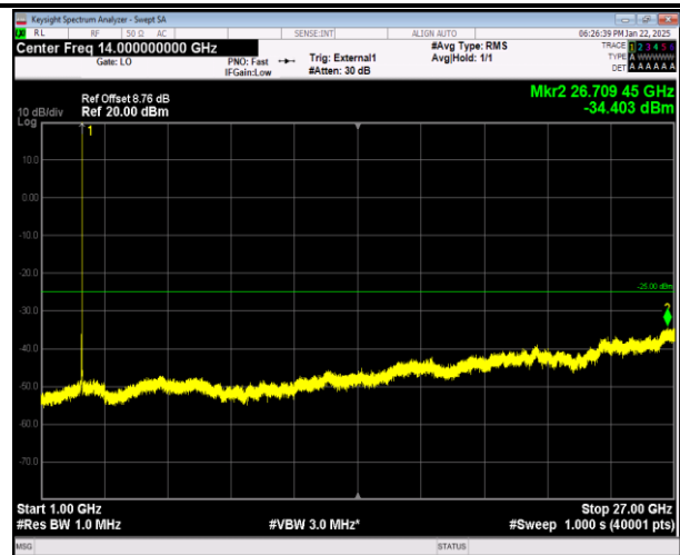
41-41-5MHz-20MHz-QPSK-QPSK-41373-41490-1RB#24-0 RB#0-1000~27000MHz-PASS
