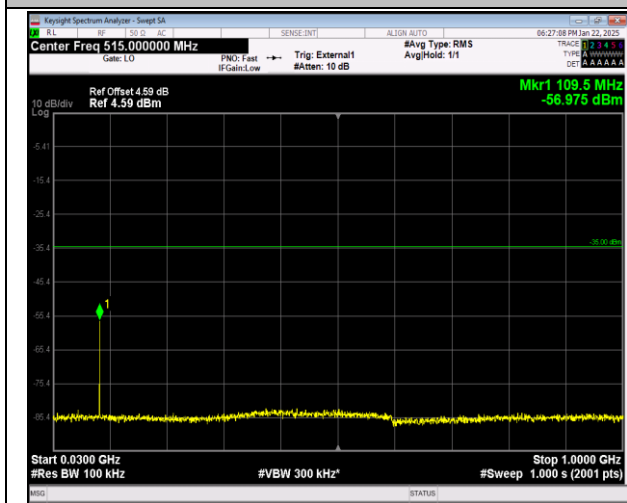
41-41-5MHz-20MHz-16QAM-16QAM-41373-41490-1RB# 24-0RB#0-30~1000MHz-PASS
