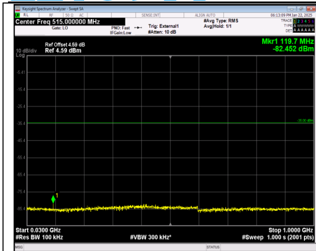
41-41-5MHz-20MHz-16QAM-16QAM-39683-39800-1RB# 24-ORB#0-30~1000MHz-PASS
