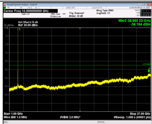
38-38-20MHz-20MHz-16QAM-16QAM-37901-38099-1RB#9 9-ORB#0-1000~27000MHz-PASS
