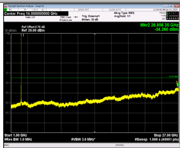
38-38-20MHz-20MHz-16QAM-16QAM-37952-38150-1RB#9 9-0RB#0-1000~27000MHz-PASS
