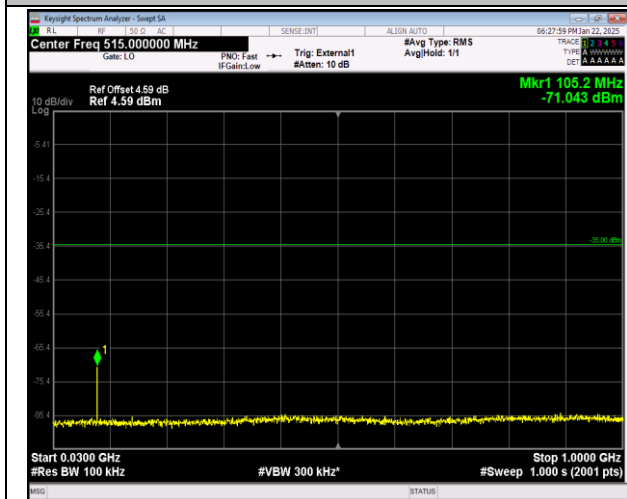
41-41-5MHz-20MHz-QPSK-QPSK-41373-41490-1RB#0-0RB#99-30~1000MHz-PASS
