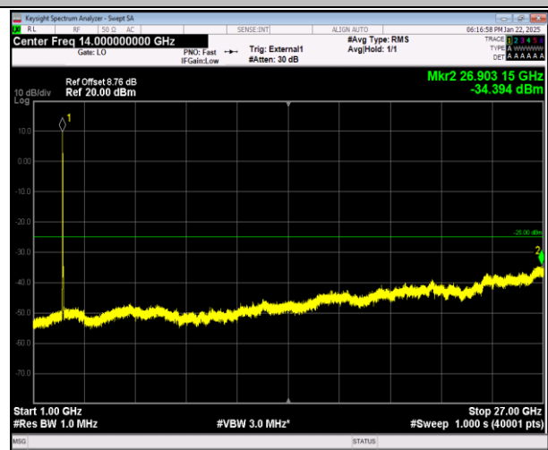
41-41-5MHz-20MHz-16QAM-16QAM-39683-39800-25RB#0 -100RB#0-1000~27000MHz-PASS
