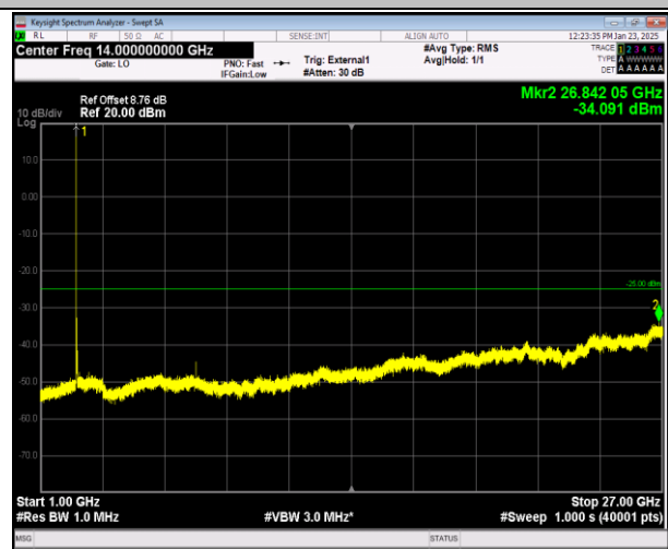
41-41-20MHz-5MHz-16QAM-16QAM-39750-39867-1RB#0- 0RB#0-1000~27000MHz-PASS
