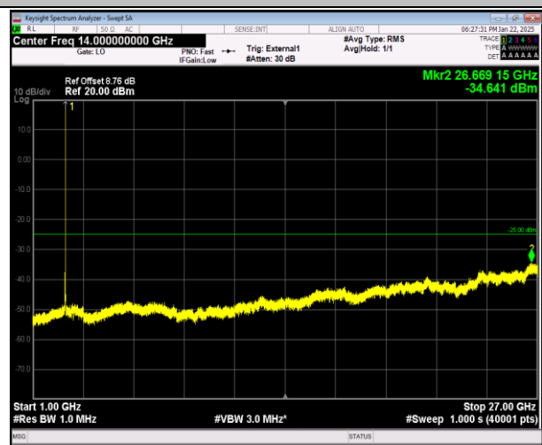
41-41-5MHz-20MHz-16QAM-16QAM-41373-41490-1RB#24 -0RB#0-1000~27000MHz-PASS
