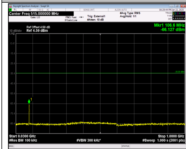
41-41-5MHz-20MHz-QPSK-QPSK-41373-41490-25RB#0 -100RB#0-30~1000MHz-PASS
