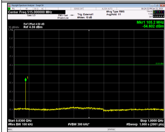
41-41-5MHz-20MHz-QPSK-QPSK-41373-41490-1RB#0-0RB#0-30~1000MHz-PASS
