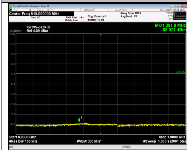
41-41-5MHz-20MHz-16QAM-16QAM-39683-39800-25RB #0-100RB#0-30~1000MHz-PASS
