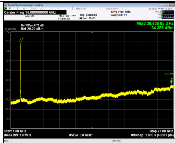
38-38-20MHz-20MHz-16QAM-16QAM-37901-38099-100RB #0-100RB#0-1000~27000MHz-PASS
