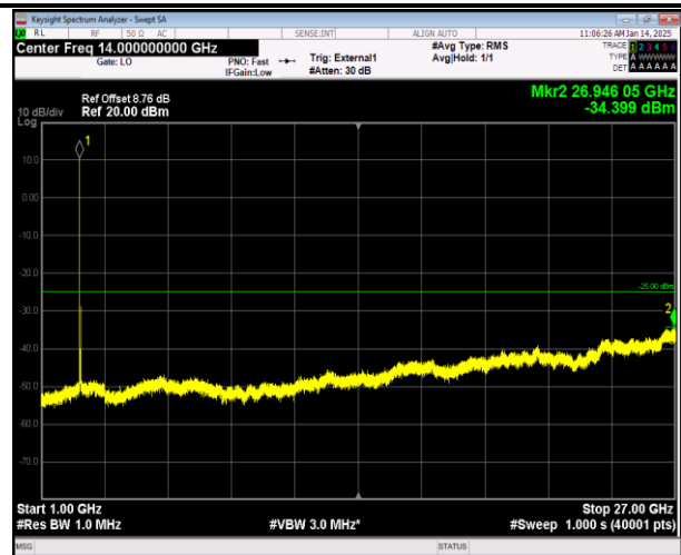
38-38-20MHz-20MHz-16QAM-16QAM-37952-38150-1RB#0 -1RB#99-1000~27000MHz-PASS
