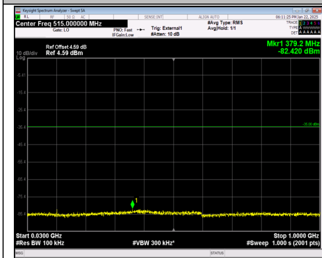
41-41-5MHz-20MHz-16QAM-16QAM-39683-39800-1RB# 0-0RB#0-30~1000MHz-PASS
