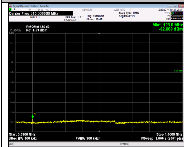
41-41-20MHz-5MHz-16QAM-16QAM-39750-39867-1RB# 0-0RB#0-30~1000MHz-PASS
