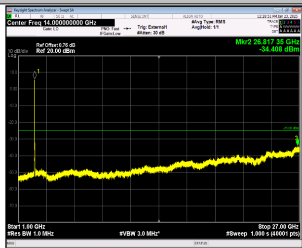
41-41-20MHz-5MHz-16QAM-16QAM-39750-39867-100RB# 0-25RB#0-1000~27000MHz-PASS
