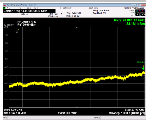
38-38-15MHz-15MHz-QPSK-QPSK-37825-37975-1RB#0-1 RB#74-1000~27000MHz-PASS
