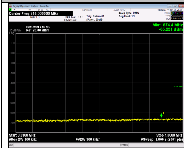
38-38-15MHz-15MHz-QPSK-QPSK-37925-38075-1RB#7 4-ORB#0-30~1000MHz-PASS
