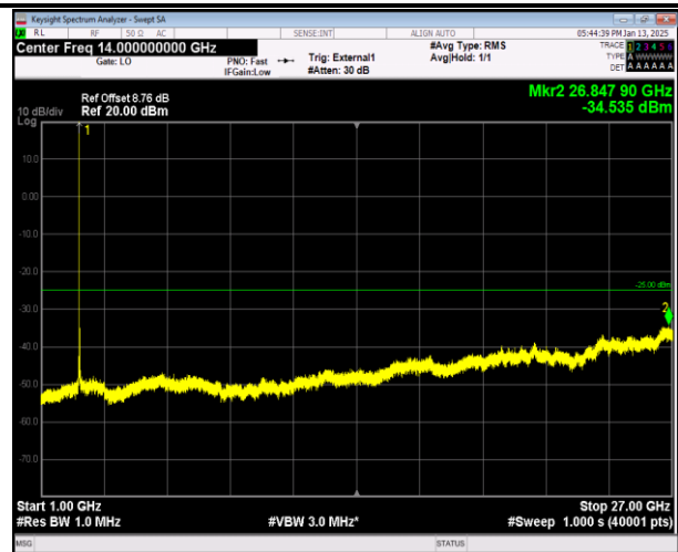
38-38-15MHz-15MHz-QPSK-QPSK-37825-37975-1RB#0-0 RB#0-1000~27000MHz-PASS
