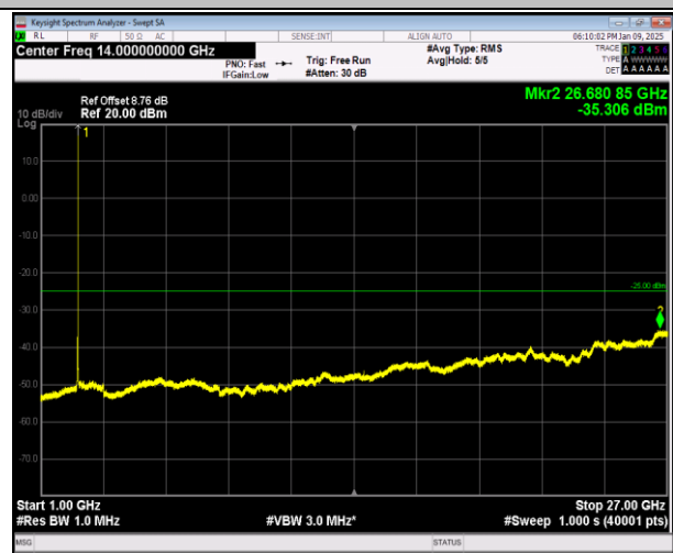
7-7-20MHz-20MHz-16QAM-16QAM-21152-21350-1RB#99- 0RB#0-1000~27000MHz-PASS
