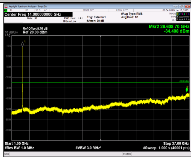
38-38-15MHz-15MHz-QPSK-QPSK-38025-38175-75RB#0- 75RB#0-1000~27000MHz-PASS
