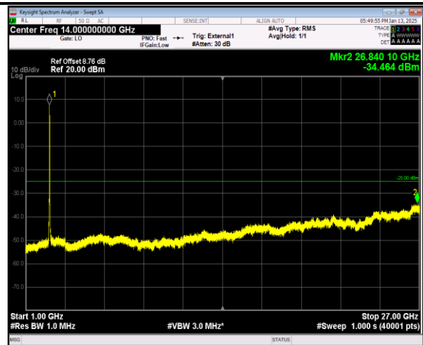
38-38-15MHz-15MHz-QPSK-QPSK-37825-37975-75RB#0- 75RB#0-1000~27000MHz-PASS
