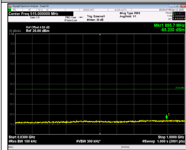
38-38-15MHz-15MHz-16QAM-16QAM-37925-38075-1RB #0-1RB#74-30~1000MHz-PASS
