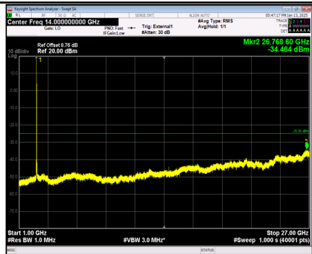
38-38-15MHz-15MHz-16QAM-16QAM-37825-37975-1RB#7 4-0RB#0-1000~27000MHz-PASS
