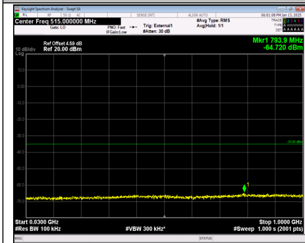
38-38-15MHz-15MHz-16QAM-16QAM-38025-38175-1RB #74-0RB#0-30~1000MHz-PASS
