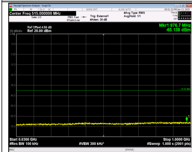
38-38-15MHz-15MHz-QPSK-QPSK-37925-38075-1RB#0 -0RB#0-30~1000MHz-PASS
