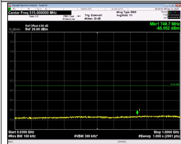
38-38-15MHz-15MHz-16QAM-16QAM-37925-38075-1RB #74-ORB#0-30~1000MHz-PASS
