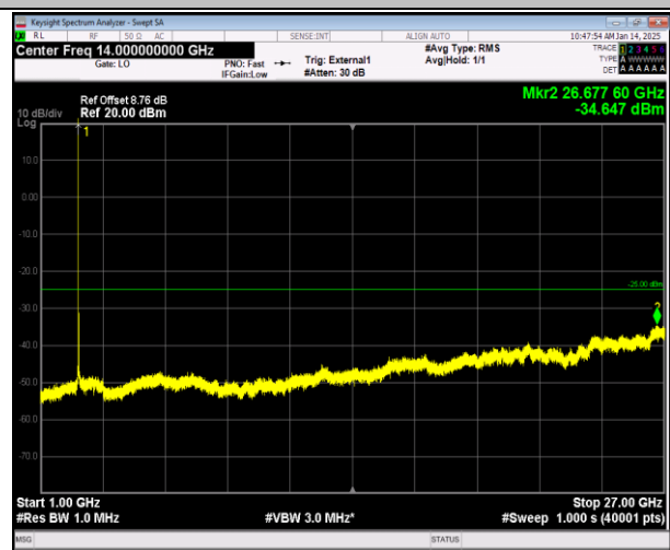
38-38-20MHz-20MHz-16QAM-16QAM-37850-38048-1RB#0 -0RB#0-1000~27000MHz-PASS
