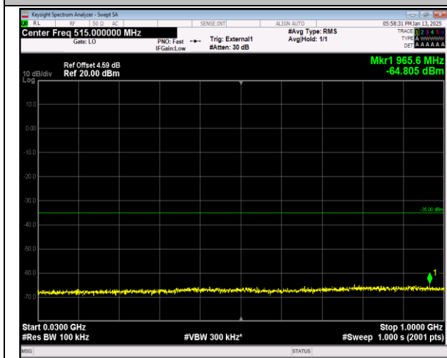
38-38-15MHz-15MHz-QPSK-QPSK-38025-38175-1RB#0 -0RB#0-30~1000MHz-PASS
