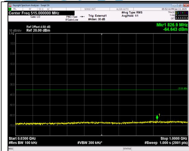
38-38-15MHz-15MHz-16QAM-16QAM-37925-38075-1RB #0-ORB#0-30~1000MHz-PASS
