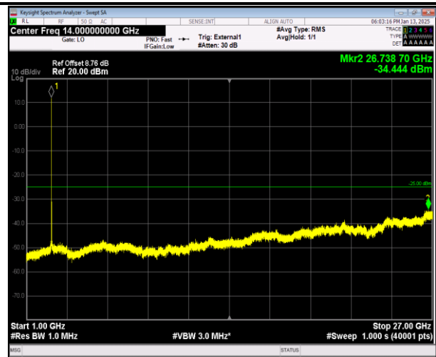
38-38-15MHz-15MHz-16QAM-16QAM-38025-38175-1RB#0 -1RB#74-1000~27000MHz-PASS
