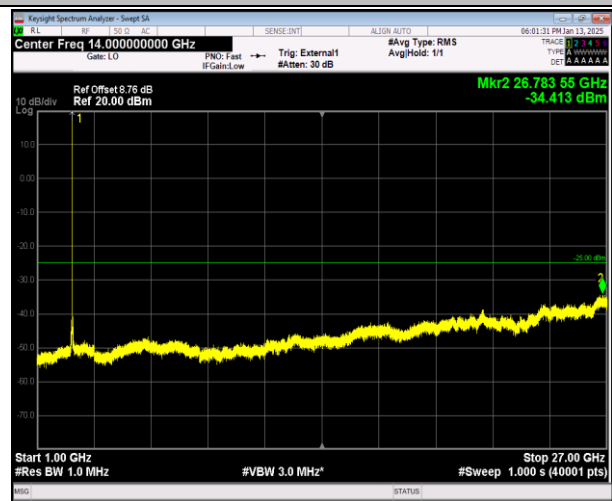
38-38-15MHz-15MHz-16QAM-16QAM-38025-38175-1RB#7 4-0RB#0-1000~27000MHz-PASS
