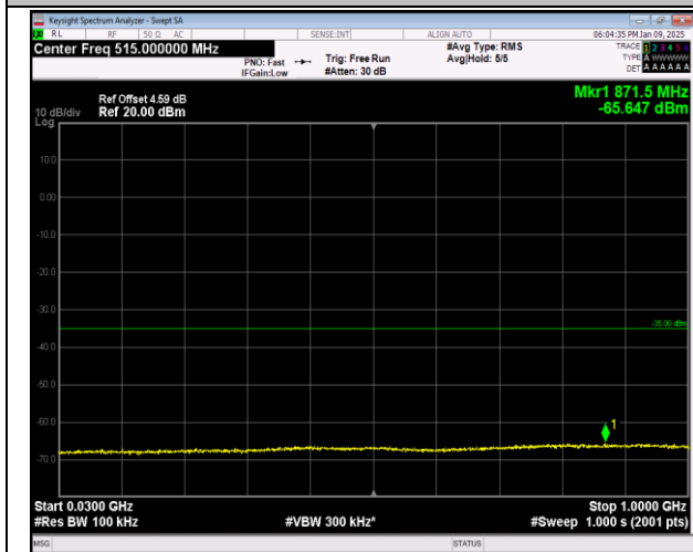
7-7-20MHz-20MHz-16QAM-16QAM-21001-21199-1RB#9 9-ORB#0-30~1000MHz-PASS
