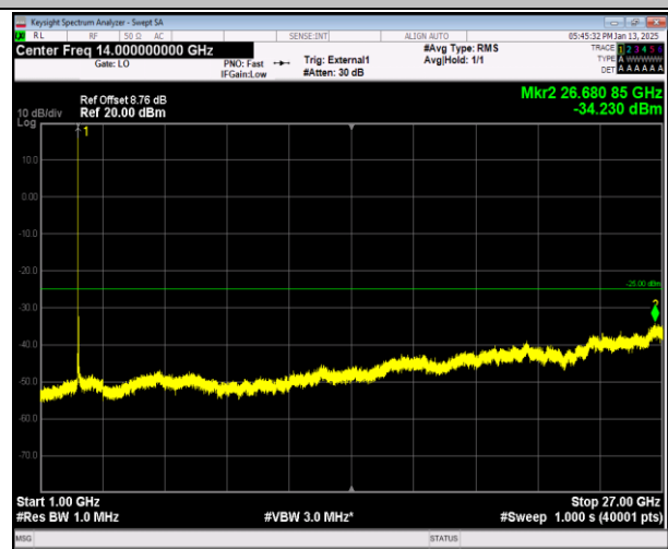
38-38-15MHz-15MHz-16QAM-16QAM-37825-37975-1RB#0 -0RB#0-1000~27000MHz-PASS
