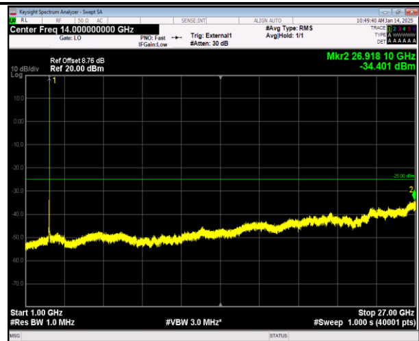
38-38-20MHz-20MHz-16QAM-16QAM-37850-38048-1RB#9 9-0RB#0-1000~27000MHz-PASS
