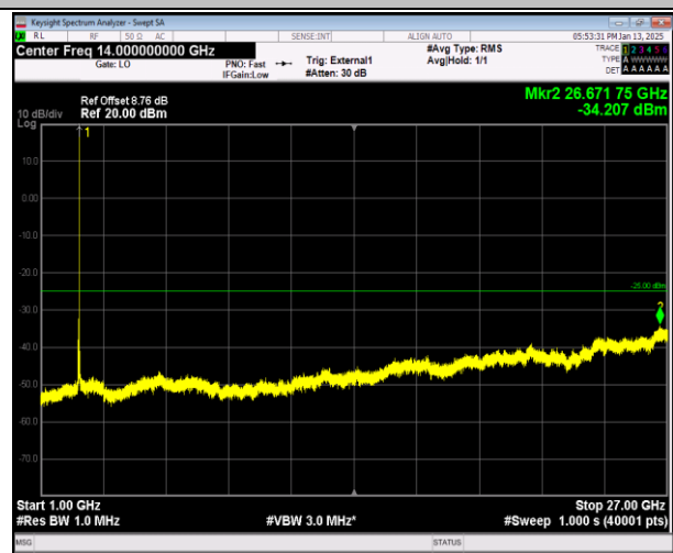
38-38-15MHz-15MHz-QPSK-QPSK-37925-38075-1RB#74- ORB#0-1000~27000MHz-PASS
