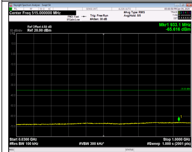
7-7-20MHz-10MHz-QPSK-QPSK-20850-20994-1RB#99-99 ORB#0-30~1000MHz-PASS
