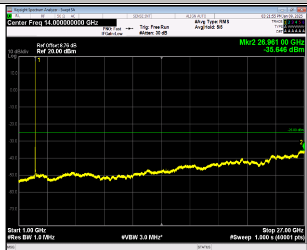
7-7-10MHz-20MHz-QPSK-QPSK-20805-20949-1RB#49-OR
