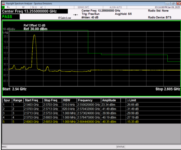
7-7-10MHz-20MHz-QPSK@QPSK-QPSK@QPSK-21206-21350-1RB#49@50RB#0-0RB#0@100RB#0-PASS
