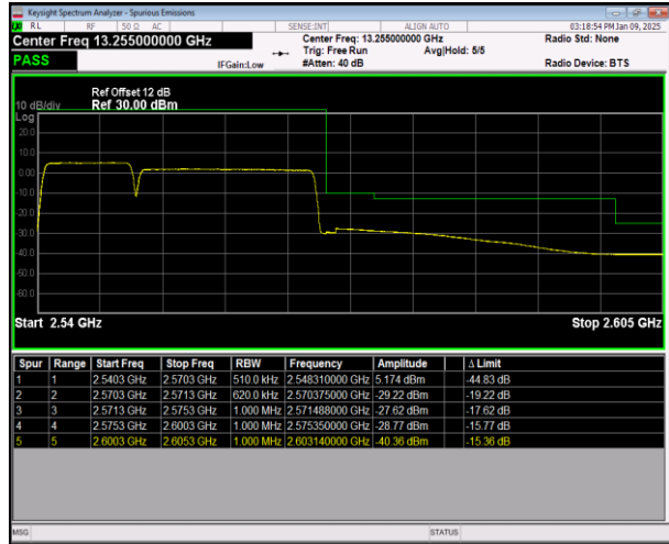
7-7-10MHz-20MHz-QPSK@QPSK-QPSK@QPSK-21206-21350-50RB#0@50RB#0-100RB#0@100RB#0-PASS
