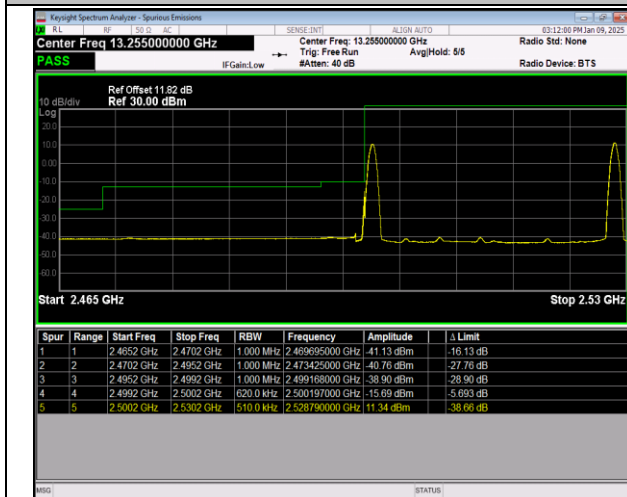
7-7-10MHz-20MHz-QPSK@QPSK-QPSK@QPSK-20805-20949-1RB#0@50RB#0-1RB#99@100RB#0-PASS
