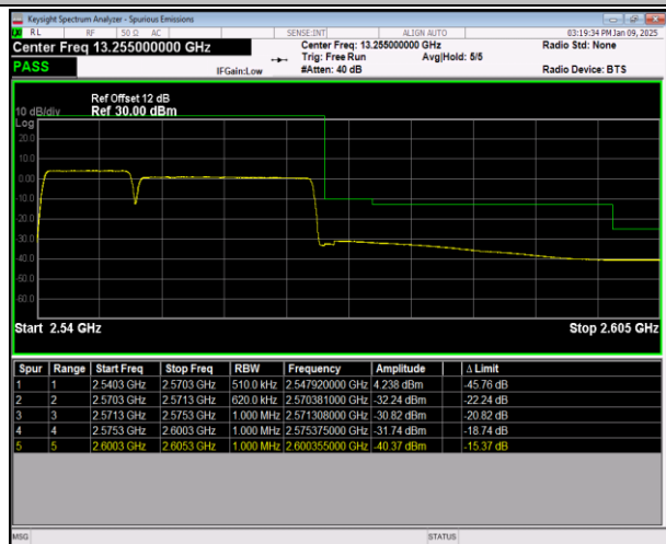
7-7-10MHz-20MHz-16QAM@16QAM-16QAM@16QAM-21206-21350-50RB#0@50RB#0-100RB#0@100RB#0-PASS
