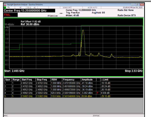
7-7-10MHz-20MHz-16QAM@16QAM-16QAM@16QAM-20
