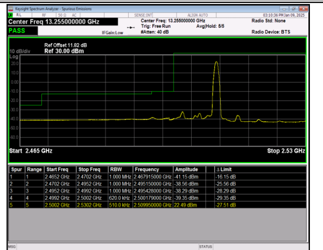
7-7-10MHz-20MHz-QPSK@QPSK-QPSK@QPSK-20805-20949-1RB#49@50RB#0-0RB#0@100RB#0-PASS
