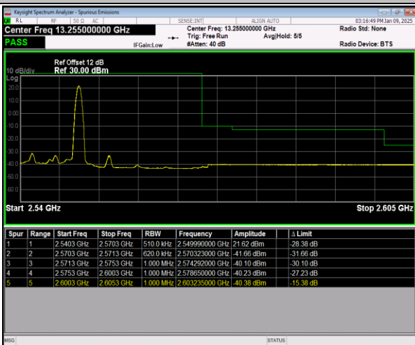
7-7-10MHz-20MHz-16QAM@16QAM-16QAM@16QAM-21206-21350-1RB#49@50RB#0-0RB#0@100RB#0-PASS
