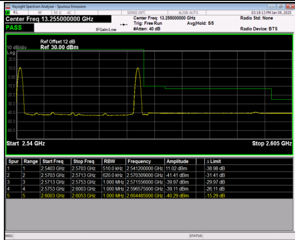
7-7-10MHz-20MHz-16QAM@16QAM-16QAM@16QAM-21206-21350-1RB#0@50RB#0-1RB#99@100RB#0-PASS
