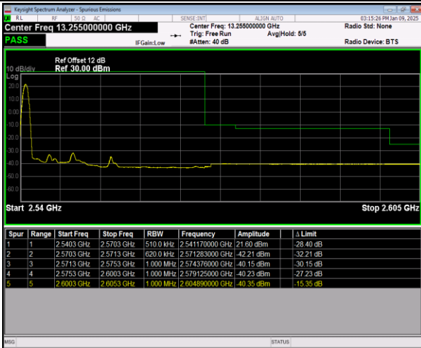
7-7-10MHz-20MHz-16QAM@16QAM-16QAM@16QAM-21206-21350-1RB#0@50RB#0-0RB#0@100RB#0-PASS
