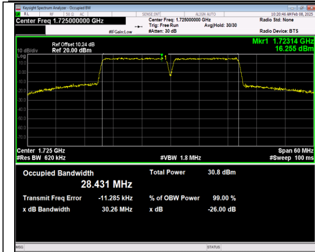
66-66-15MHz-15MHz-QPSK-QPSK-132047-132197-75R B#0-75RB#0-PASS
