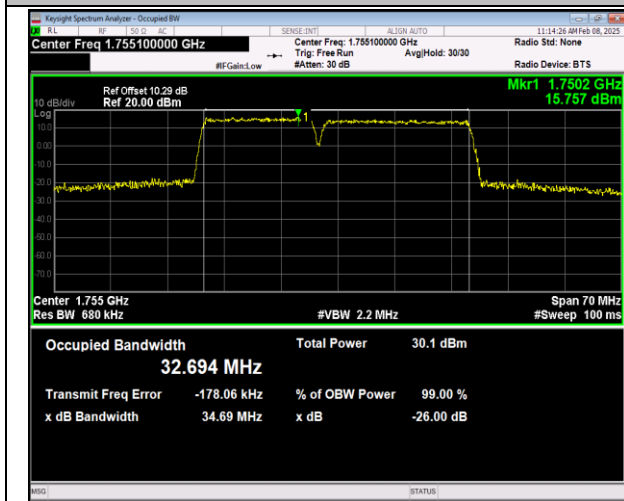
66-66-15MHz-20MHz-QPSK-QPSK-132325-132496-75R B#0-100RB#0-PASS
