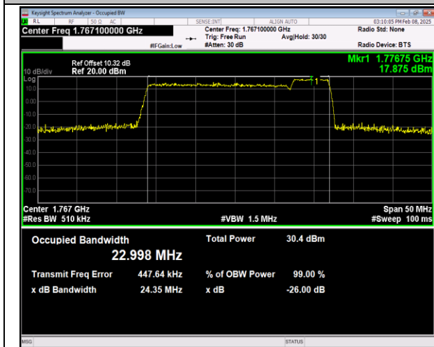
66-66-20MHz-5MHz-QPSK-QPSK-132522-132639-100R B#0-25RB#0-PASS
