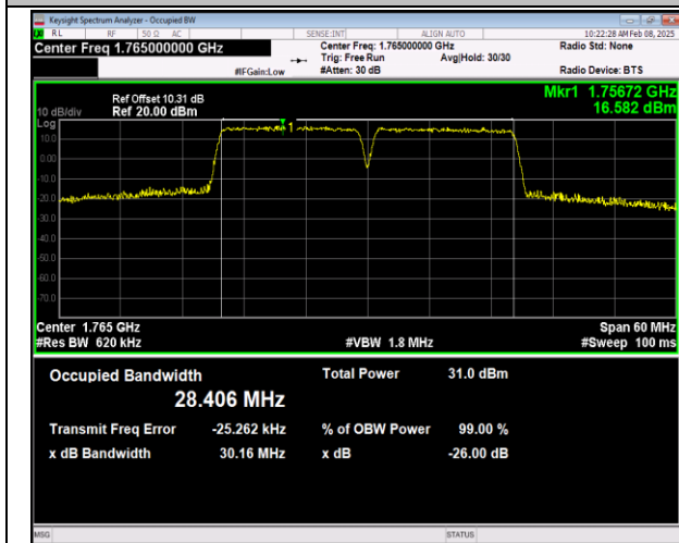
66-66-15MHz-15MHz-QPSK-QPSK-132447-132597-75R B#0-75RB#0-PASS
