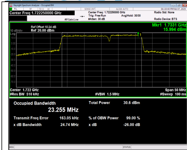
66-66-15MHz-10MHz-QPSK-QPSK-132047-132167-75R B#0-50RB#0-PASS
