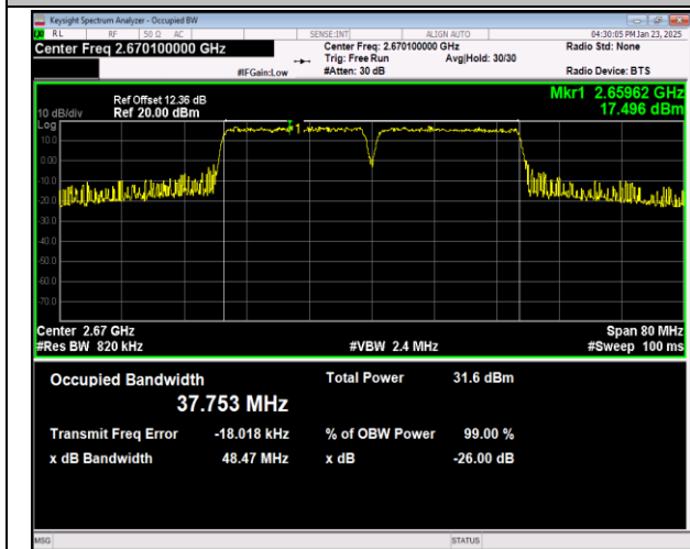
41-41-20MHz-20MHz-QPSK-QPSK-41292-41490-100RB #0-100RB#0-PASS
