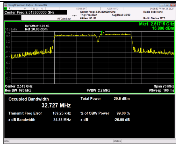
41-41-20MHz-15MHz-16QAM-16QAM-39750-39921-100R B#0-75RB#0-PASS
