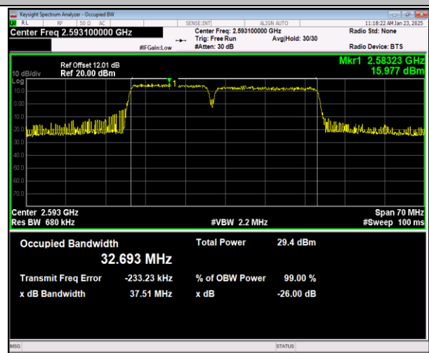
41-41-15MHz-20MHz-16QAM-16QAM-40523-40694-75RB #0-100RB#0-PASS
