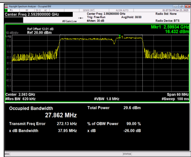
41-41-20MHz-10MHz-16QAM-16QAM-40571-40715-100R B#0-50RB#0-PASS
