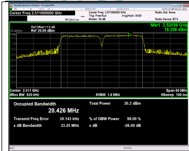
41-41-15MHz-15MHz-QPSK-QPSK-39725-39875-75RB# 0-75RB#0-PASS
