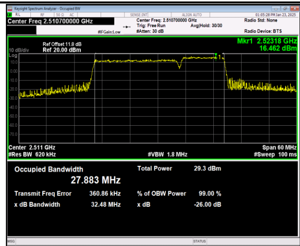
41-41-20MHz-10MHz-16QAM-16QAM-39750-39894-100R B#0-50RB#0-PASS
