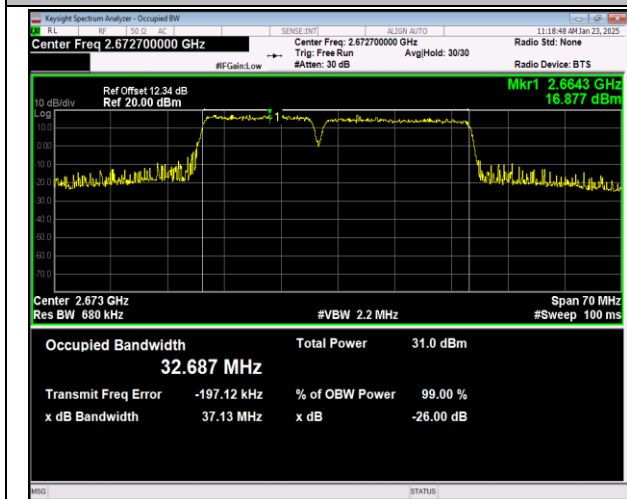
41-41-15MHz-20MHz-QPSK-QPSK-41319-41490-75RB# 0-100RB#0-PASS
