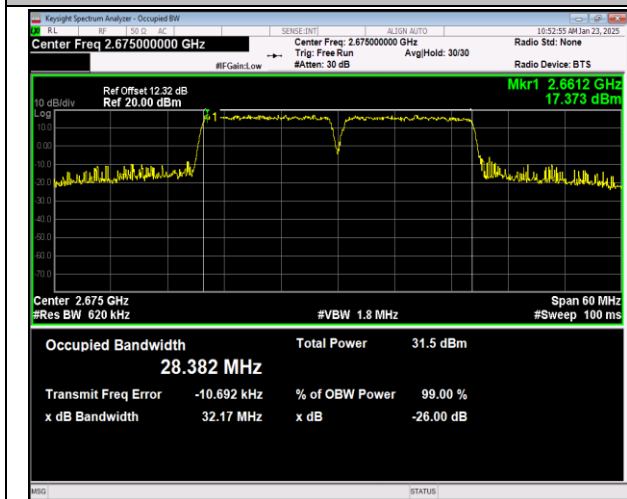
41-41-15MHz-15MHz-QPSK-QPSK-41365-41515-75RB# 0-75RB#0-PASS
