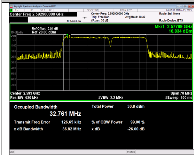
41-41-20MHz-15MHz-QPSK-QPSK-40546-40717-100RB #0-75RB#0-PASS
