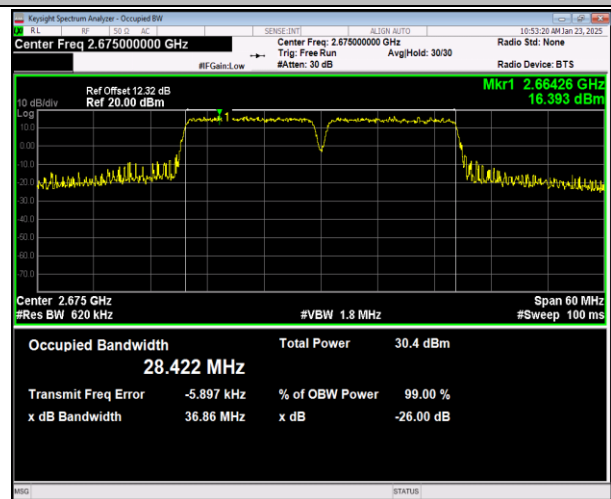
41-41-15MHz-15MHz-16QAM-16QAM-41365-41515-75RB #0-75RB#0-PASS
