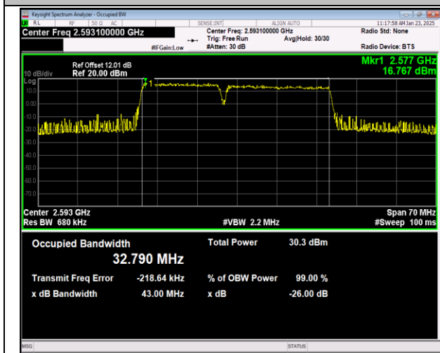
41-41-15MHz-20MHz-QPSK-QPSK-40523-40694-75RB# 0-100RB#0-PASS
