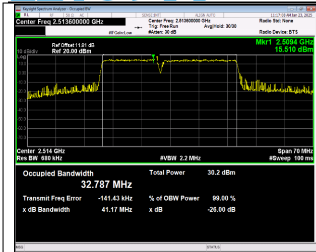
41-41-15MHz-20MHz-QPSK-QPSK-39728-39899-75RB# 0-100RB#0-PASS
