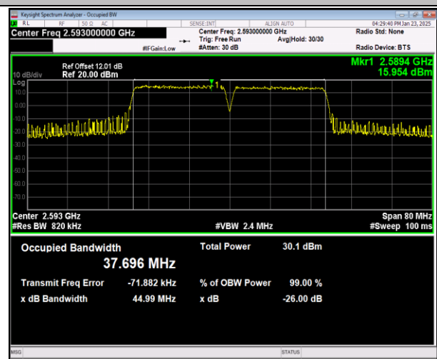
41-41-20MHz-20MHz-16QAM-16QAM-40521-40719-100RB B#0-100RB#0-PASS
