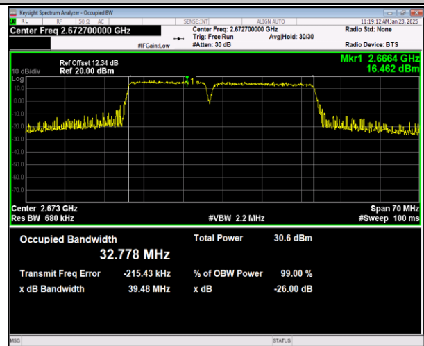
41-41-15MHz-20MHz-16QAM-16QAM-41319-41490-75RB #0-100RB#0-PASS
