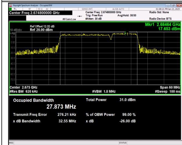
41-41-20MHz-10MHz-QPSK-QPSK-41391-41535-100RB #0-50RB#0-PASS
