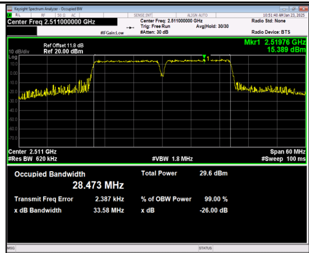
41-41-15MHz-15MHz-16QAM-16QAM-39725-39875-75RB #0-75RB#0-PASS
