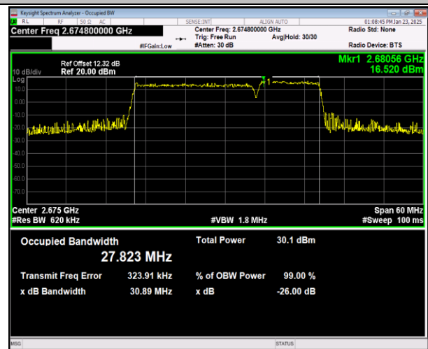
41-41-20MHz-10MHz-16QAM-16QAM-41391-41535-100R B#0-50RB#0-PASS
