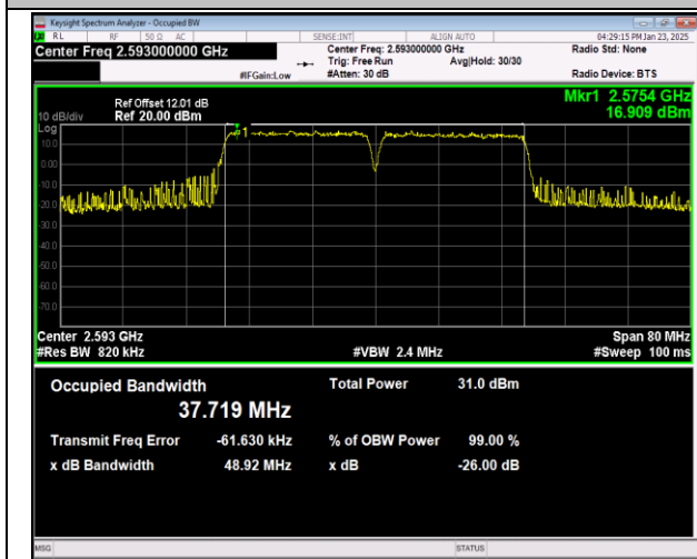
41-41-20MHz-20MHz-QPSK-QPSK-40521-40719-100RB #0-100RB#0-PASS
