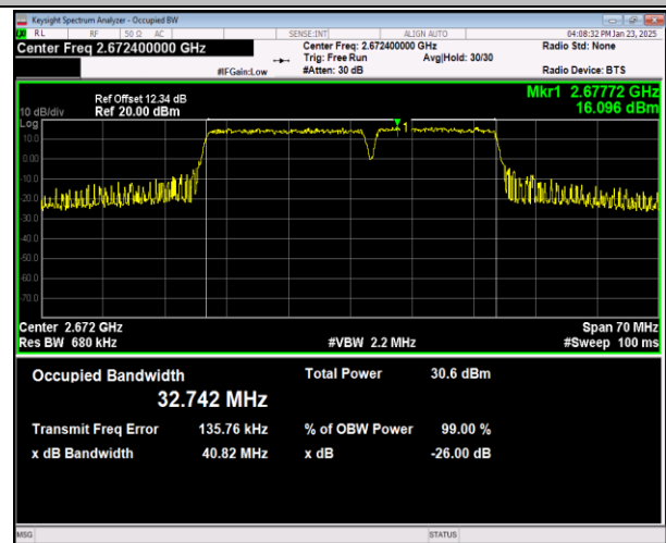
41-41-20MHz-15MHz-16QAM-16QAM-41341-41512-100R B#0-75RB#0-PASS
