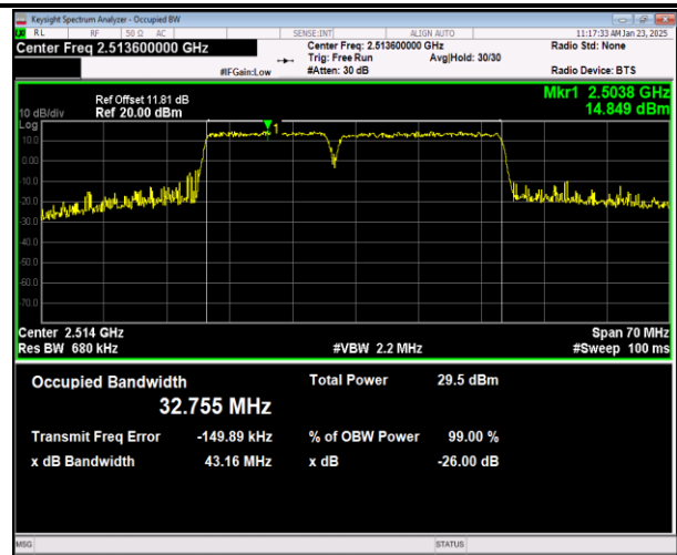
41-41-15MHz-20MHz-16QAM-16QAM-39728-39899-75RB #0-100RB#0-PASS
