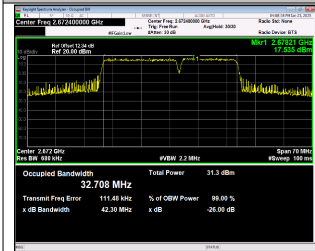
41-41-20MHz-15MHz-QPSK-QPSK-41341-41512-100RB #0-75RB#0-PASS
