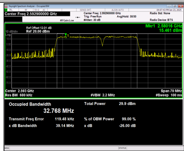
41-41-20MHz-15MHz-16QAM-16QAM-40546-40717-100R B#0-75RB#0-PASS
