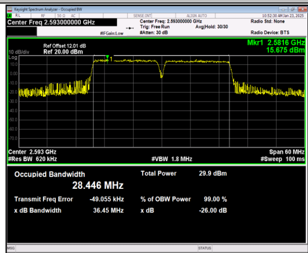
41-41-15MHz-15MHz-16QAM-16QAM-40545-40695-75RB #0-75RB#0-PASS
