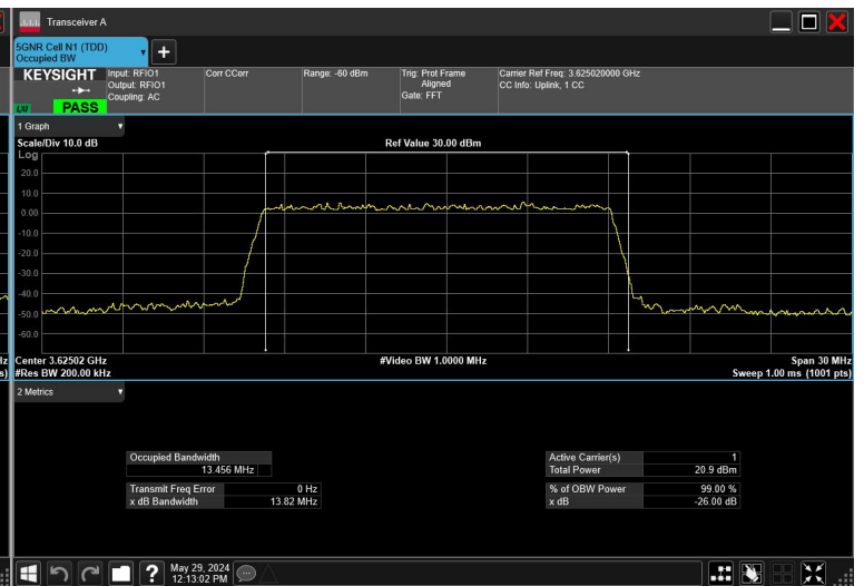
15MHz_30kHz_3625MHz_DFT-s-OFDM 64QAM_RB36@0
